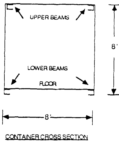
(a) TYPICAL OF CONTAINERS OBSERVED IN ON-SITE INSPECTION
