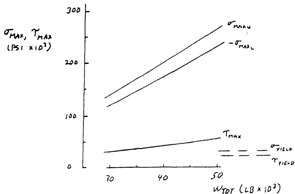
Figure 26. "Lower Beam Only", Maximum Bending Moment
