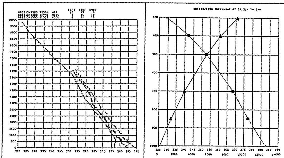
Fig. 11. Case 3 temperature profiles. 1200 UTC 13 December 1988. Fig. 11a shows HAT (triangle) rawinsonde and NC06 (square), NC08 (circle) dropwinsondes as linear height (m) and temperature (K) plot, Fig. 11b shows spectral gridded profile as linear pressure versus temperature (square) and linear pressure versus height (triangle) plot.
