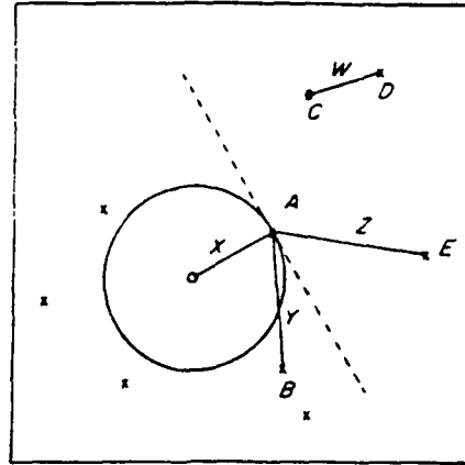
Key ● A randomly chosen plant x Other plants ○ A randomly chosen point A, B, C, D, E. Plant locations W, X, Y, Z. Nearest-neighbour distances
