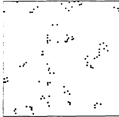
Figure 2-7: An Example of a Poisson Cluster Process
