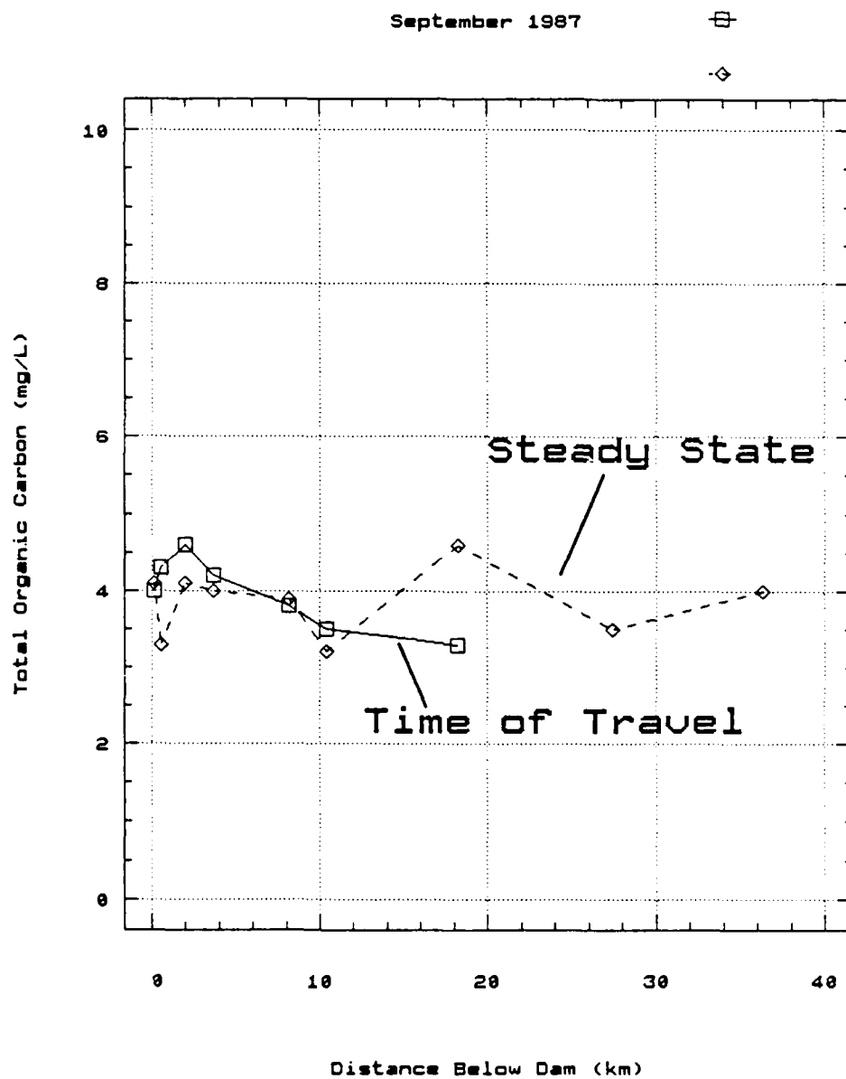
Figure C28. Lake Greeson tailwater, total organic carbon versus distance below dam for time-of-travel and steady-state sampling, 9/12/87-9/14/87
