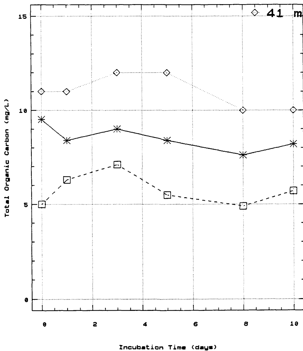
Figure C48. Lake Greeson, August 25, 1987, 10-day BOD, mean total organic carbon
