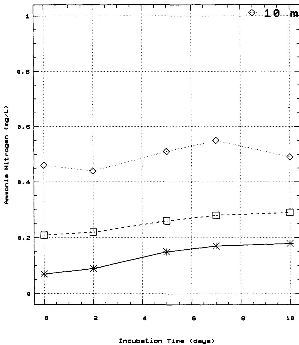
Figure 83. Lake Nimrod, July 6, 1988, 10-day BOD, mean ammonia nitrogen
