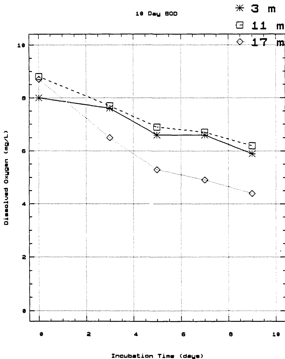
Figure C105. Rough River Lake, August 11, 1988, 10-day BOD, mean DO
