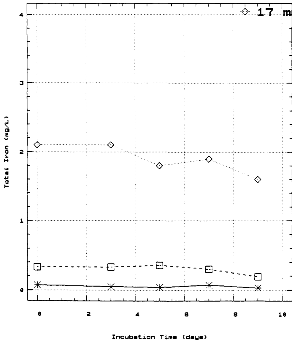
Figure C109. Rough River Lake, August 11, 1988, 10-day BOD, mean total iron
