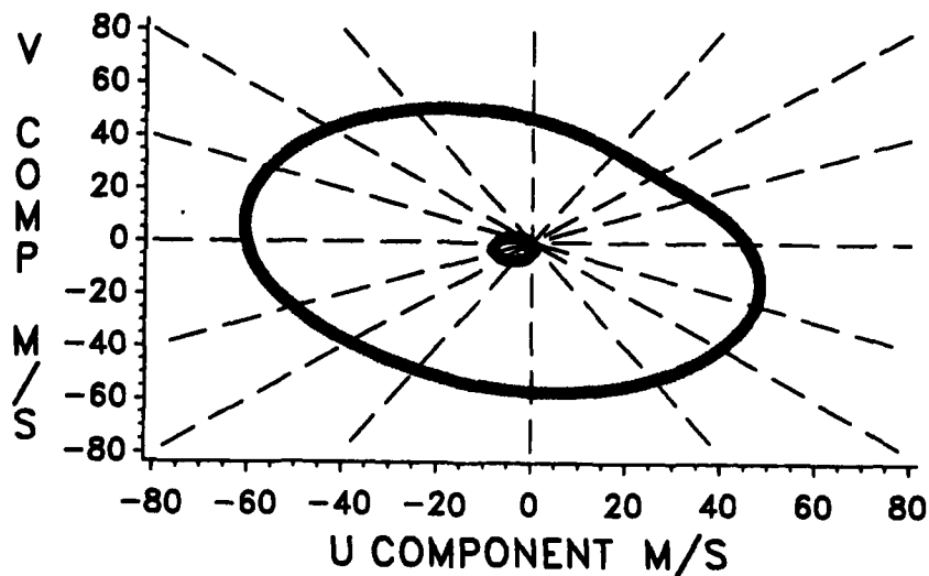
Figure E-22. Wind Interpercentile Range and Mean, January, 50 KM.
