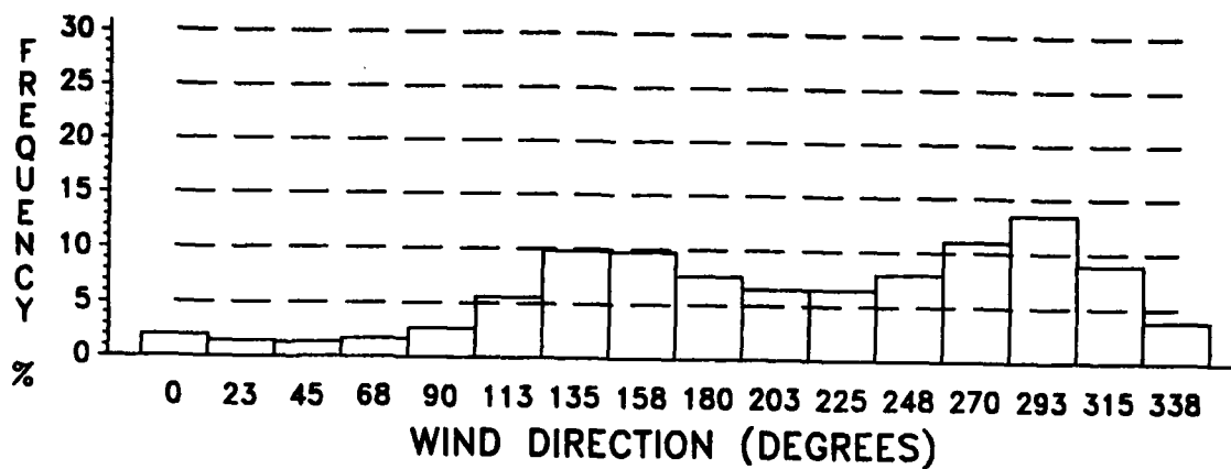
Figure E-7. Wind Direction Frequency, January, 60 KM.
