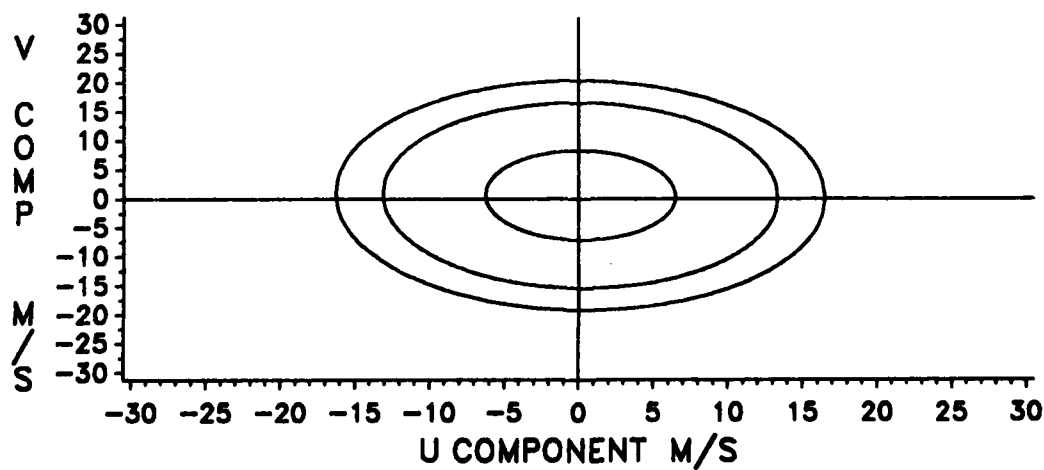
Figure E-41. Wind Probability Ellipses, July, 4 KM.
