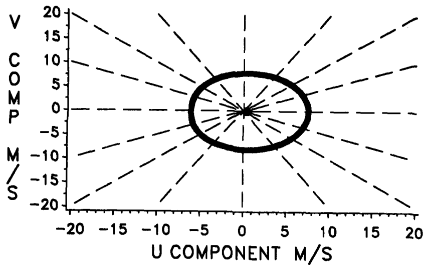
Figure E-26. Wind Interpercentile Range and Mean, July, 12 KM.
