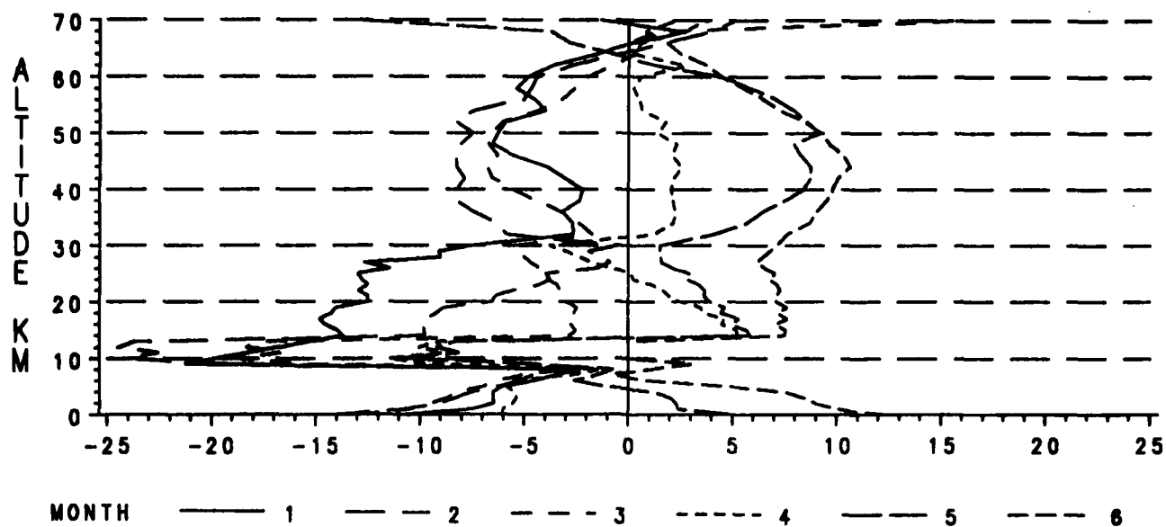
Figure F-15. Delta Temperature (K), January-June.
