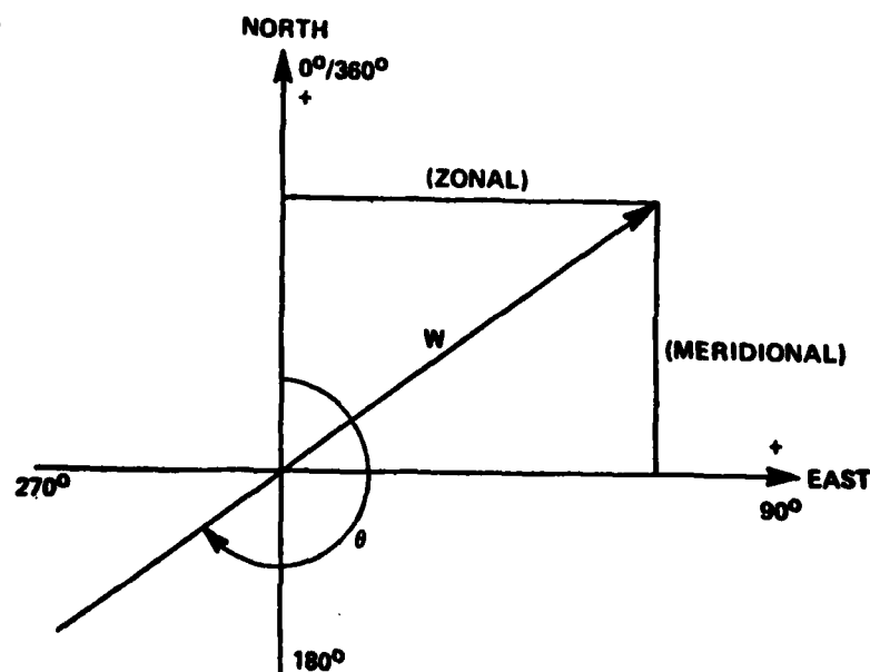
Figure 2-1. The Standard Meteorological Coordinate System.
