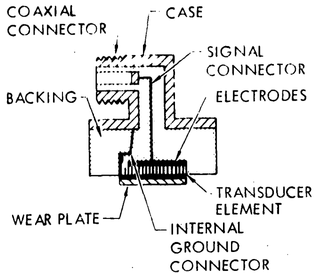
Figure 10. Contact search unit
