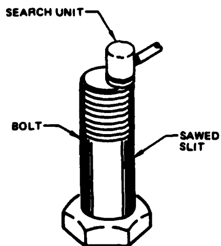
Figure 15. Reference standard for inspection of a bolt
