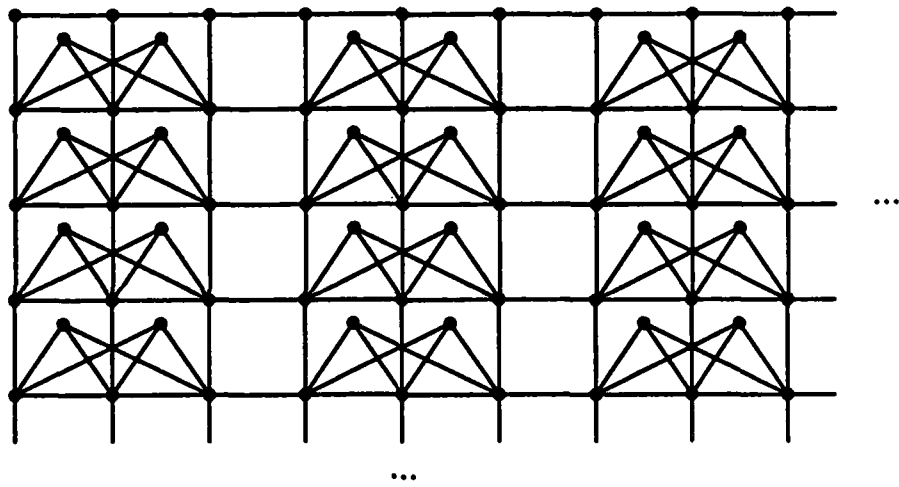
Figure 9: A graph that may require O(n) decomposition iterations.
