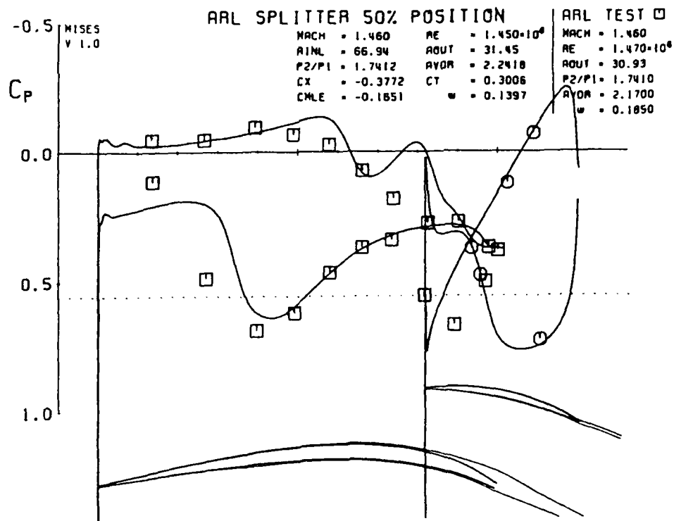
Figure 4.24: Surface pressures for ARL blades, p_2/p_1 = 1.741 , 109% AVDR.
