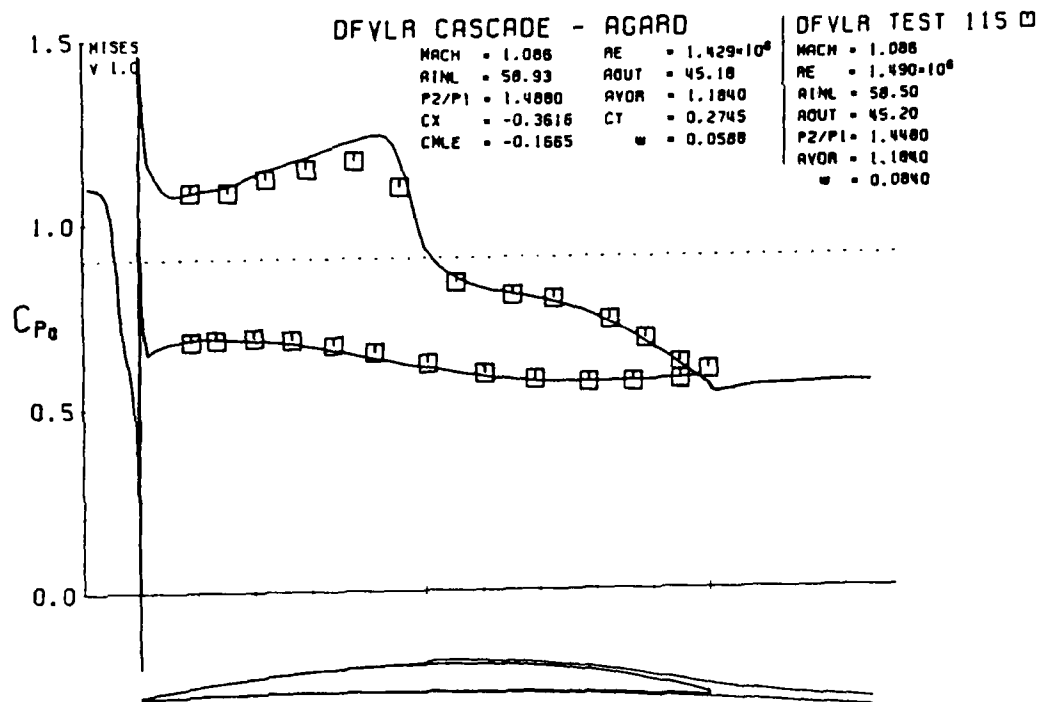
Figure 4.12: DFVLR blade: M = 1.086 , \beta_1 = 58.5^\circ , AVDR = 1.184
