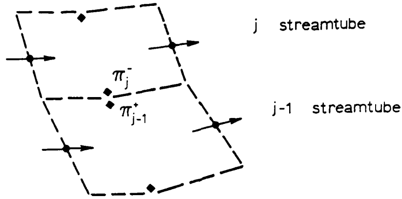
Figure A.5: Pressures on neighboring streamtubes
