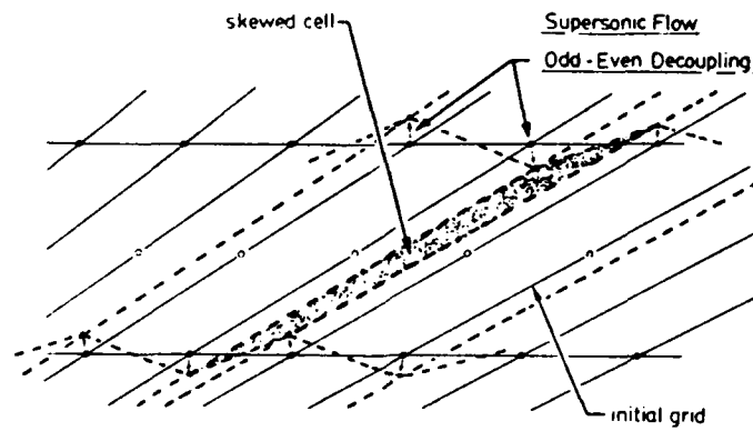
Figure 3.11: Supersonic odd-even instability for skewed grids.
