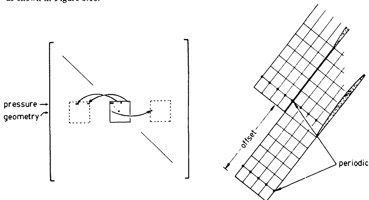
Figure 3.16: Arrangement of off-diagonal periodicity terms for offset grid.
