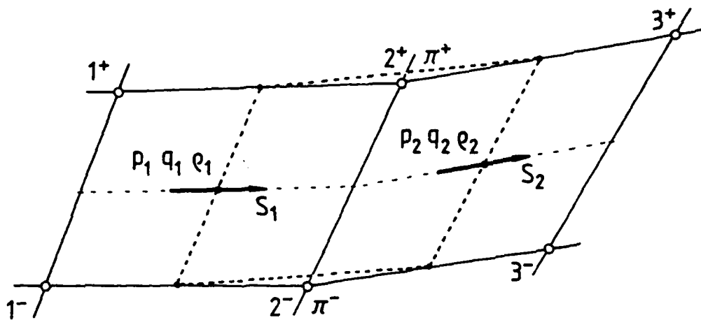
Figure A.1: Conservation cell on nodal grid
