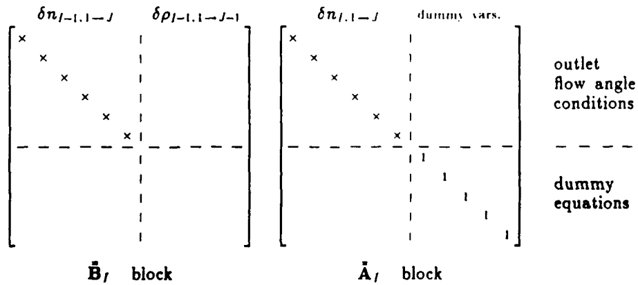
Figure D.6: Structure of exit blocks.
