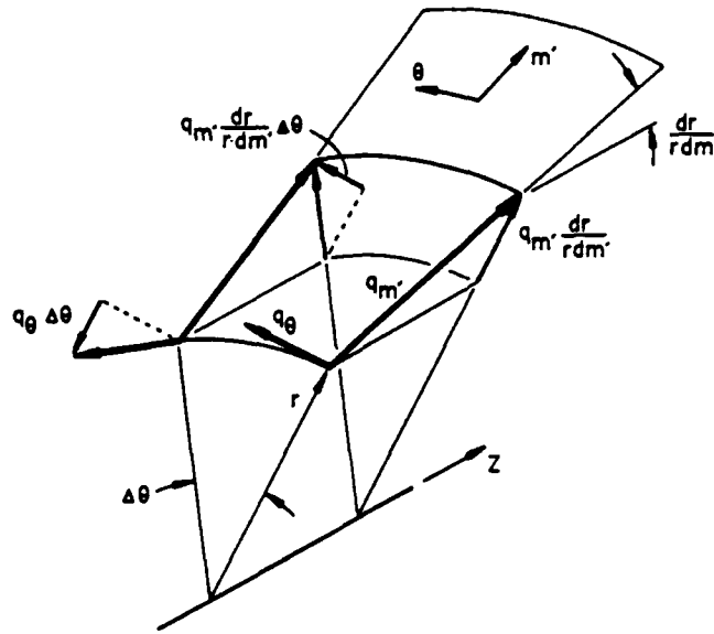
Figure A.4: Flux terms from circumferential displacement of velocity vectors
