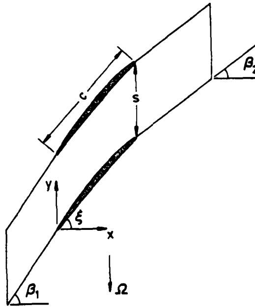
Figure 2.1: Cascade coordinate system
