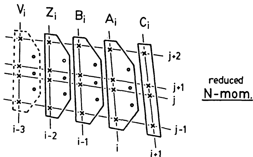
Figure D.10: Domain of dependence for reduced N-momentum equation across stagnation streamline.
