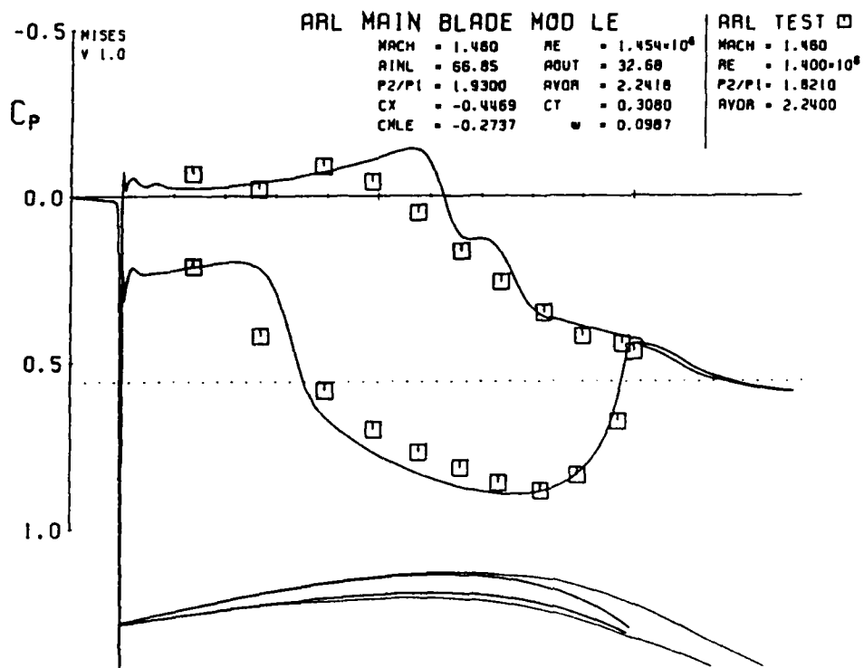
Figure 5.1: Pressure distribution for main blade at p_2/p_1 = 1.93 , 109% AVDR
