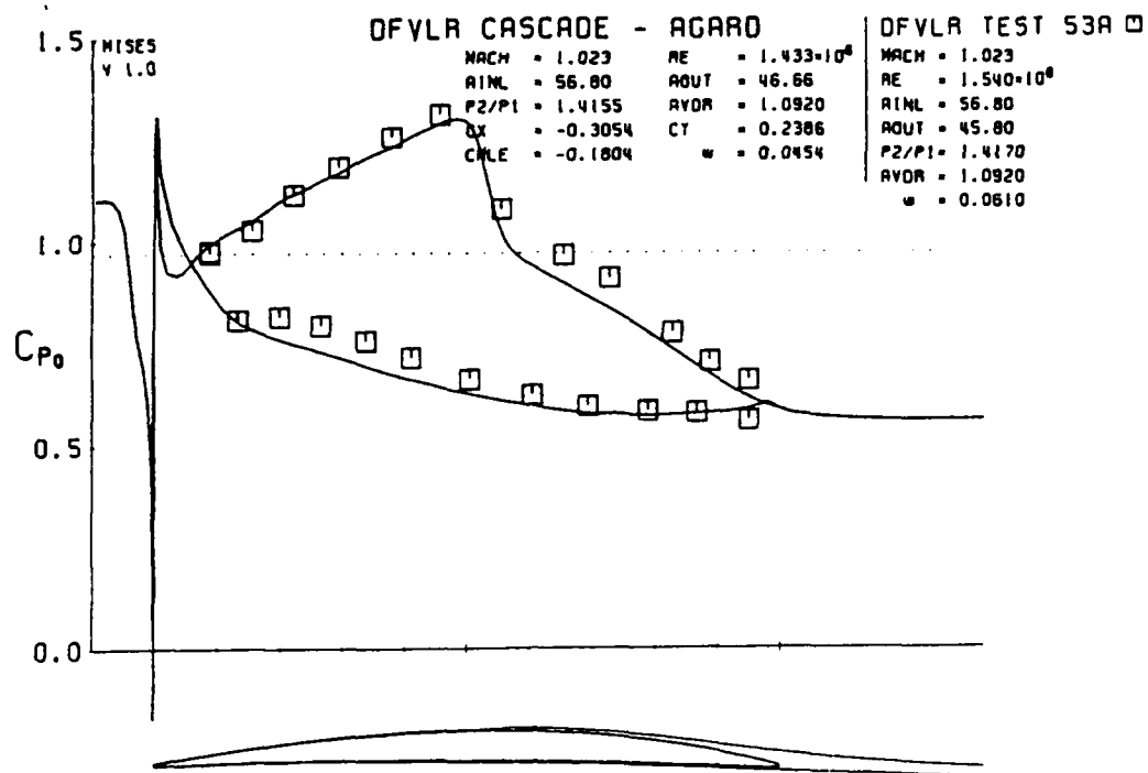
Figure 4.10: DFVLR blade: M = 1.023 , \beta_1 = 56.8^\circ , AVDR = 1.092
