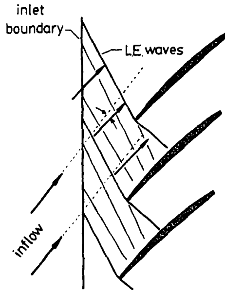
Figure 2.6: Supersonic/axially-subsonic inflow for cascade, showing inlet wave system
