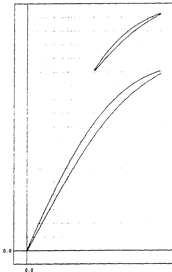
Figure 4.14: Blade and splitter vane for ARL cascade
