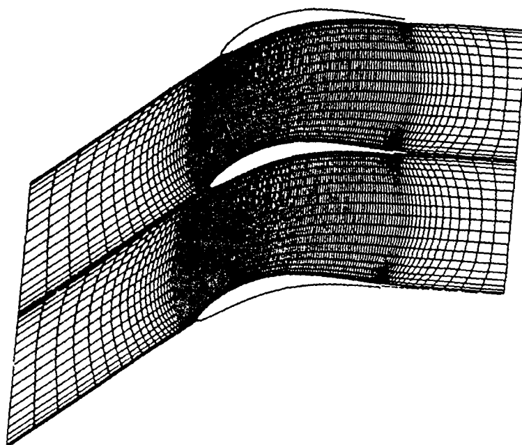
Figure 4.1: UTRC test case grid 132x20
