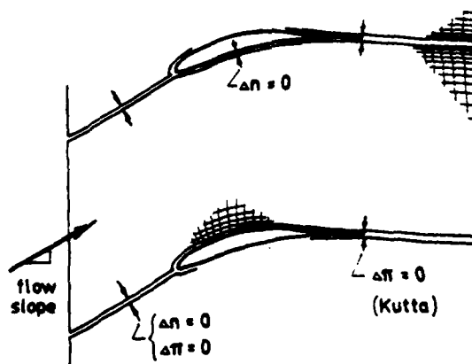
Figure 3.3: Boundary conditions on domain boundaries.
