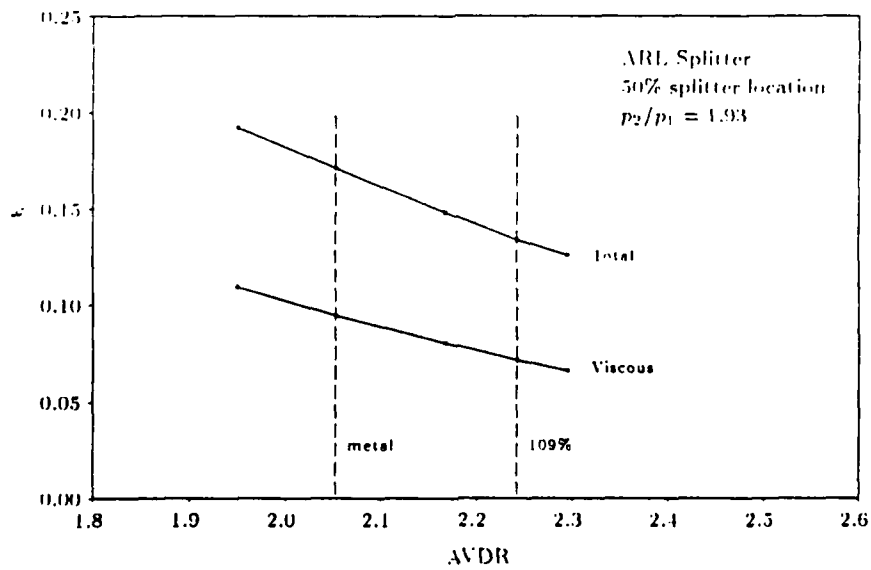
Figure 4.19: Effect of AVDR on total and viscous loss for ARL cascade
