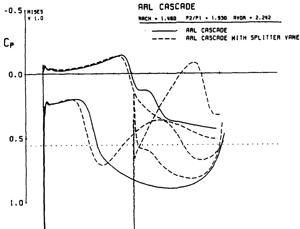
Figure 1.2: Effect of splitter vane on pressure distributions for ARL cascade.
