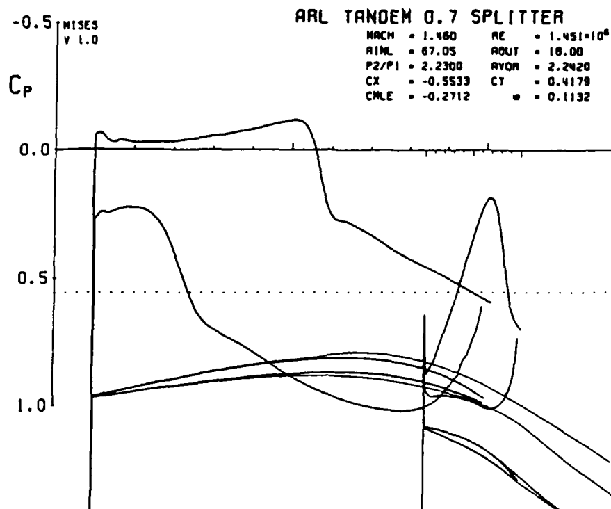
Figure 5.14: Surface pressures for 70% chord tandem splitter, 109% AVDR.
