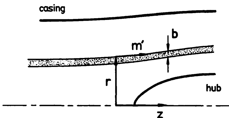
Figure 2.3: Meridional ( r - z ) plane for defining stream surfaces
