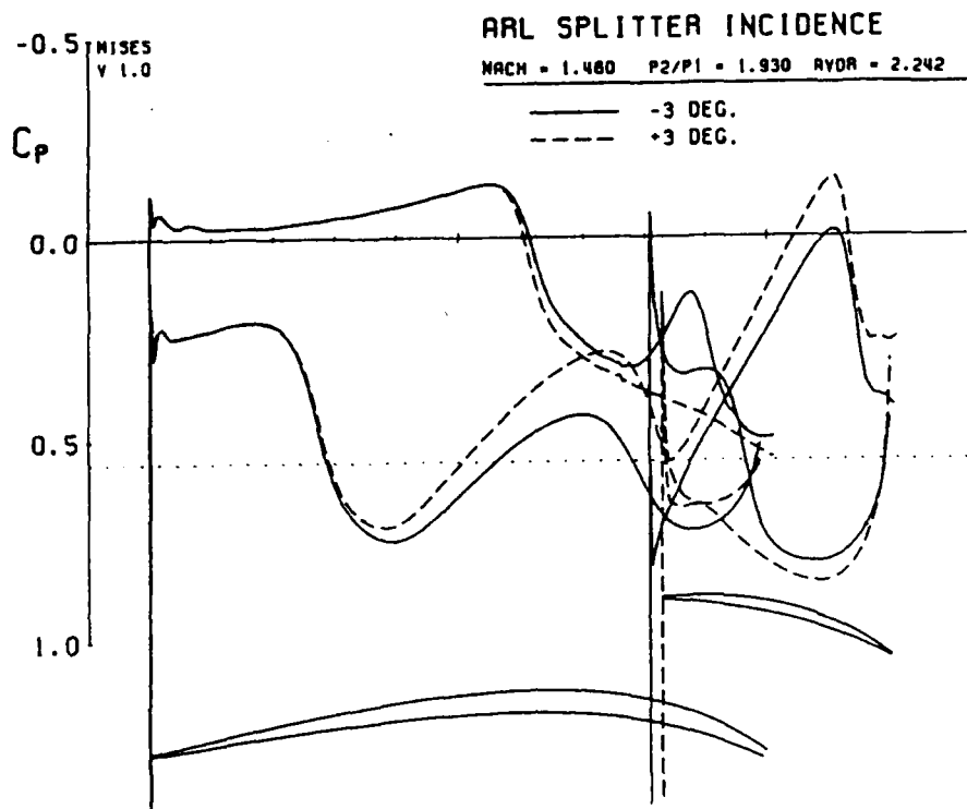
Figure 5.8: Surface pressures for ARL cascade at \pm 3^\circ splitter incidence
