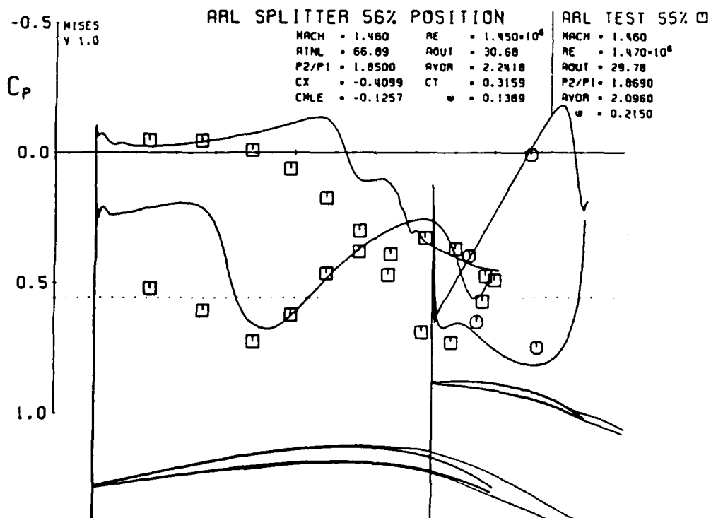
Figure 5.5: Pressure distribution for ARL cascade with 56% splitter position
