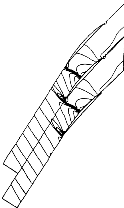
Figure 4.13: Mach contours for DFVLR blade, M = 1.086 , contour interval 0.05
