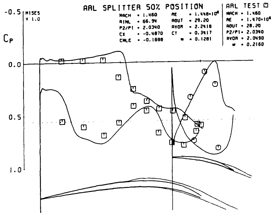
Figure 4.22: Surface pressures for ARL with splitter. p_2/p_1 = 2.034 , 109^\circ AVDR.
