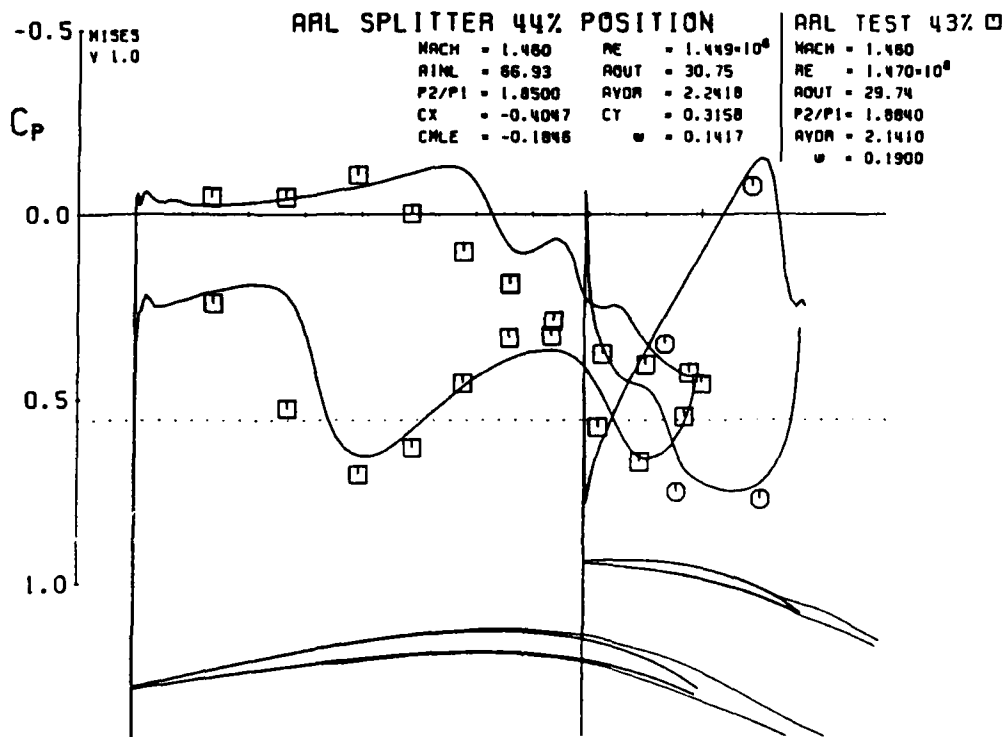
Figure 5.4: Pressure distribution for ARL cascade with 44% splitter position
