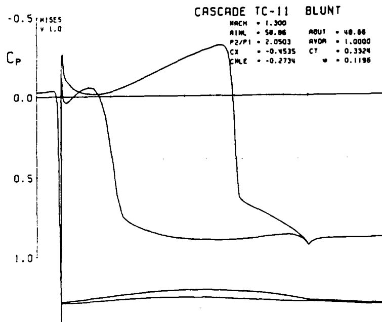
Figure 3.14: Pressure distribution for supersonic cascade with offset-periodic grid.
