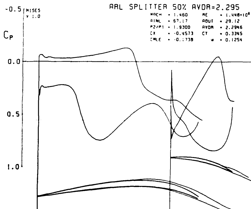
Figure 4.21: Pressure distribution for AVDR = 2.295.
