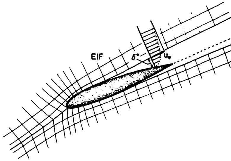
Figure 2.4: Equivalent inviscid flow defined by BL displacement thickness
