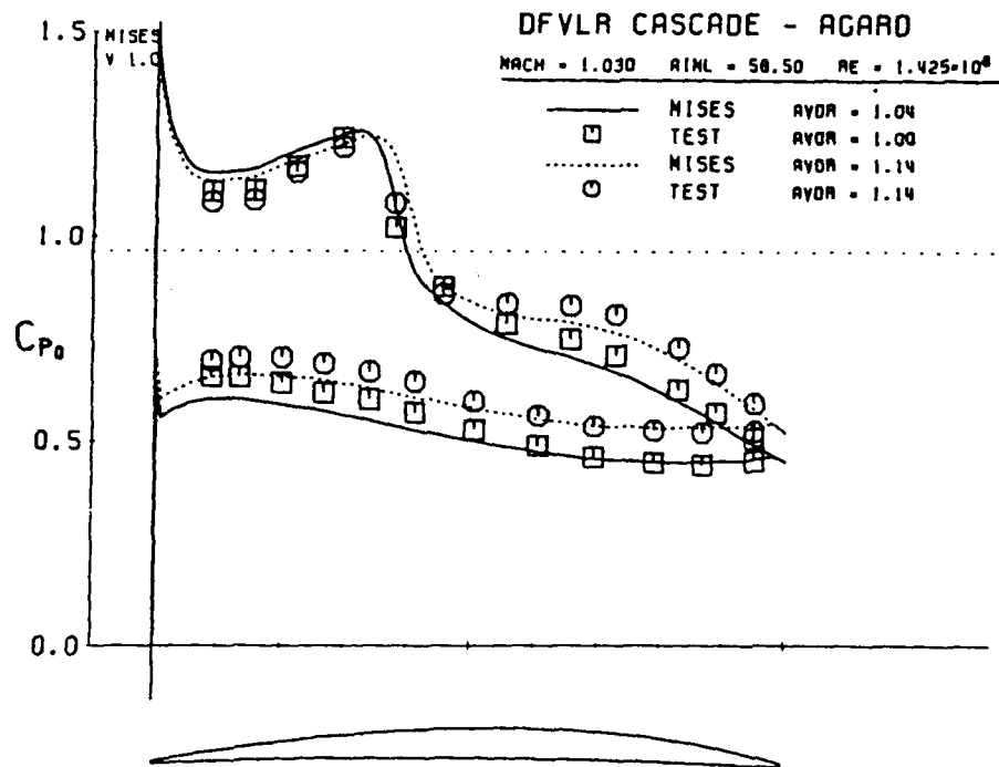
Figure 4.7: AVDR Effect on DFVLR blade: M = 1.03 , \beta_1 = 58.5^\circ .
