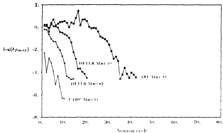
Figure 4.29: Convergence of Max density change for analysis cases
