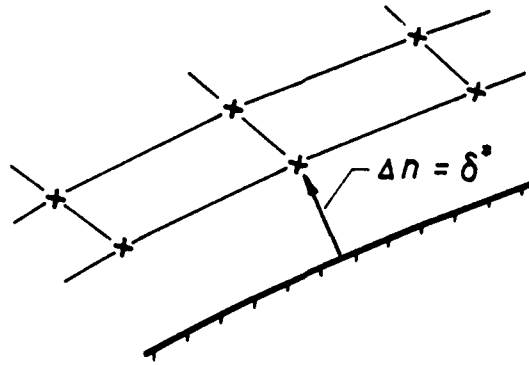
Figure 3.5: Boundary conditions for viscous coupling.
