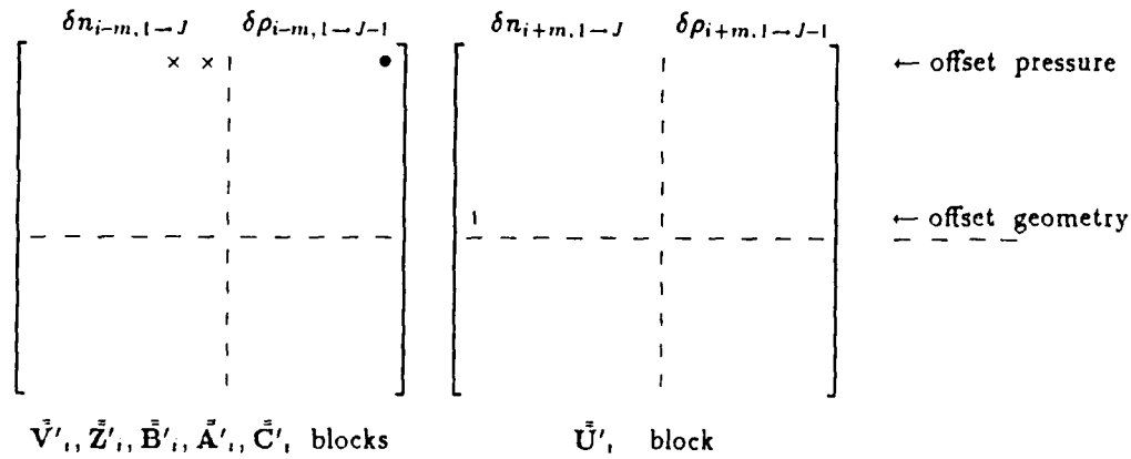
Figure D.12: Structure of lower and upper triangle blocks for offset-periodic matrix
