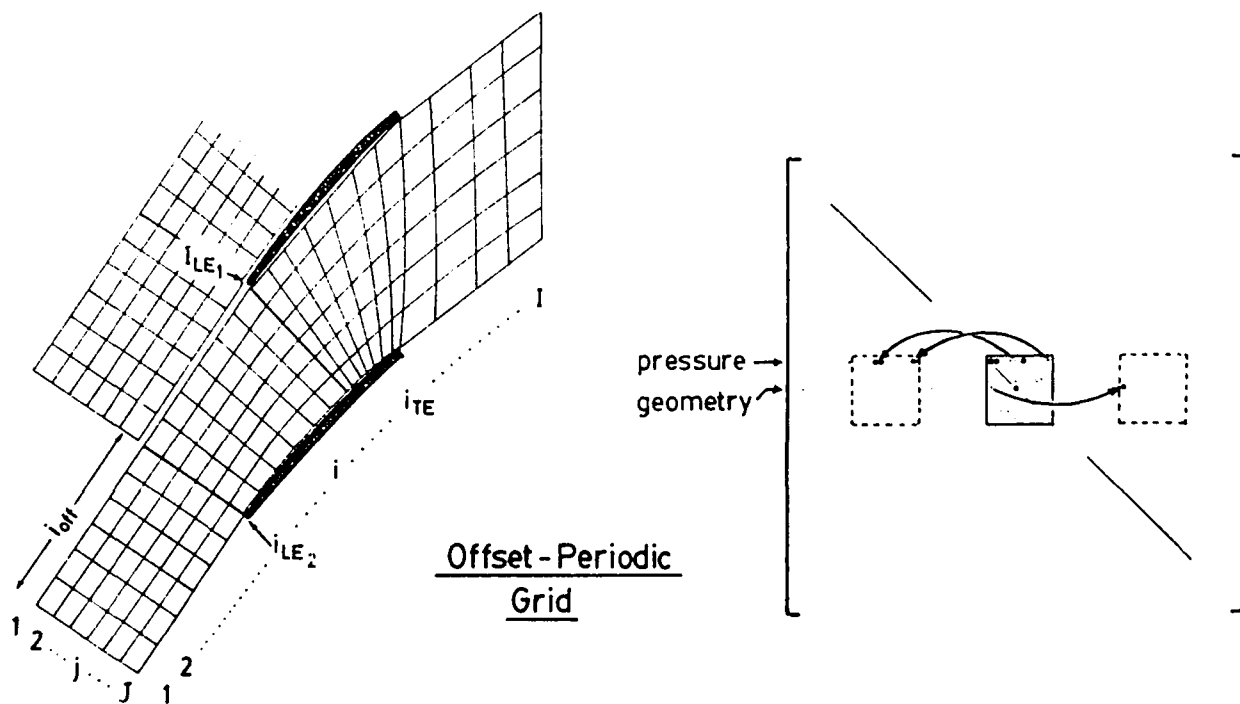
Figure D.11: Offset-periodic inlet geometry and indexing.
