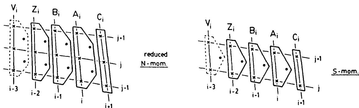
Figure D.2: Domain of dependence for S-momentum and N-momentum equations.
