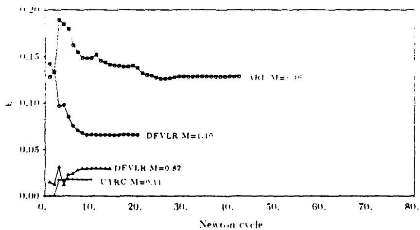
Figure 4.30: Convergence of loss for analysis cases
