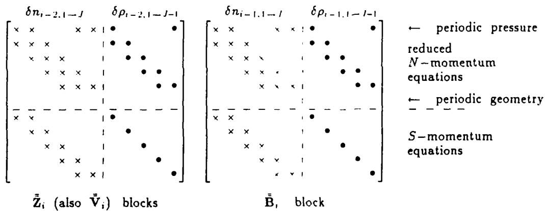
Figure D.4: Structure of \bar{\bar{Z}}_i and \bar{\bar{B}}_i blocks.
