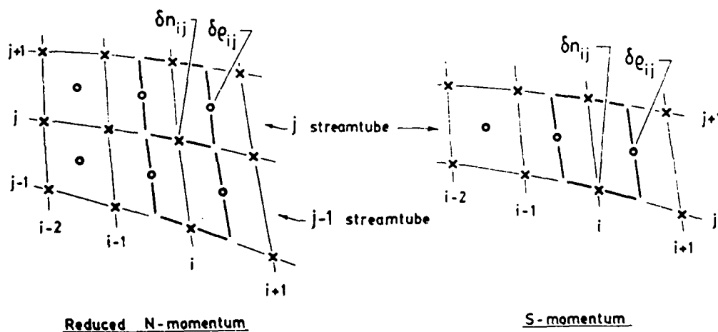
Figure D.1: Newton variables for discrete Euler equations.
