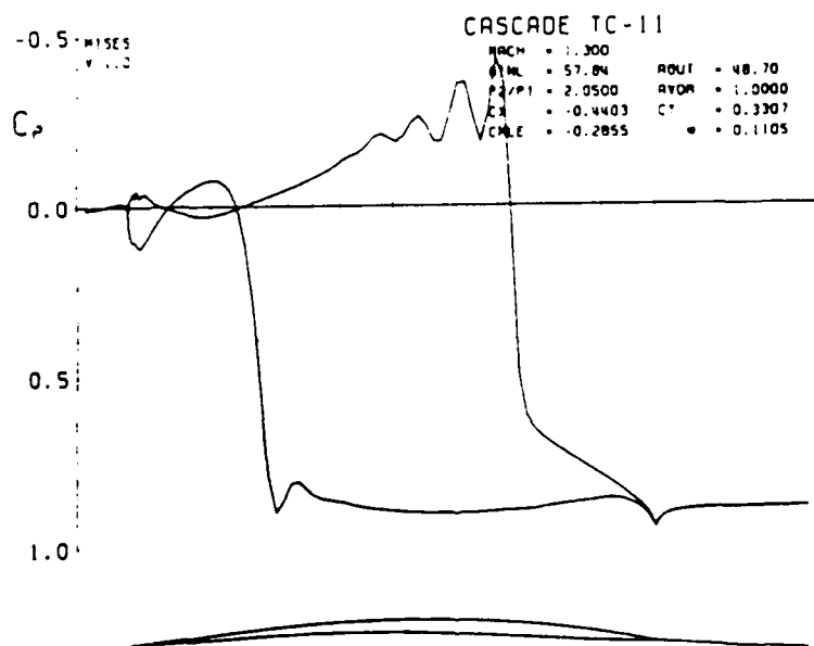
Figure 3.10: Dispersion effects at shock for skewed grid.
