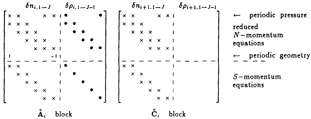
Figure D.3: Structure of \bar{\bar{A}}_i and \bar{\bar{C}}_i blocks.
