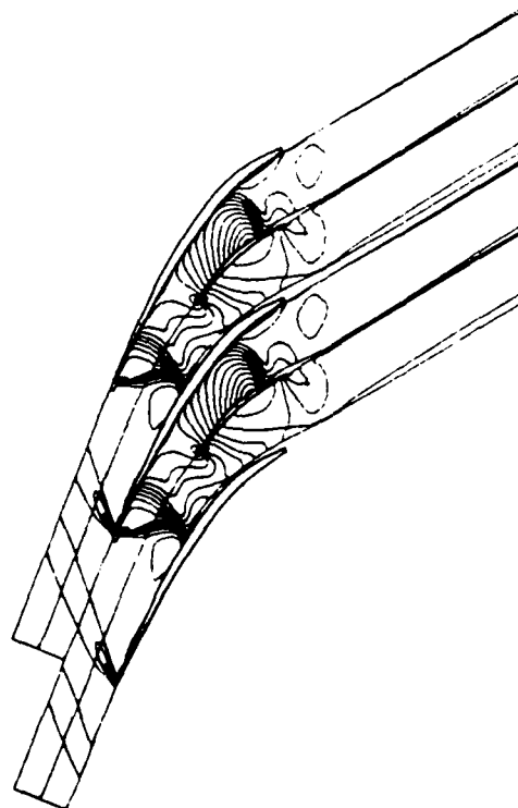
Figure 4.23: Mach contours for ARL cascade. contour interval 0.05, p_2/p_1 = 2.034
