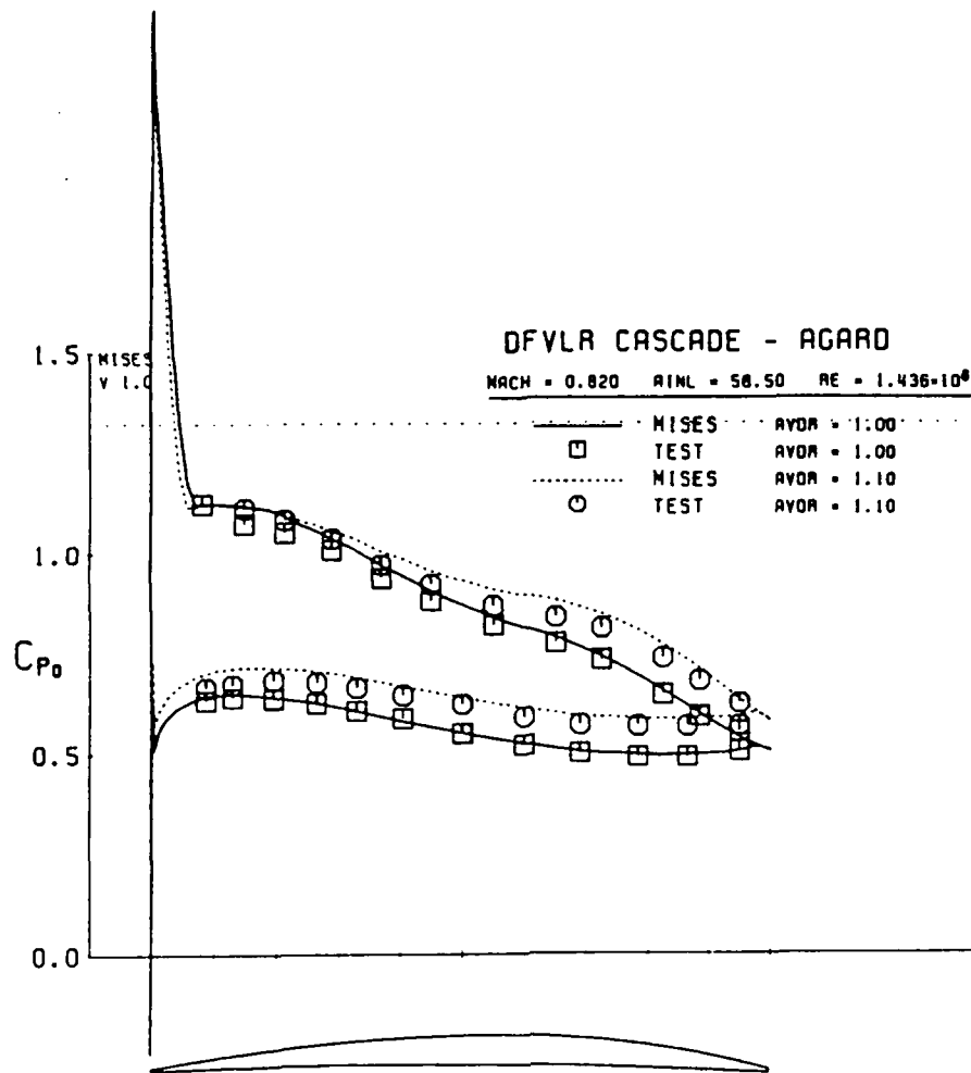
Figure 4.5: AVDR Effect on DFVLR blade: M = 0.82 , \beta_1 = 58.5^\circ .
