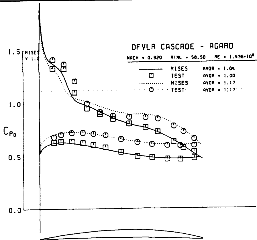
Figure 4.6: AVDR Effect on DFVLR blade: M = 0.92 , \beta_1 = 58.5^\circ .
