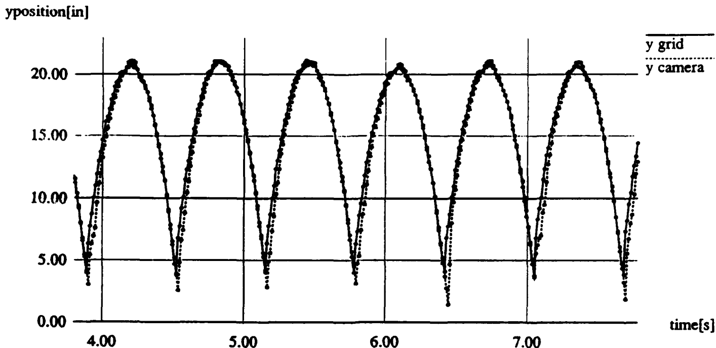
Fig. 13: Comparison of Steady State Performance (y position) between Vision and Inductive Sensing
