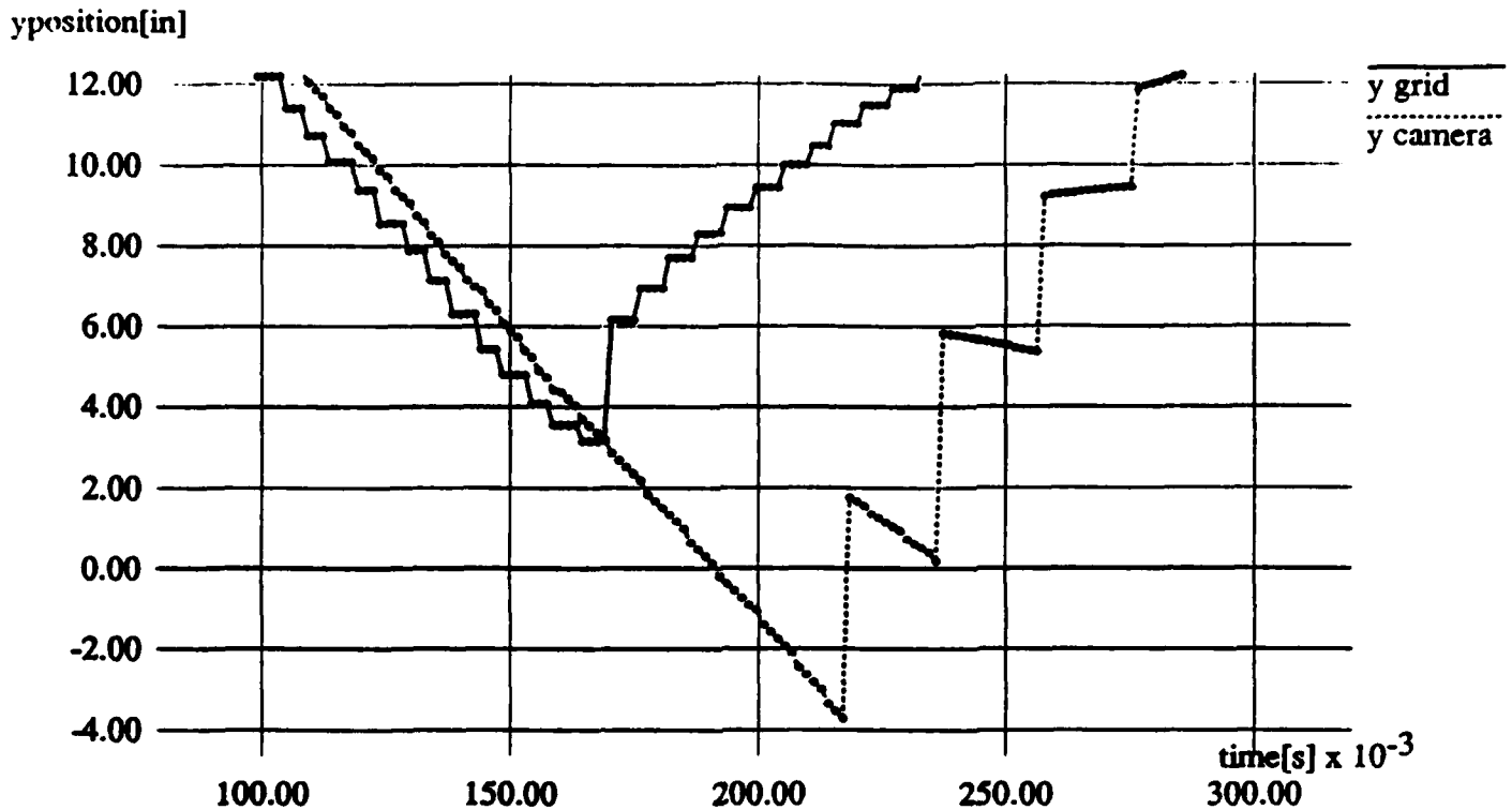
Fig. 9: Output (y position) of the Linear Observer
