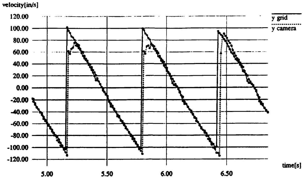
Fig. 12: (y) Velocity Estimates
