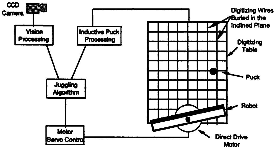
Fig. 1: Configuration of the Planar Juggler
