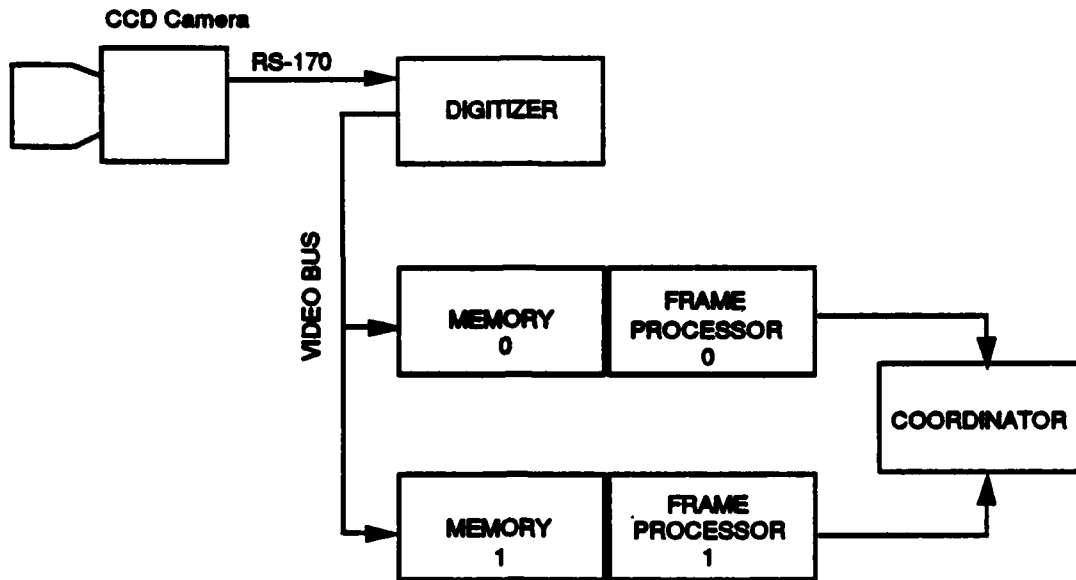
Fig. 4: The Cyclops Vision System
