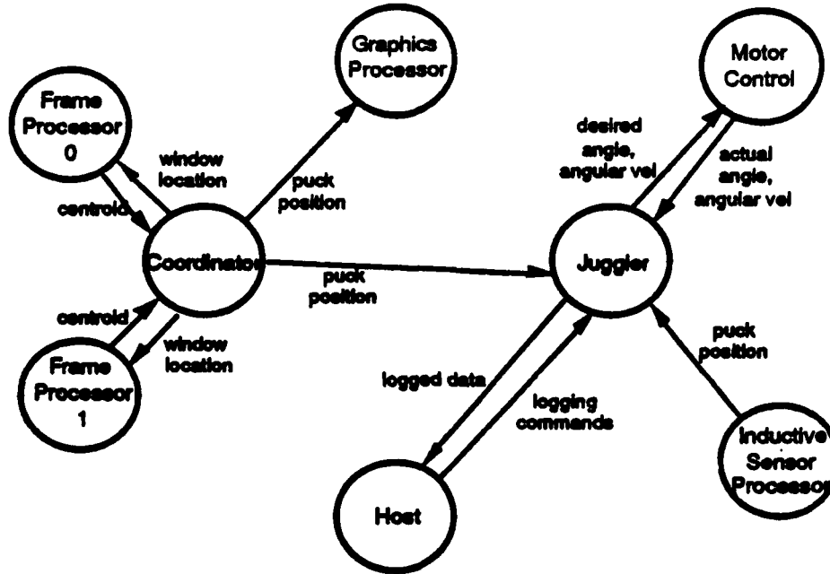
Fig. 6: The MIMD Architecture for the Juggler
