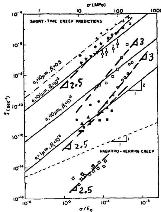
Fig. 2. Steady-state creep characteristics of polycrystalline alumina and alumina-silicon carbide composite. See [2] for details. The dark dashed lines come from the theory discussed in Section 2.2.4.
