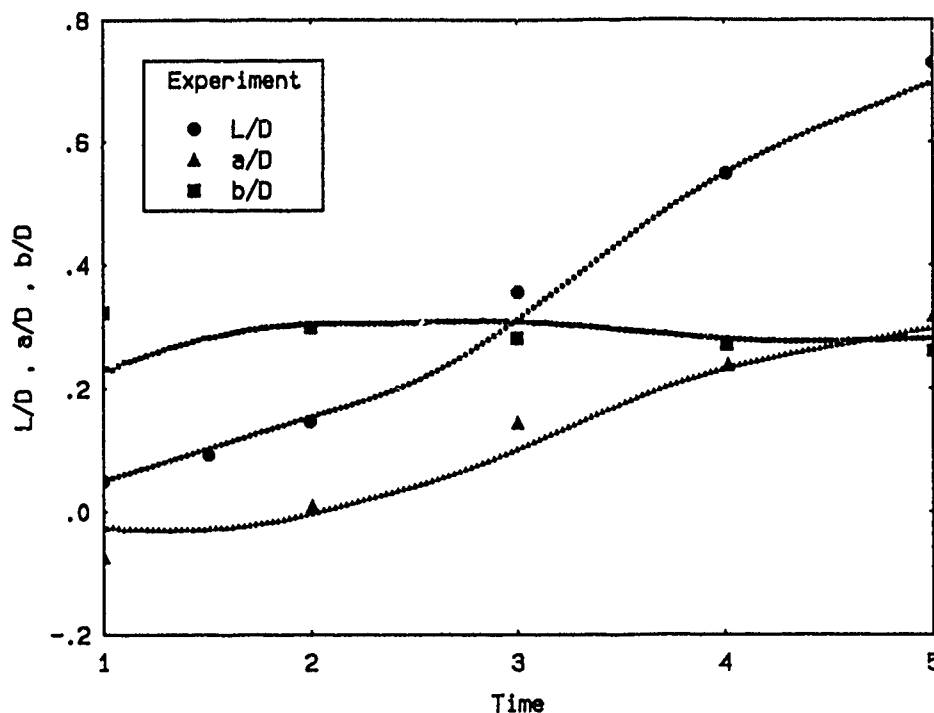
FIGURE 4.4.7 Comparison of the time history of the computed geometrical parameters of the closed wake for Re = 3000 with Bouard & Coutanceau measurements.
