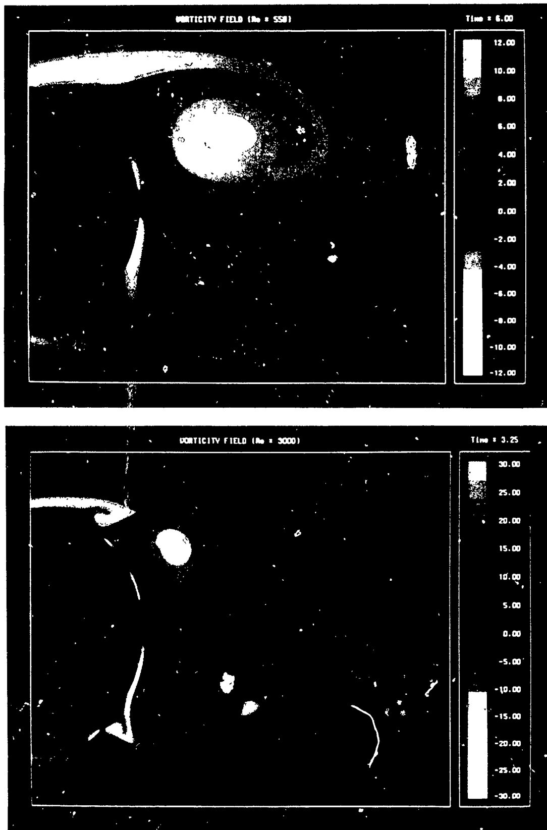
FIGURE C.1 Vorticity field for Re = 550 at T = 6 (top), and for Re = 3000 at T = 3.25 (bottom).
