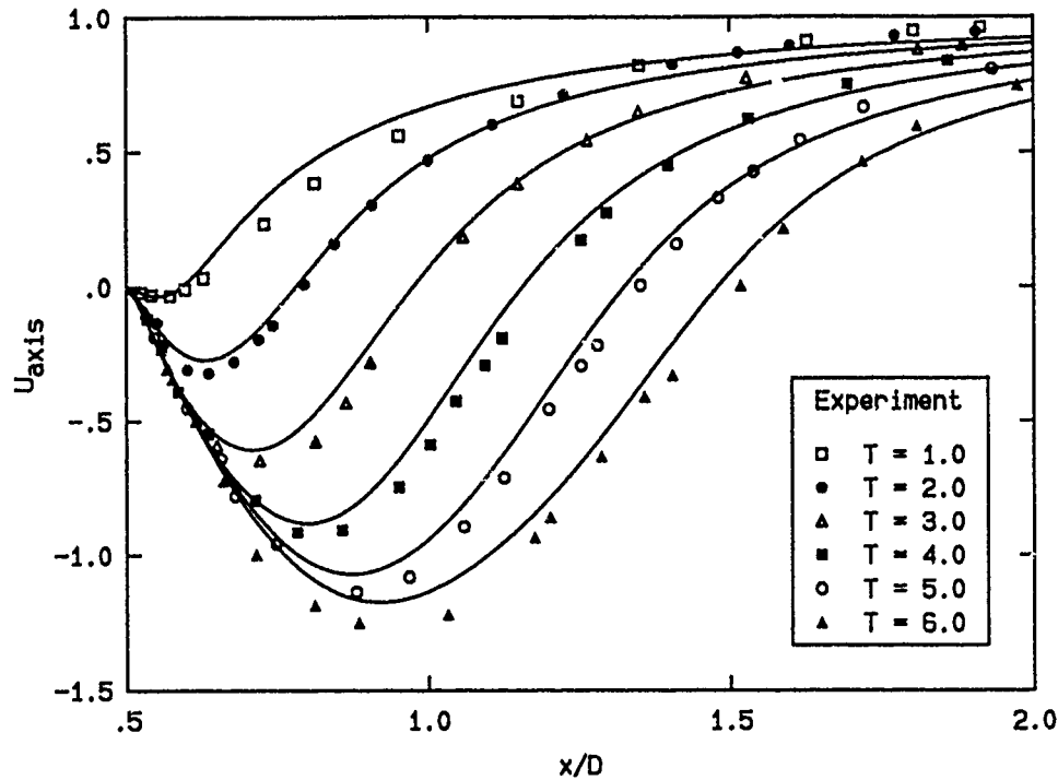
FIGURE 4.4.5 Comparison of the velocity on the symmetry axis for Re = 550 obtained numerically (solid lines) and experimentally.
