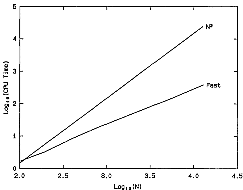
FIGURE 3.1.2 Performance of the fast algorithm
