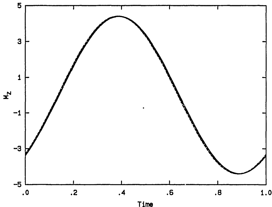
FIGURE 2.3.3 Moment on the cylinder obtained analytically (solid) and numerically for 44 (dash) and 62 (dot-dash) layers of particles.
