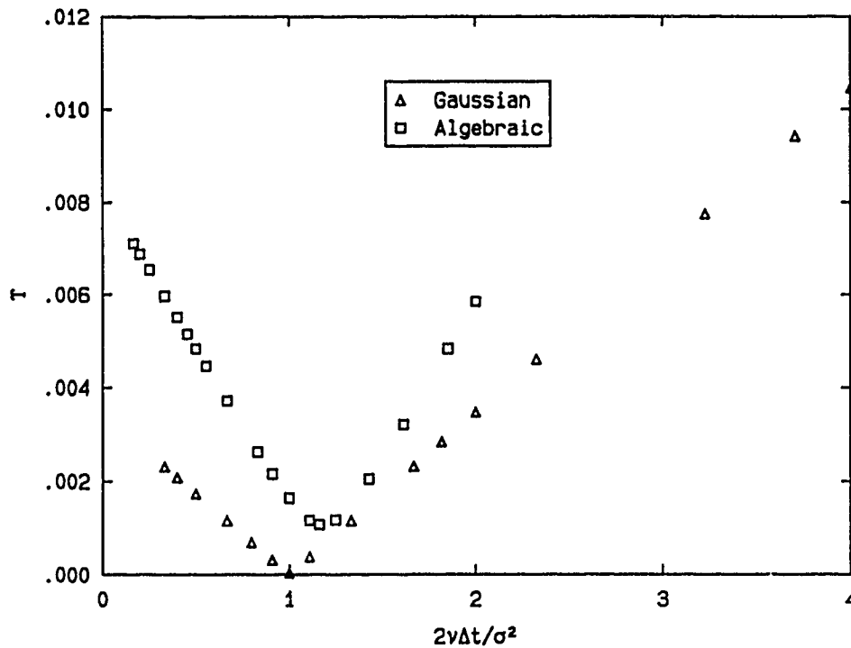
FIGURE 2.2.4 Accuracy of the weight redistribution method.
