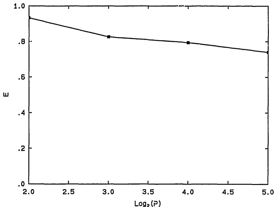
FIGURE 3.5.1 Parallel efficiency of the fast algorithm.
