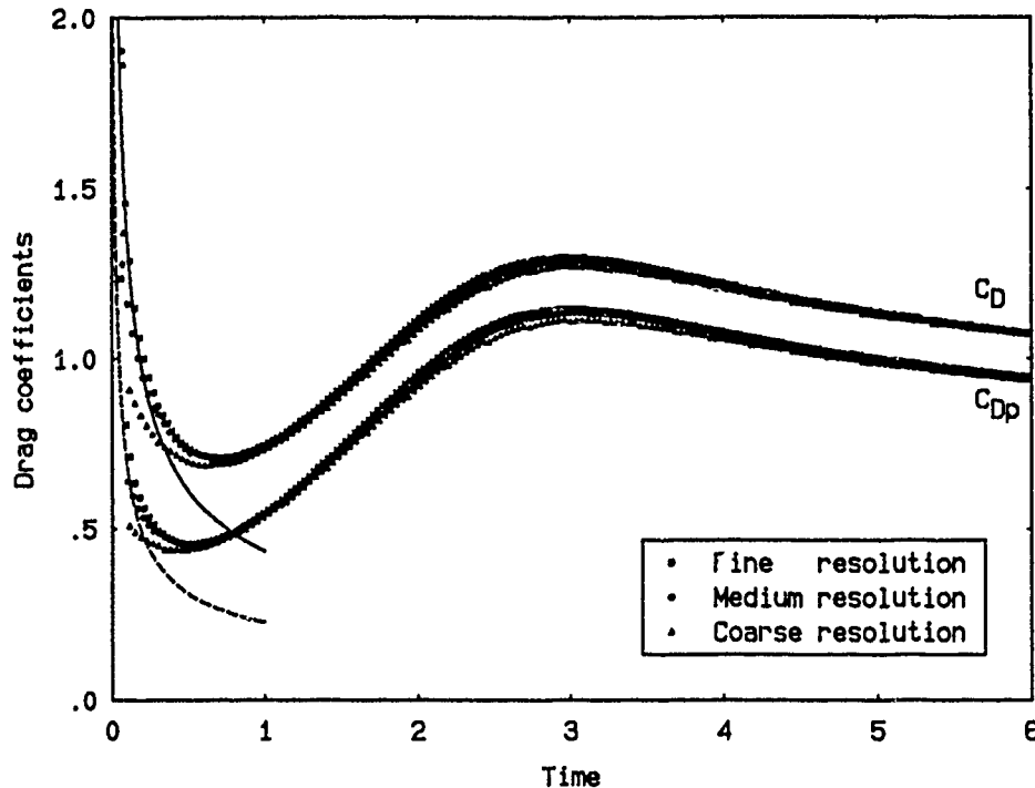
FIGURE 4.3.3 Convergence study of the drag coefficients time history and comparison with Bar-Lev & Yang analytical results (solid and dash lines).
