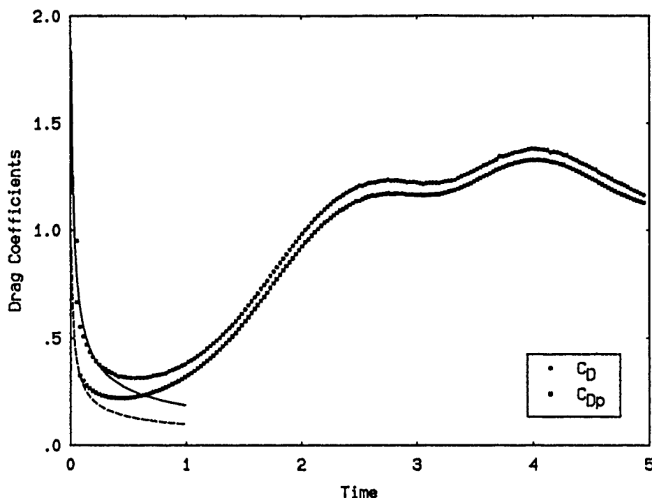
FIGURE 4.4.9 Comparison of time history of the numerical drag coefficients with Bar-Lev & Yang analytical solution (solid and dash lines) for Re = 3000 .
