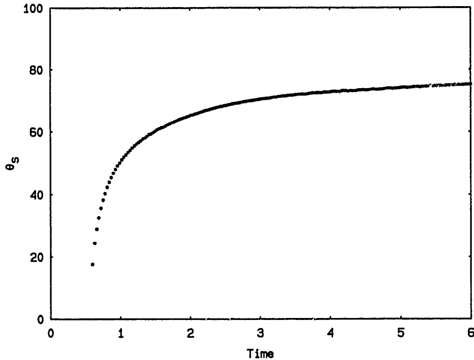
FIGURE 4.4.3 Time history of separation angle for Re = 550 .
