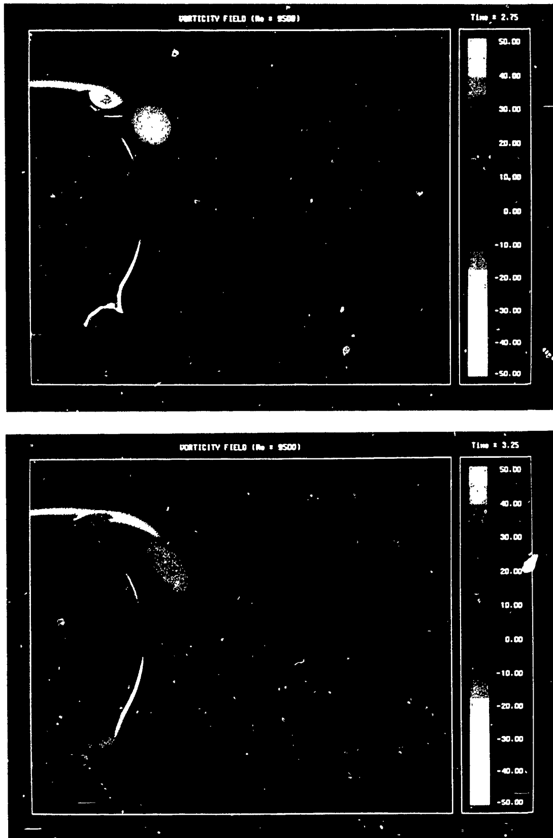
FIGURE C.2 Vorticity field for Re = 9500 at T = 2.75 (top), and at T = 3.25 (bottom).
