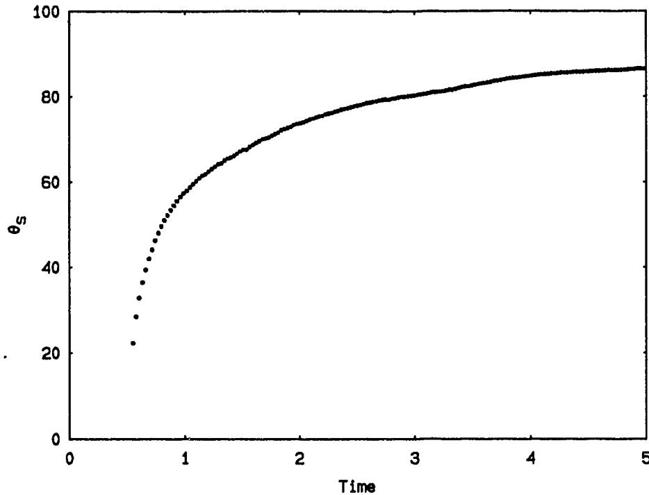
FIGURE 4.4.8 Time history of separation angle for Re = 3000 .
