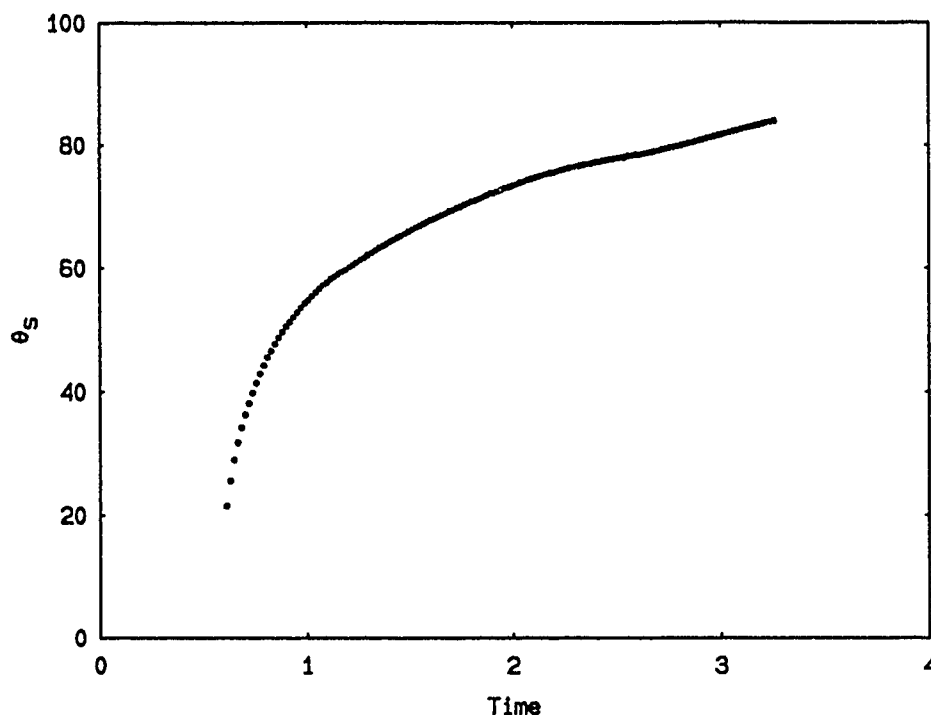
FIGURE 4.4.14 Time history of separation angle for Re = 9500 .
