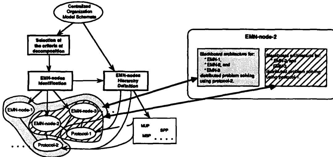
Figure 3-31: Example of task decomposition
