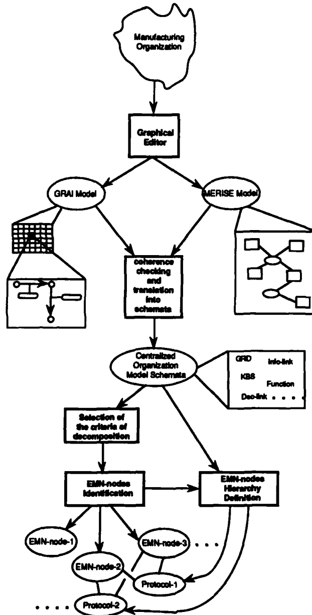
Figure 3-1: EMN architecture instantiation
