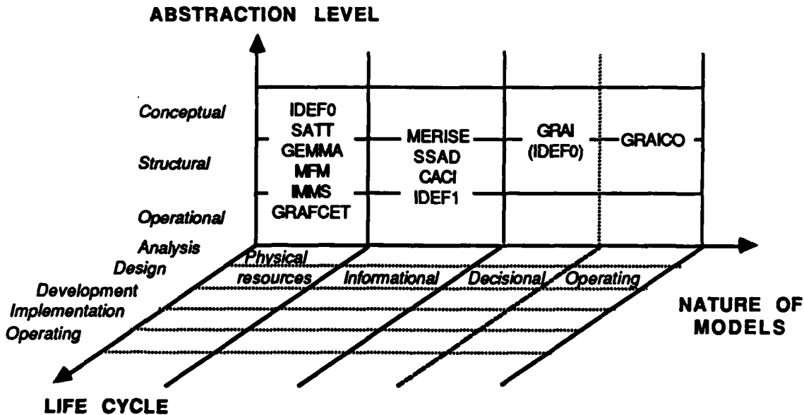
Figure 3-2: Methodologies typology
