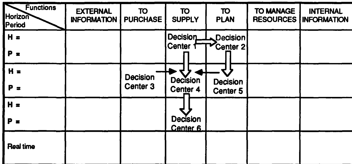
Figure 3-5: GRAI grid
