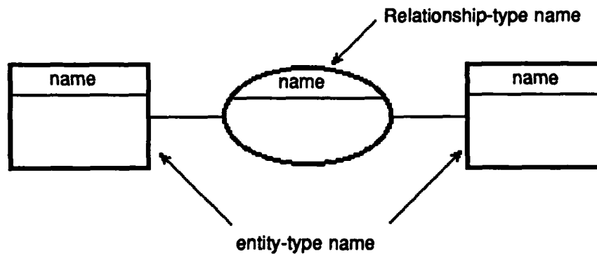
Figure 3-22: The entity/relationship model
