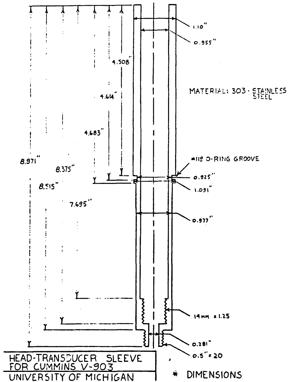
Figure 5-17. Pressure-Transducer Sleeve
