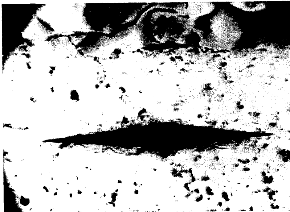
Figure 5-100. Cr 2 C 3 Coating, Unworn, Surface Layer Thickness 0.18 mm, 0.1 and 1.0 Kg Load Vickers Test, Scattered Cracks, Objective Lens: 50/0.85, Photo Lens: X 10, Magnification: X 430
