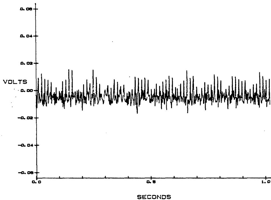
Figure 5-28. Original Strain-Gauge Bridge Noise, No Bridge Excitation
