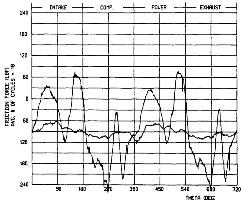
Figure 5-43. Strain-Gauge Signal Without Bridge Excitation Before and After Reduction of Magnetic Interference, 1200 RPM
