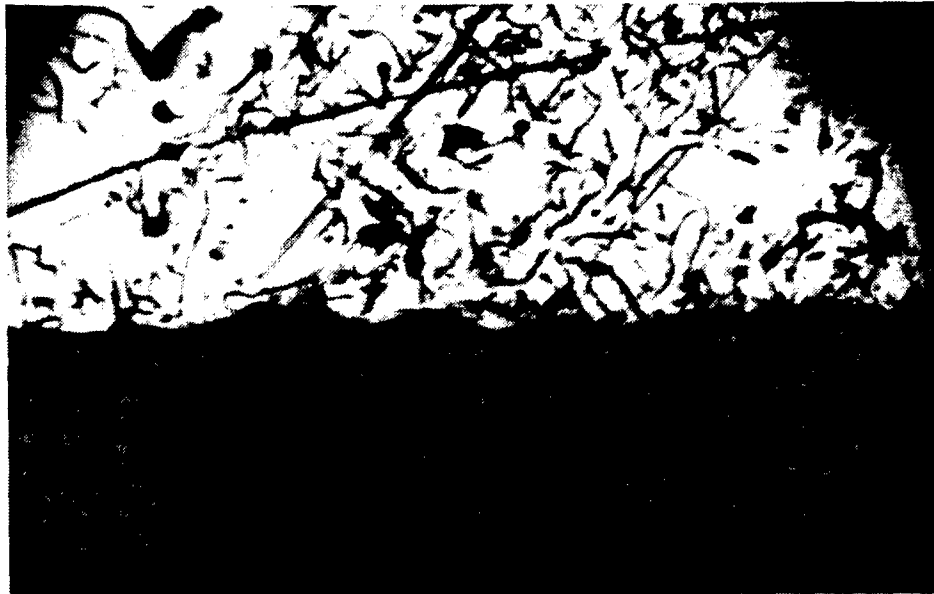
Figure 5-89. Cr2O3 Coated, 2 Kg Load Knoop Indenter Applied on Middle of Surface Layer, Cracks Along Corner Evident, #19, Build 4, Cylinder 3, T.R.R., Objective Lens: 16/0.22, Photo Lens: X 10, Magnification: X 155
