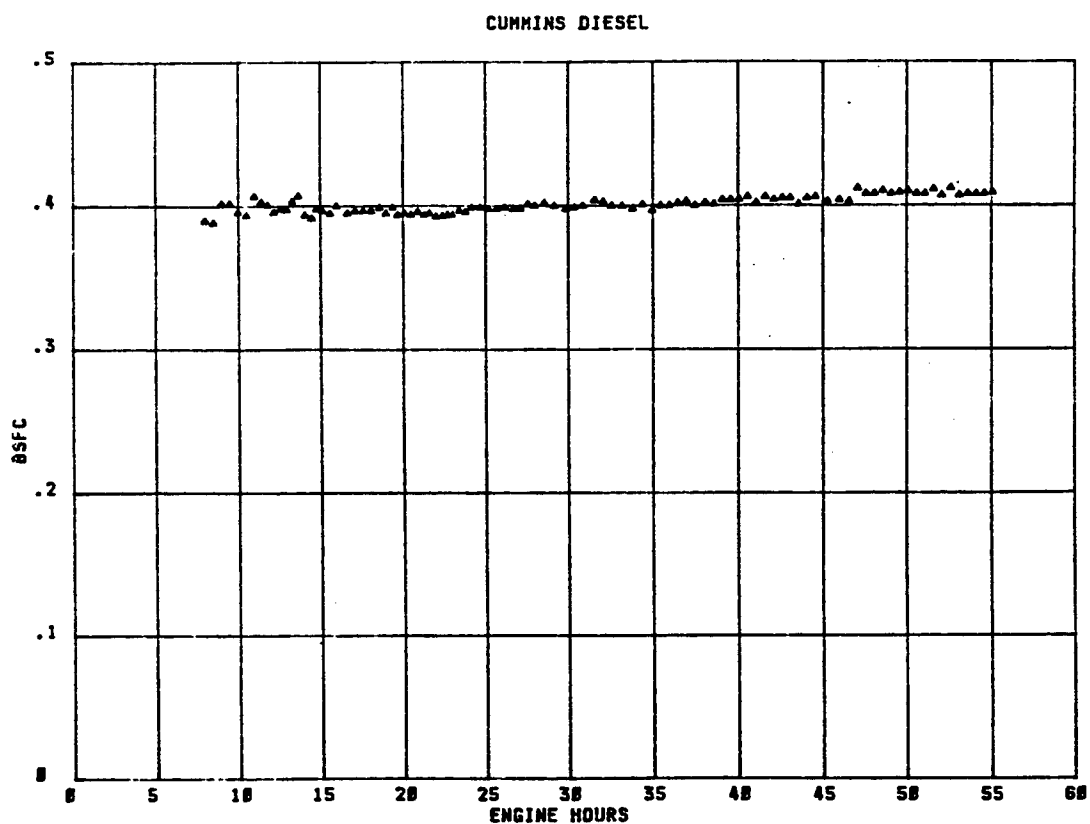
Figure 5-38. Brake Specific-Fuel Consumption During Break-In: BSFC units, lbm/bhp-hr
