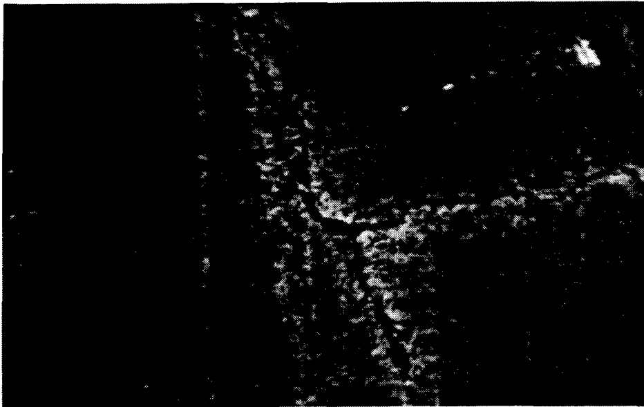
Figure 5-91. Cr2O3 Coated, Many Axial and Radial Cracks Exist Within 14-46 mm From Top Side of the Cylinder, #19, Build 4, Cylinder 3, T.R.R., Objective Lens: 16/0.22, Photo Lens: X 10, Magnification: X 155
