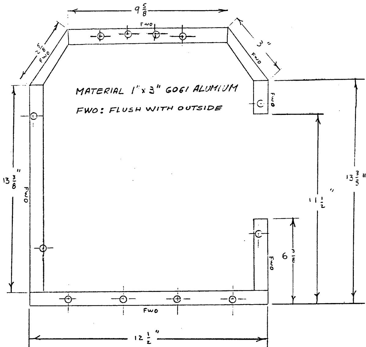
Figure 5-13. Oil-Pan Modifications
