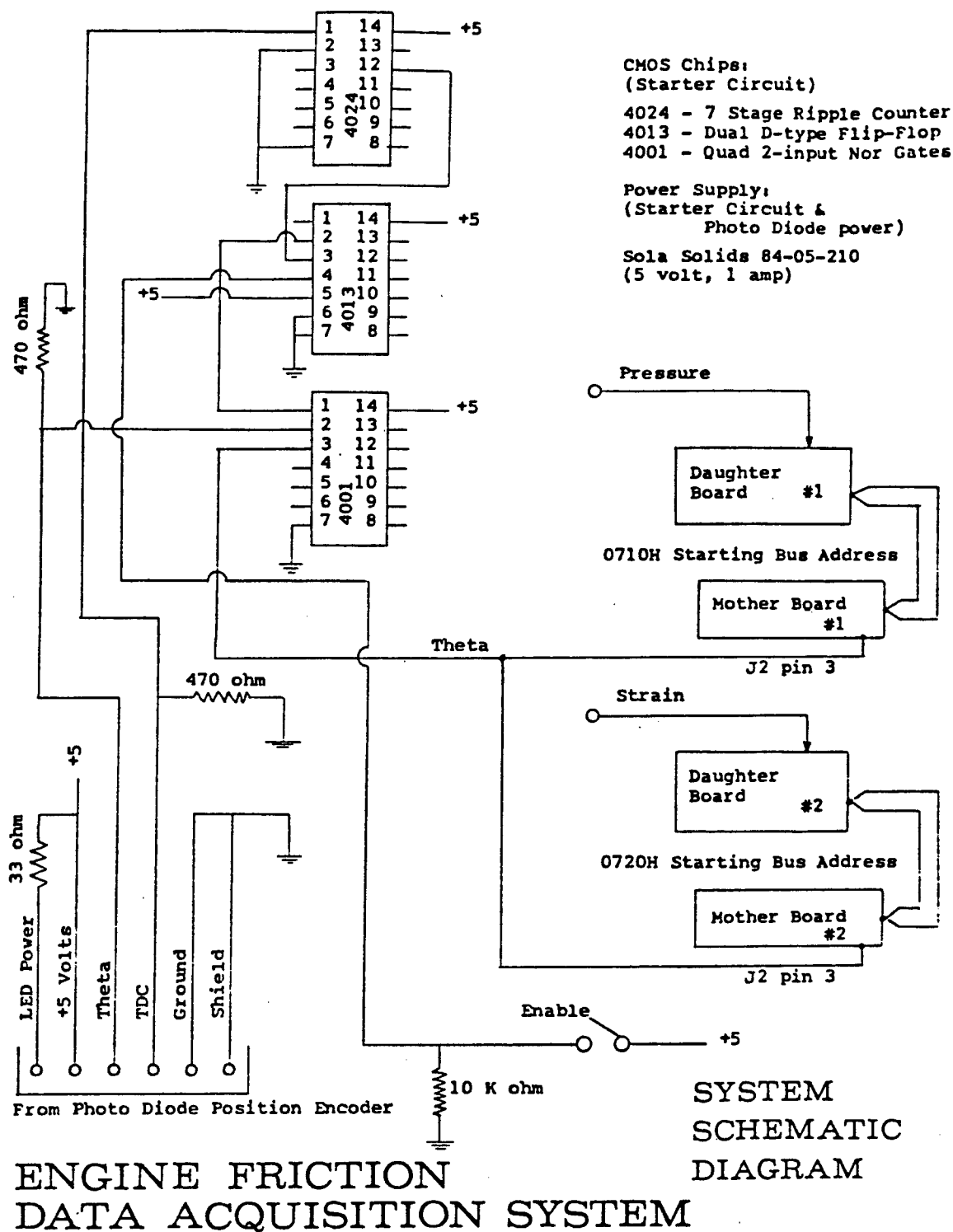
Figure 5-24. Schematic of Data Acquisition System
