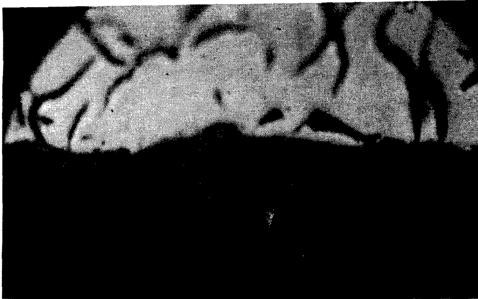
Figure 5-98. Cr 2 O 3 -Dipped Coating, Unworn, Surface Layer Thickness 0.035 mm, 0.1 Kg Load Vickers Test, Small Cracks at Left Corner, Objective Lens: 50/0.85, Photo Lens: X 10, Magnification: X 430
