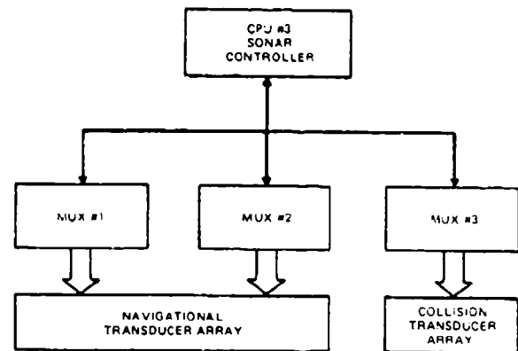
Figure 14. Block diagram of sonar multiplexing scheme which handles a total of 36 ultrasonic transducers.
