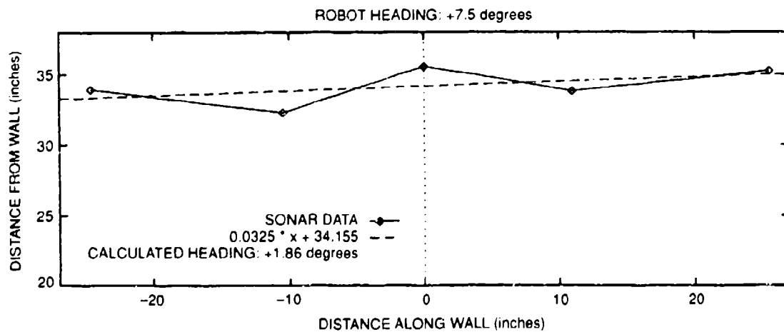
Figure 71b. A calculated angular offset of 1.86° is obtained for an actual orientation of +7.5°.
