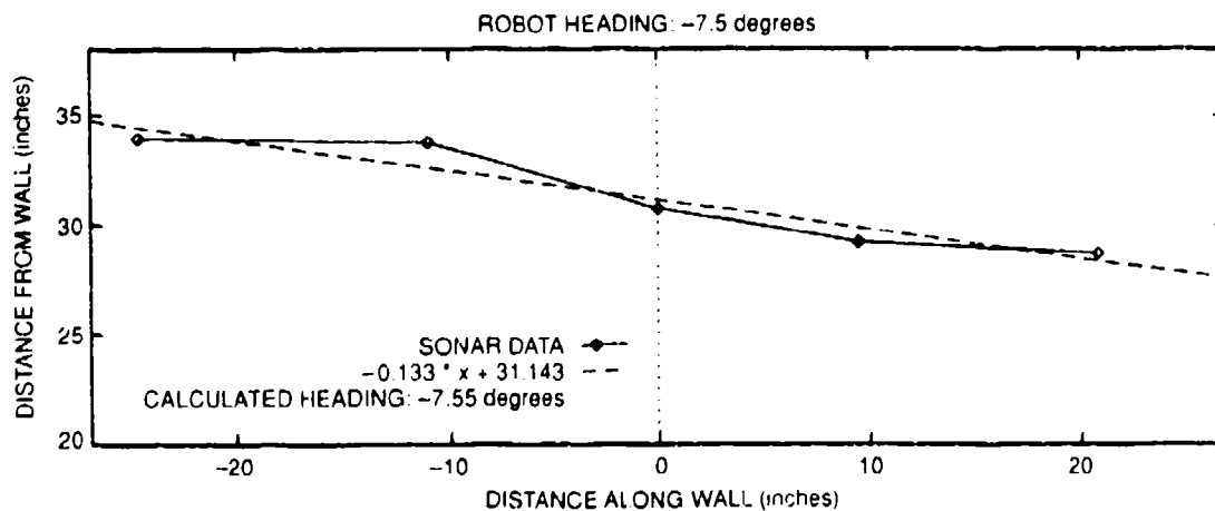
Figure 71c. A second line-fit operation is performed for an actual orientation of -7.5°, resulting in a calculated angular offset of -7.55°. Inconsistencies in performance are due primarily to specular reflection at the target surface.
