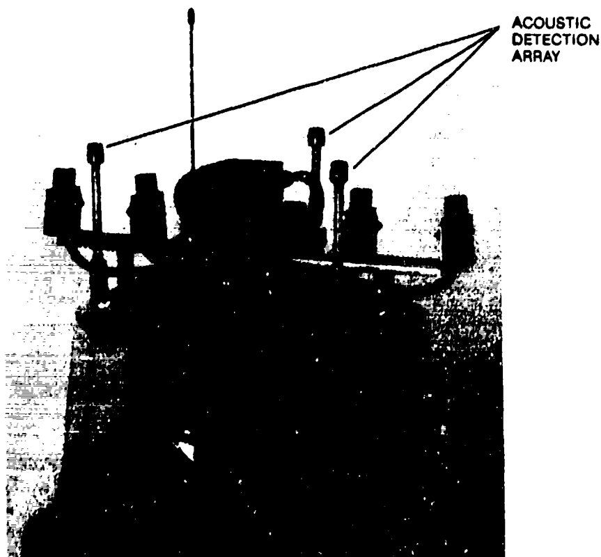
Figure 29. Three spring-mounted omnidirectional sensors are employed in the passive acoustical detection array mounted on the head as shown in this photo.
