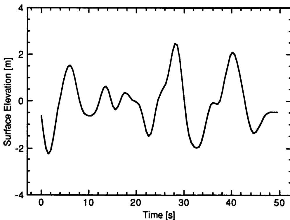
Figure 3. Simulated 4 m sea state (WMO sea state 5) waveform based on the Bretschneider spectrum: H_s = 4 \text{ m} , T_p = 12 \text{ s} .
