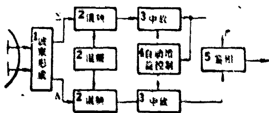
Fig. 1. Principal block diagram of passive radar guidance head Key: 1. Formation of wave beam 2. Mixing (frequency) 3. Intermediate amplification 4. Automatic gain control 5. Phase discrimination
