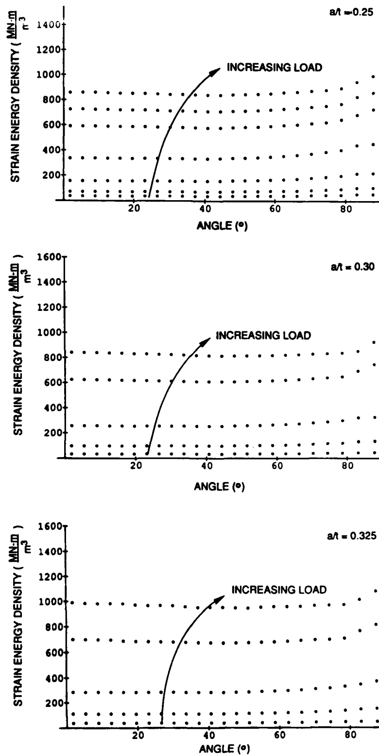
Fig. 16 — Strain Energy Density Profiles for Semi-Circular ( a/b = 1.0 ) Cracks In Tension
