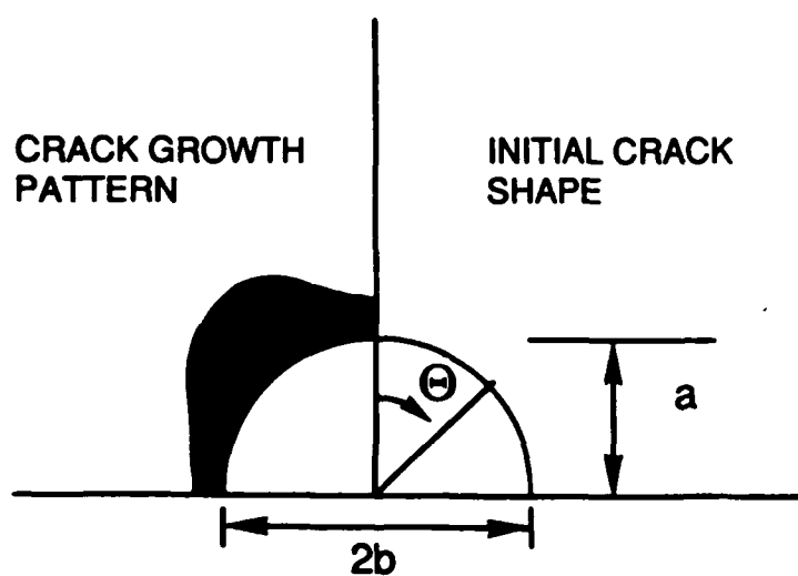
Fig. 28 — Critical Strain Energy Density Profiles and Crack Growth Patterns for Semi-Circular ( a/b = 1.0 ) Cracks In Bending
