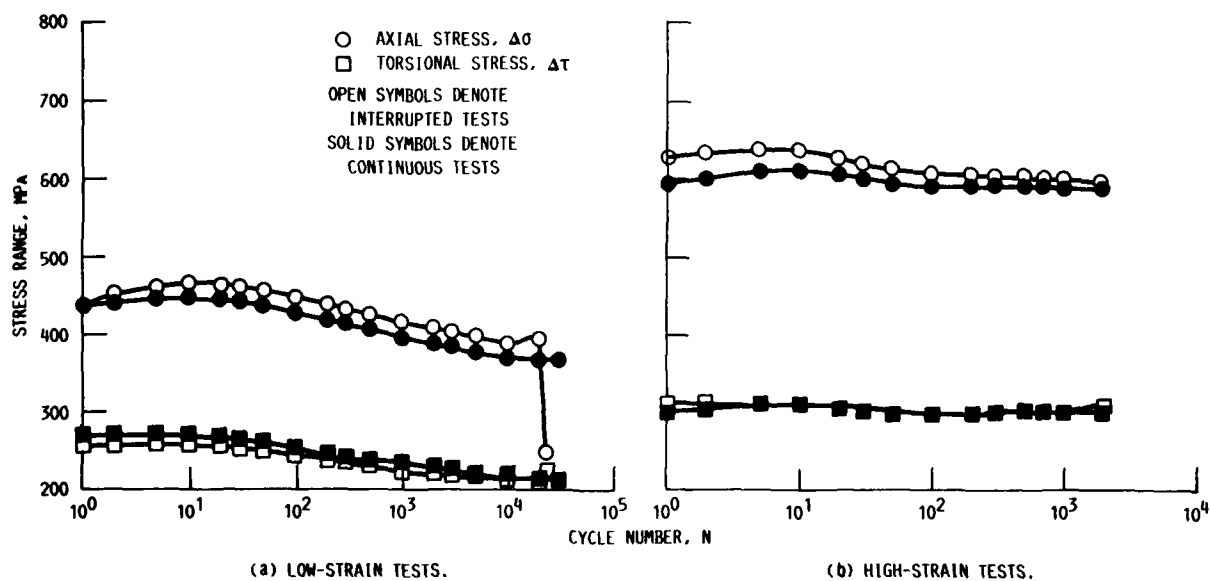
FIGURE 8. - STRESS RANGE VERSUS NUMBER OF CYCLES.
