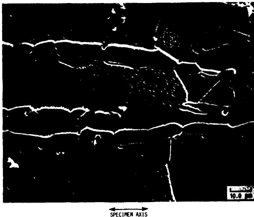
FIGURE 6. - MICROSTRUCTURE OF AISI 304 STAINLESS STEEL. THE ELONGATED FERRITE GRAINS FOLLOW THE EXTRUSION DIRECTION OF THE BAR. ETCHANT, 10 PERCENT OXALIC ACID.
