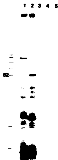
FIGURE 1. Incorporation of [ ^3\text{H} ]leucine into mechanically released C. burnetii proteins during heat shock. Intracellular organisms were obtained from mechanically disrupted fibroblasts, isolated from host components, and acid activated at pH 4.5 in a medium containing glucose, glutamate, amino acids with [ ^3\text{H} ]leucine, and buffered salts. Incubations were carried out for 12 h. Proteins were extracted by boiling in SDS with \beta -mercaptoethanol and electrophoresed through gradient polyacrylamide gels, which were then subjected to fluorography; a radioautogram is shown. (Lane 1) Proteins labeled during a 12-h incubation at 21°C. (Lane 2) Proteins labeled during incubation at 21°C for 6 h followed by a 6-h incubation at 42°C (heat shock). (Lane 3) Proteins labeled during acid activation in the presence of chloramphenicol (1.5 mM) and heat shocked as in lane 2. (Lane 4) Soluble supernatant proteins from organisms incubated at 21°C. (Lane 5) Soluble supernatant proteins from organisms exposed to heat shock. The position of the 62-kDa heat shock protein, which was identified with specific antibody and antisera, is indicated at the left. The locations of bands representing other proteins induced by heat shock are indicated by the horizontal lines at the left. Note the apparent change in migration of a 30-kDa protein after heat shock (lane 2).
