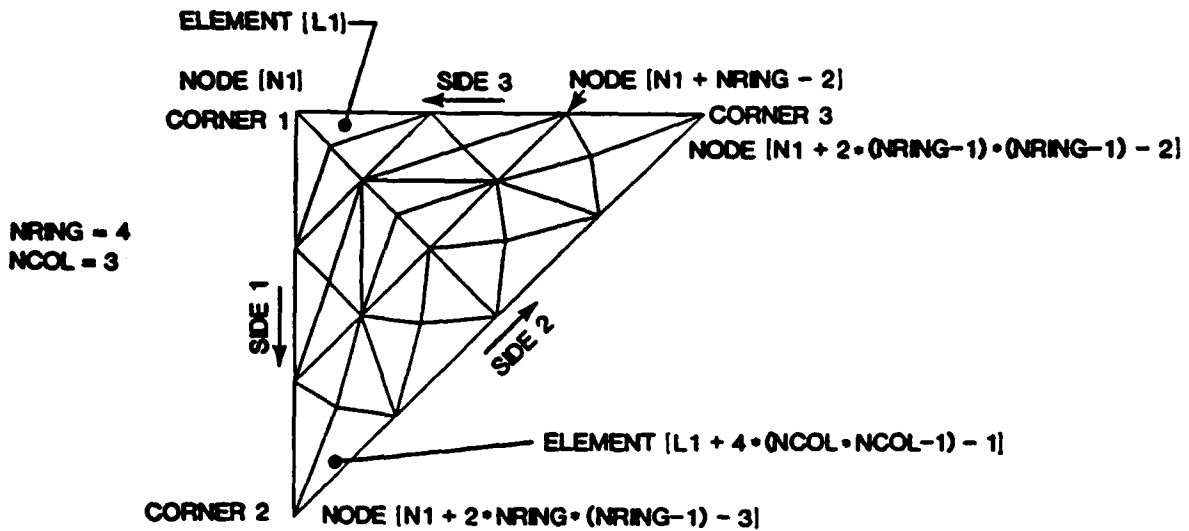
FIGURE 5. THREE-SIDED SHAPE GEOMETRY
