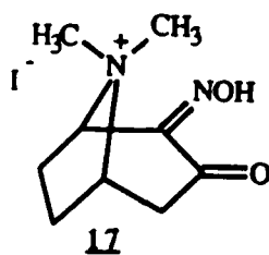
2-Oximino-tropan-3-one methiodide
