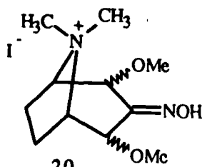
2,4-Dimethoxy-3-oximino-tropane methiodide
