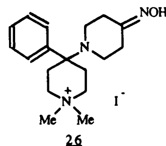
1-(1'-Dimethyl-4'-phenylpiperidinal) piperidoneoxime iodide
