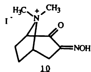
(±)-3-Oximino-tropan-2-one methiodide
