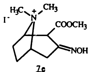
2-Carbomethoxy-3-oximino tropane methiodide
