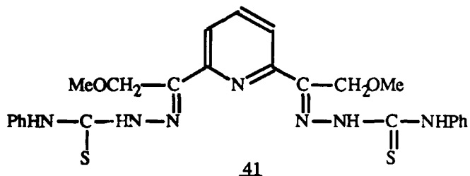
2,6-bis(Methoxymethylcarbonyl) pyridine bis-4'-phenylthiosemicarbazone
