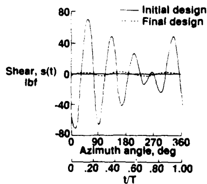
Fig. 7 Time history of vertical root shear minimized for 2 modes/3 harmonics.
