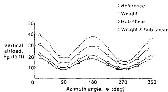
Fig. 11 Azimuthal distributions of vertical airload, 75% radius, \mu = 0.3 .
