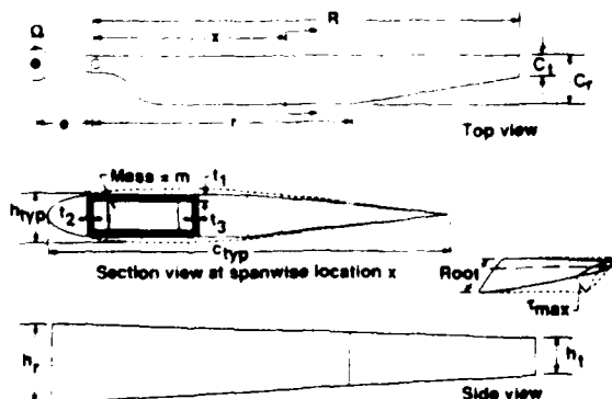
Fig. 3 Blade model and design variables.
