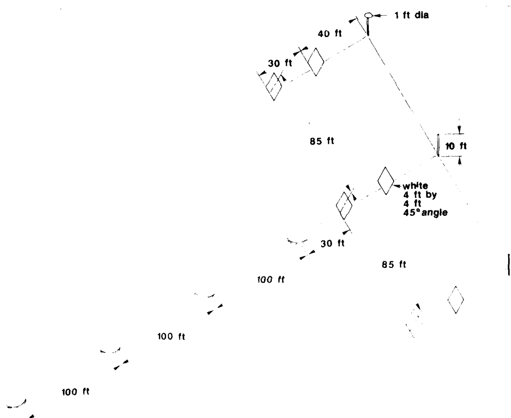
Figure 5. Schematic drawing of test field.
