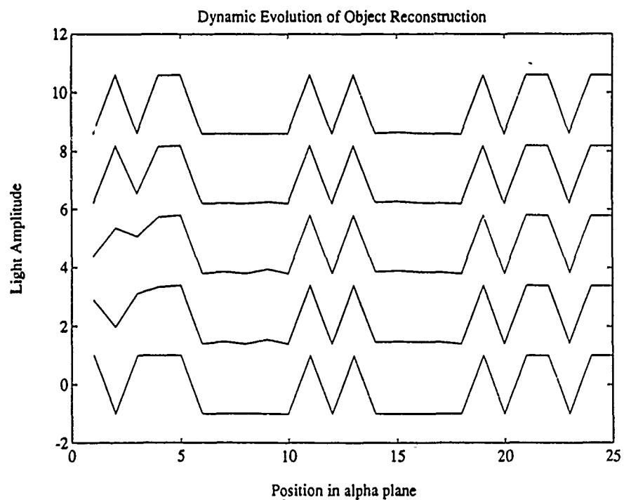
Figure D-6. Results of NHAM computer simulation. a. Evolution of \beta domain over five iterations showing convergence to a stored state. b. Corresponding evolution of \alpha domain.
