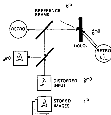
Fig. 1 Recording and readout of objects in reference-based NHAM
