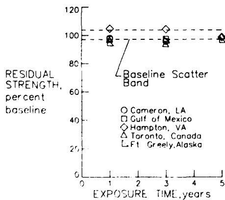
Figure 10 .-Effect of Exposure Location on the Residual Compression Strength of Kevlar-49/CE-306
