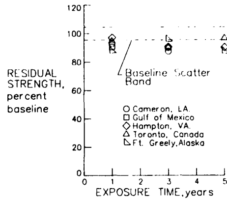
Figure 18.-Effect of Exposure Location on the Residual Short Beam Shear Strength of Kevlar-49/LRF-277
