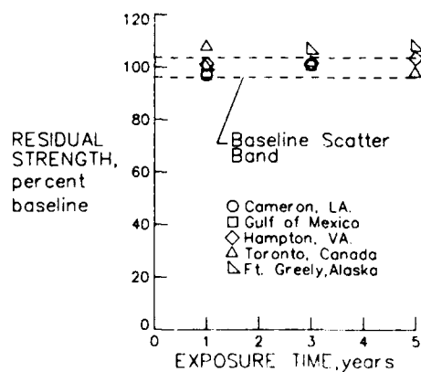
Figure 29 -Effect of Exposure Location on the Residual Tension Strength of T-300/E-788
