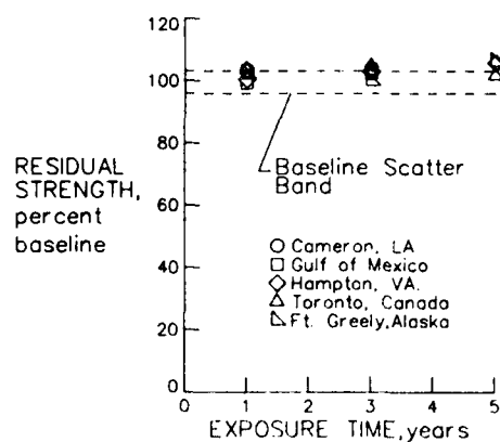
Figure 27 -Effect of Exposure Location on the Residual Tension Strength of Kevlar-49/LRF-277
