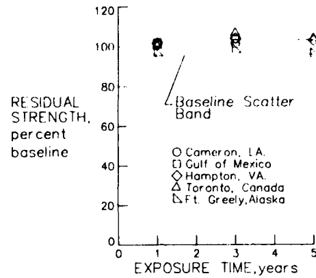
Figure 20.-Effect of Exposure Location on the Residual Short Beam Shear Strength of T-300/E-788
