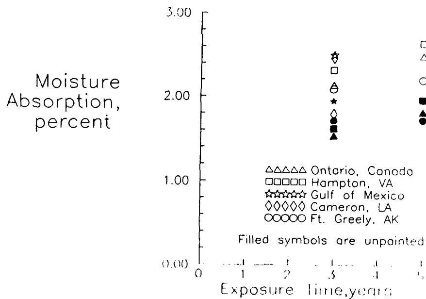
Figure 32. - Moisture absorption of Kevlar-49/E-185 Composite Material
