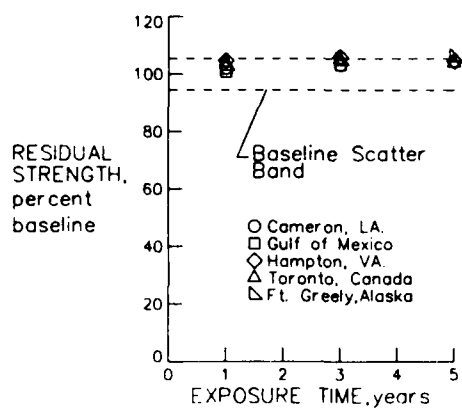
Figure 26 -Effect of Exposure Location on the Residual Tension Strength of Kevlar-49/F-185
