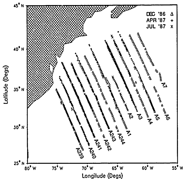
Fig. 1. Chart of the northwest Atlantic showing locations of AXBTs, dropped along Geosat ERM ground tracks, used in this study. Geosat ERM ascending ground tracks are labeled from A1 through A244, beginning with the track over Bermuda and increasing toward the east.
