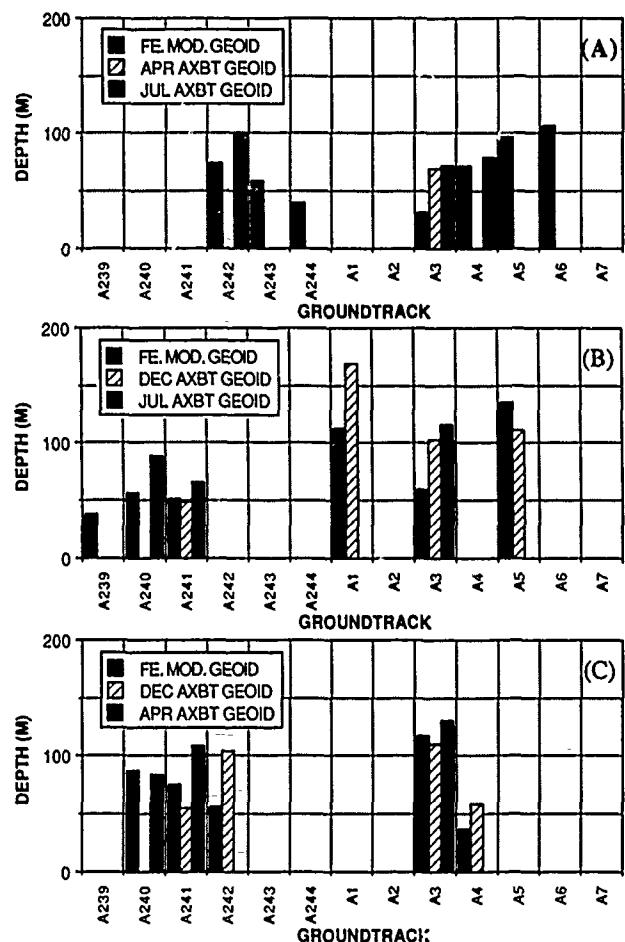
Fig. 15. Histograms of the root-mean-square 15°C isotherm depth difference, \text{rms}[X_{15} - S_{15}(d_A)] , between AXBT profiles and synthetic temperature profiles, where synthetic profiles were computed based on the surface heights ( d_A ) derived from the altimeter. Each rms value computed using all AXBTs and corresponding altimeter-derived synthetic profiles at the AXBT positions along a given Geosat ERM groundtrack and for a given AXBT survey period: (a) December 1986, (b) April 1987, (c) July 1987. Surface heights computed from the altimeter data employed (cases as indicated on graphs) one or more of the geoid height estimates defined in the text as the feature-modeled geoid and the December, April, and July AXBT geoids.
