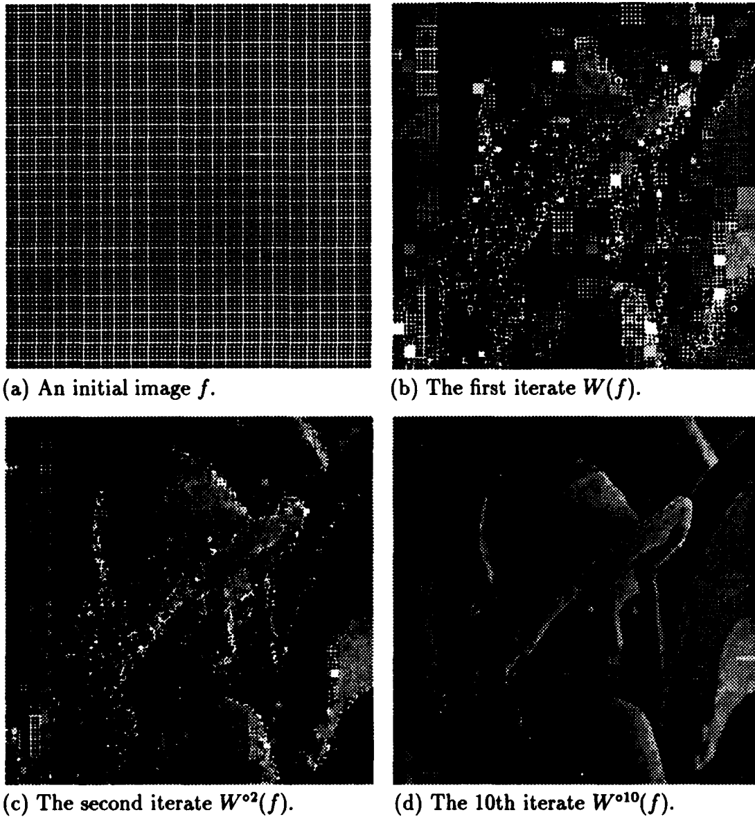
Figure 11. Decoding process for Lena.
