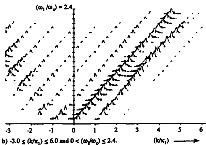
Fig. 12. Repeats Fig. 10a with a change in the wavenumber-frequency range displayed from the standard range -1.5 \leq (k/k_1) \leq 3.0 and 0 < (\omega/\omega_0) \leq 0.6 to the values noted.
