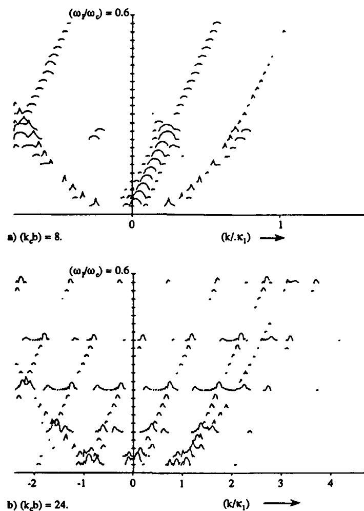
Fig. 7. Magnitude of the reflection coefficient \overline{R}_s^{-1}(kl/k_1) for the proper model [Eq. (42a)] as a function of the normalized wavenumber (k/k_1) in the standard format and under standard conditions with the exception that instead of the standard value of (k_c b) = 16 , the value is as noted.
