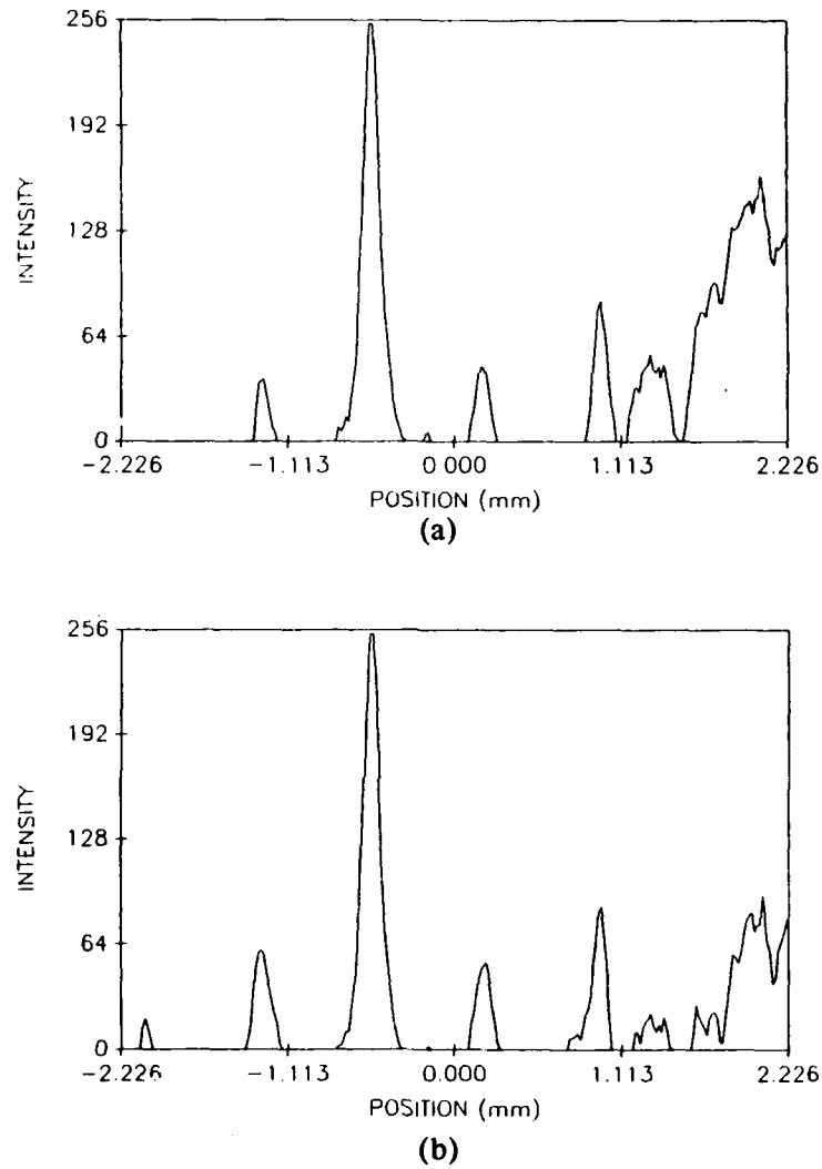
Fig. 14 — Magnitude of normalized correlation coefficient, |\mu_A|^2 computed by Fourier technique for (a) unenhanced and (b) enhanced experimentally recorded speckle
