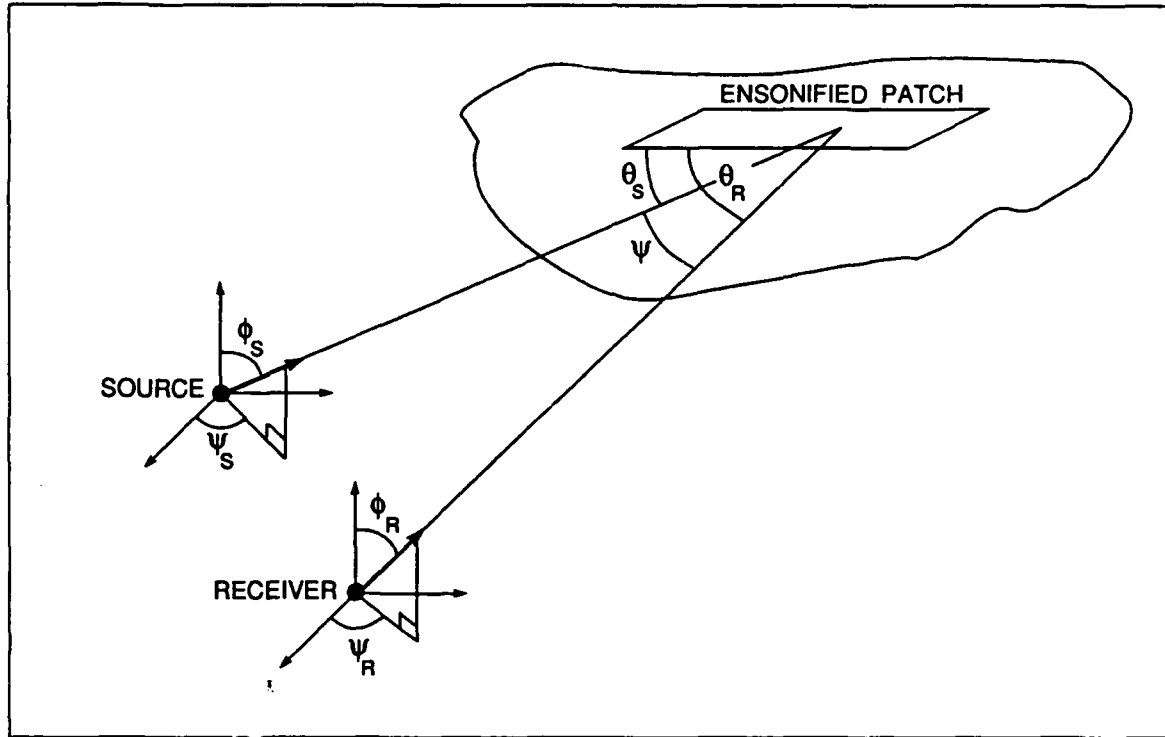
Fig. 1 - Short-range geometry
