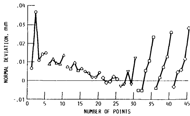
FIGURE 6. - PLOT OF DEVIATION OF REAL SURFACE \Sigma_r .
