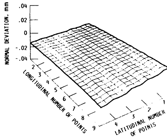
FIGURE 9. - DEVIATION OF FITTED IMAGE SURFACE \Sigma_f .
