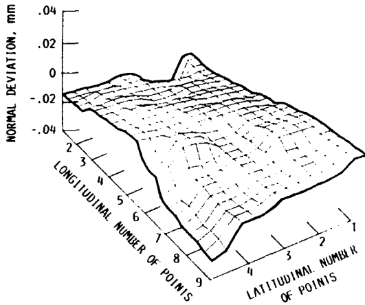
FIGURE 7. - DEVIATION OF IMAGE SURFACE \Sigma_r^* .
