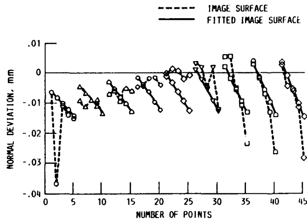
FIGURE 8. - PLOT OF DEVIATIONS OF IMAGE SURFACE \Sigma_r^* AND FITTED IMAGE SURFACE \Sigma_f .
