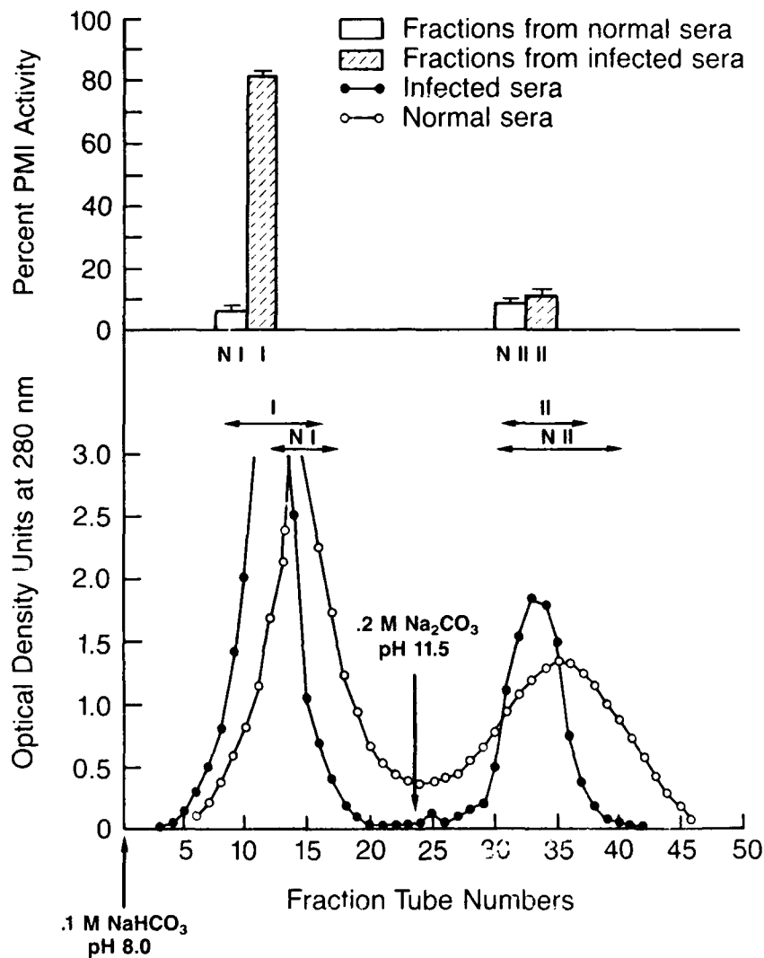
Figure 6. Elution profile from immunoaffinity chromatography of peak F from Sephadex G-200 column. Second peak which eluted at a high pH failed to induce PMIF response. However, it had antibody activity to E. canis (mean % \pm SE).
