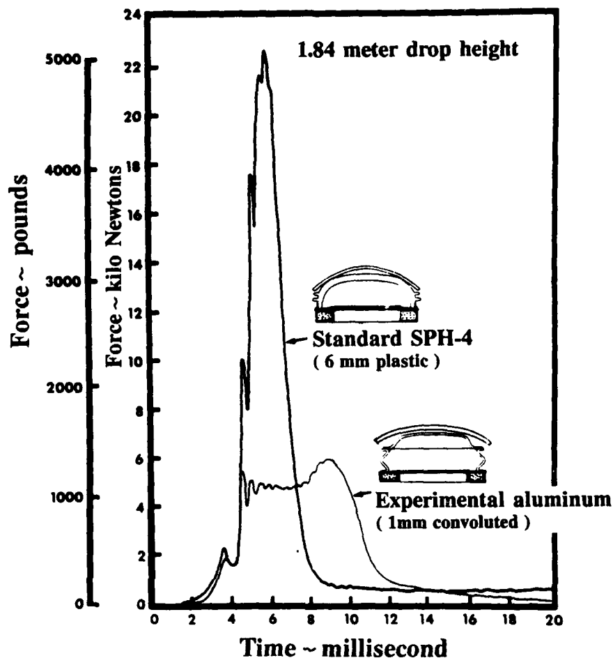
Figure 10. Comparison of force transmitted to standard SPH-4 earcup and a crushable earcup
