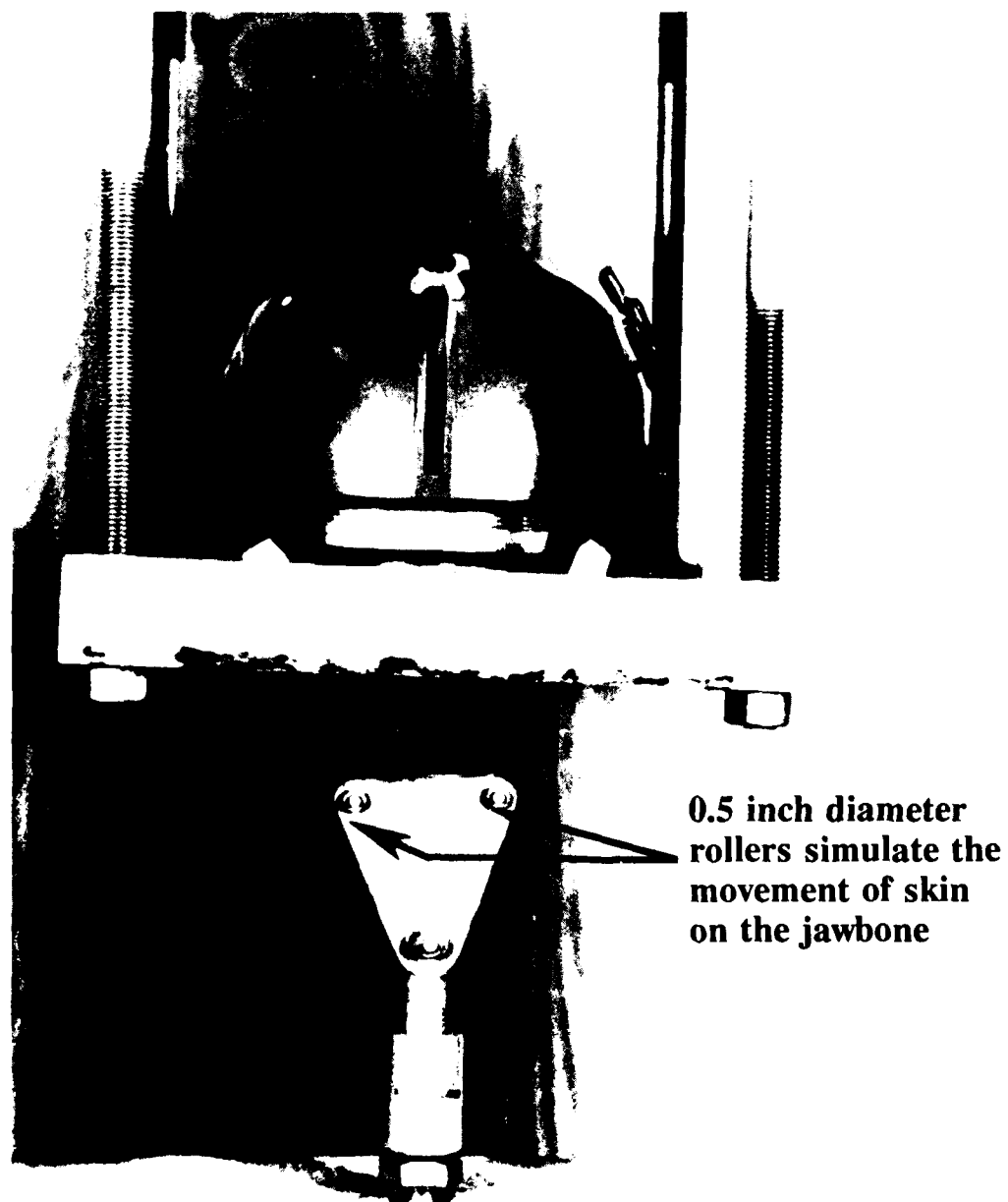
Figure 12. USAARL chinstrap test device.
