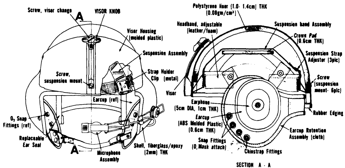
Figure 2. SPH-4 helmet assembly.
