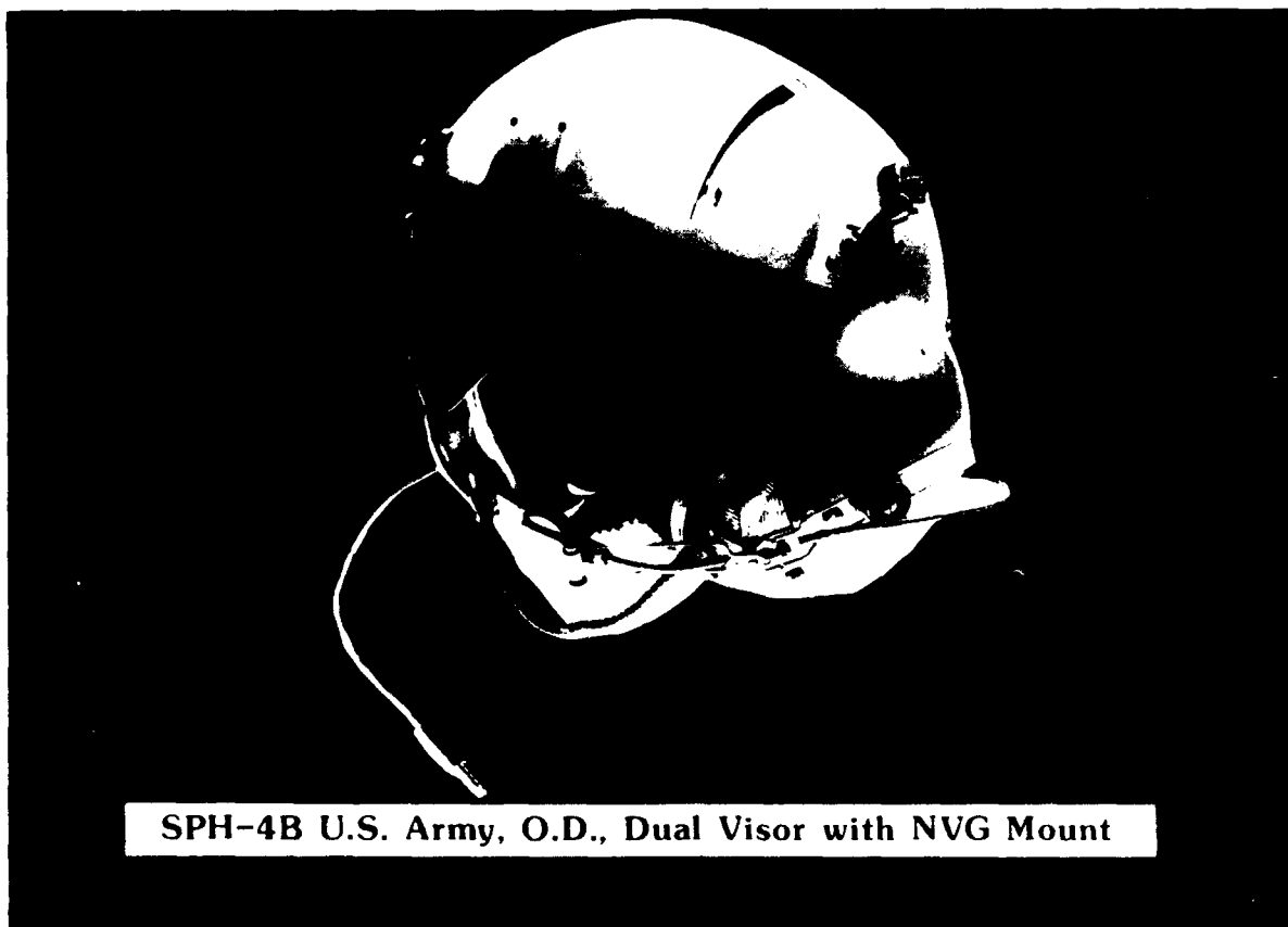
Figure 4. SPH-4B helmet (courtesy Gentex Corporation).
