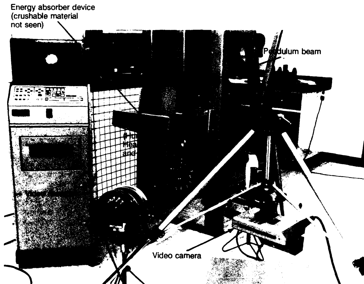
Figure 13. Pendulum device and high-speed video recorder.
