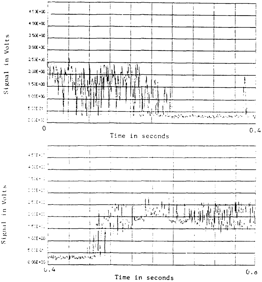
Fig. 7 Return signal as a function of time for the run with probability distribution shown in Fig. 8. The zero is offset vertically by about 0.3 volts in this figure, permitting display of the noise when zero signal is present.
