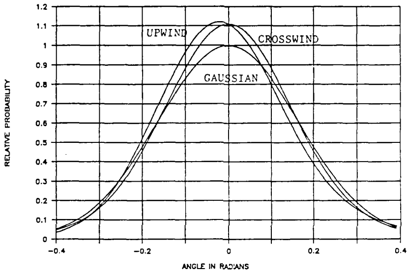
Fig. 14 Gram-Charlier distribution for wind speed of 10 m/sec.
