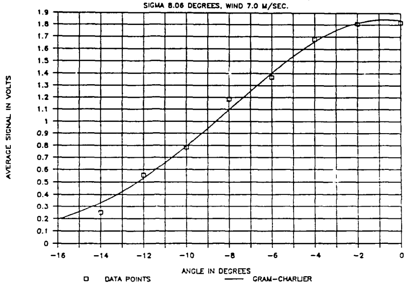
Fig. 15 Gram-Charlier upwind function fitted to the average signal values for the scan set that includes the curves of Figs. 8 to 10.
