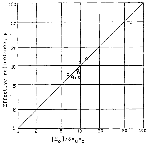
Fig. 16 Observed effective reflectance, \rho , plotted as a function of [H_o]/8\sigma_u\sigma_c
