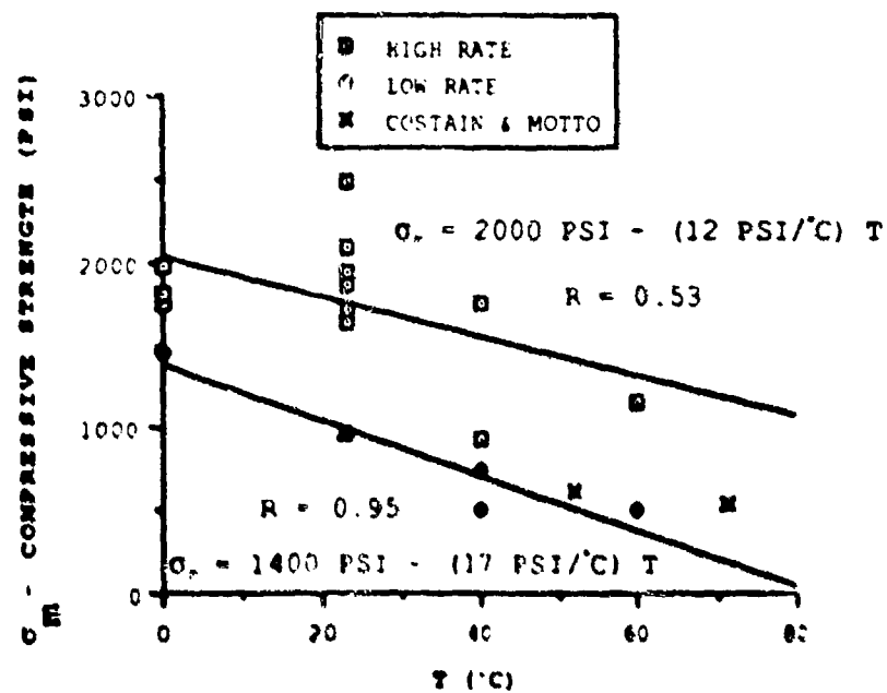
Figure 8. Compressive strength, \sigma_m , versus temperature for TNT for the low and high strain rates. Also shown are points from the work of Costain and Molto (ref 8).
