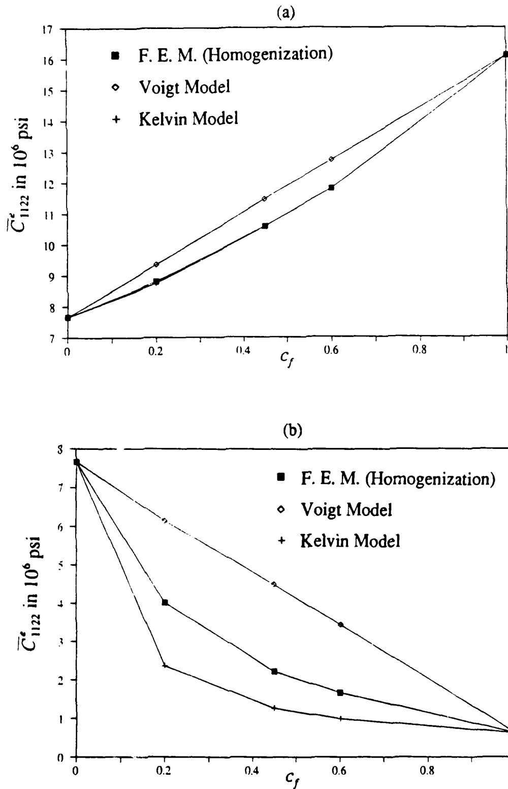
Fig. 4. Variation of the composite elastic moduli \bar{C}_{112}^* with fiber volume fraction c_f . (a) and (b), respectively, represent the results for the B/Al and Gr/Al.
