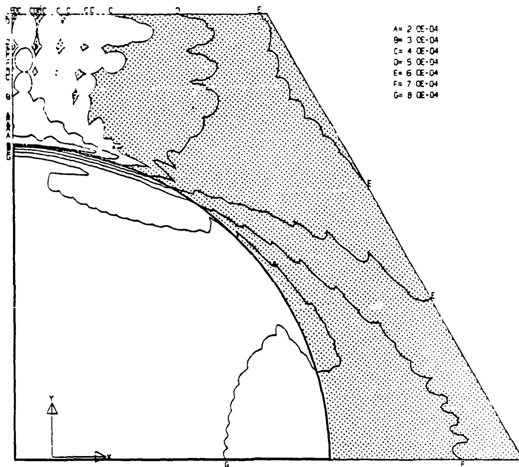
Fig.17. Contour of equivalent stress \bar{\sigma} in B/A1 at 15th step. c_f = 45\% , n = 5 , \beta = 0.5 , and \chi = 0.0 . The dotted region represents the plastic zone.
