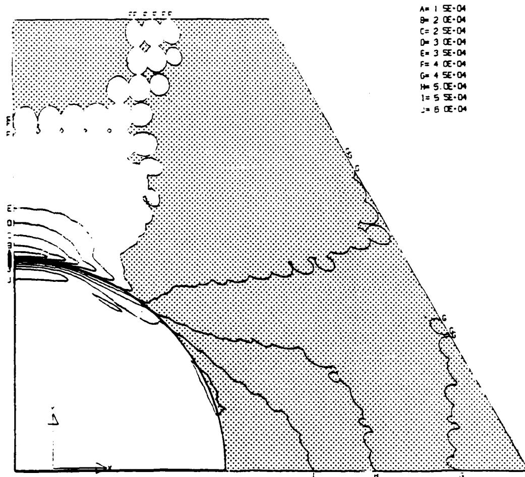
Fig.14. Contour of equivalent stress \bar{\sigma} in B/Al at 5th step. c_f = 20\% , n = 5 , \beta = 0.5 , and \chi = 0.0 . The dotted region represents the plastic zone.
