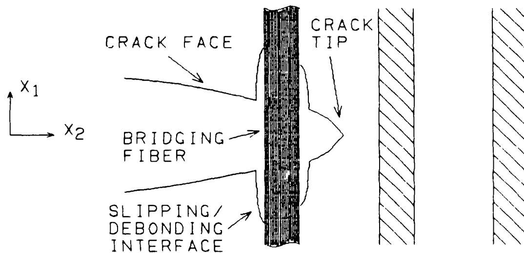
Figure 1.2a. Idealized initial configuration of a propagating crack in a unidirectional fiber reinforced ceramic. The crack front is straight and lies between bridged and approached fibers.
