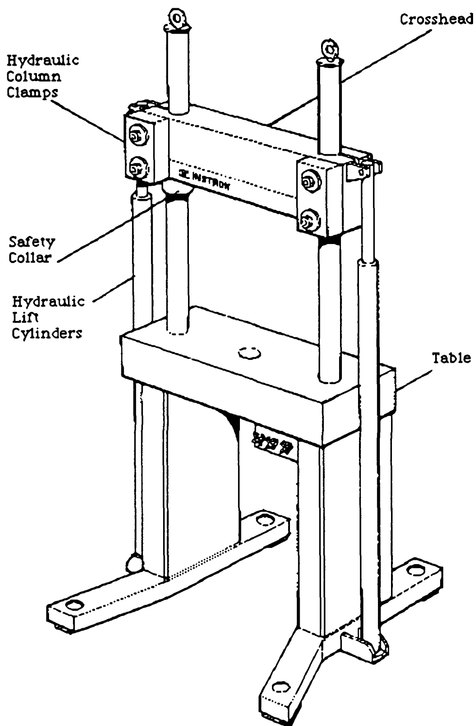
FIGURE 10: Schematic Diagram of the Mechanical Testing Machine.
