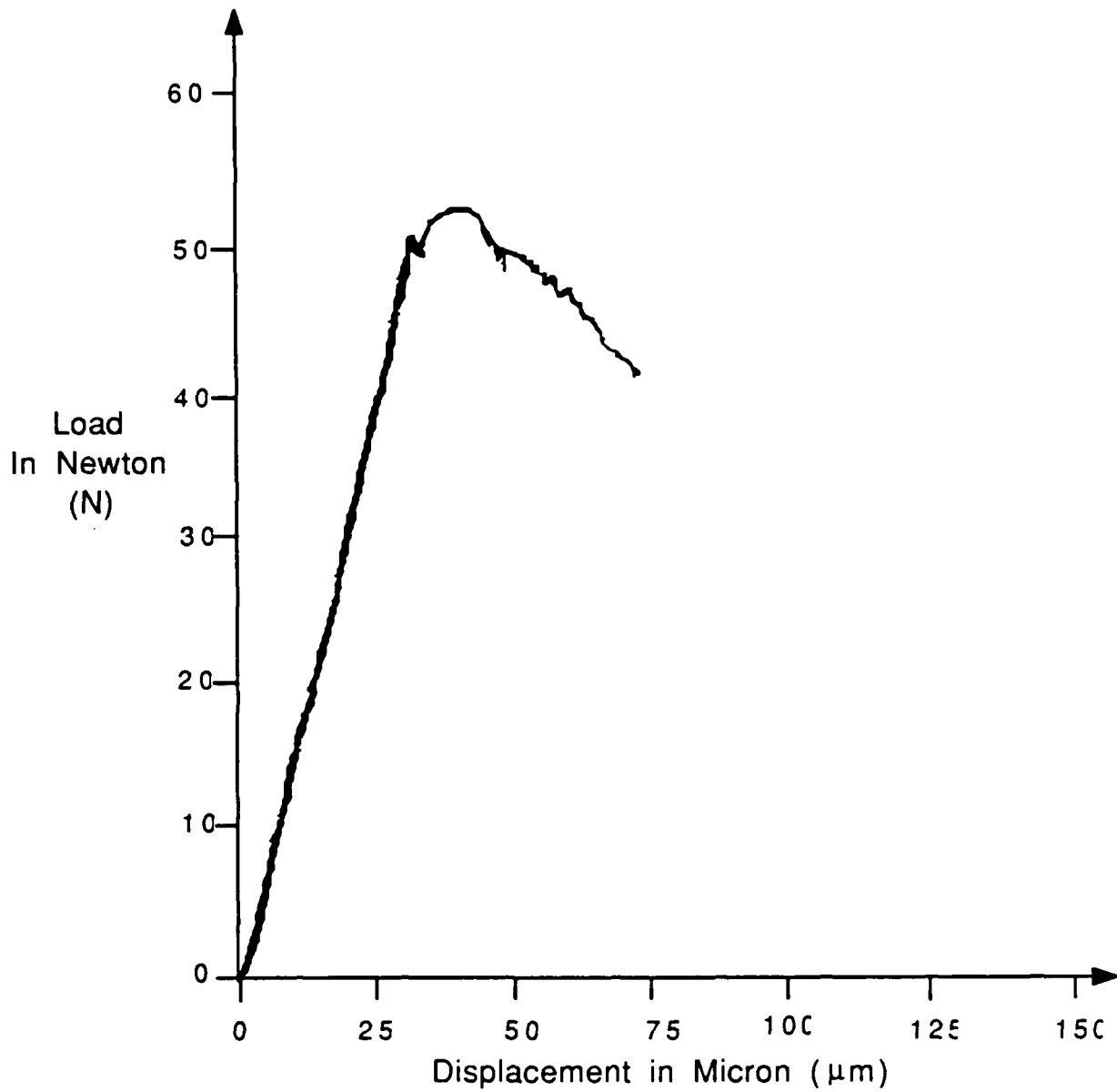
FIGURE A1: Load-Displacement Curve for 15 Vol.% Tateho SiC Whisker/Aluminum Oxide Matrix Composite at Room Temperature with an Angle of 69.44 Degree at the Base of the Chevron Notch.
