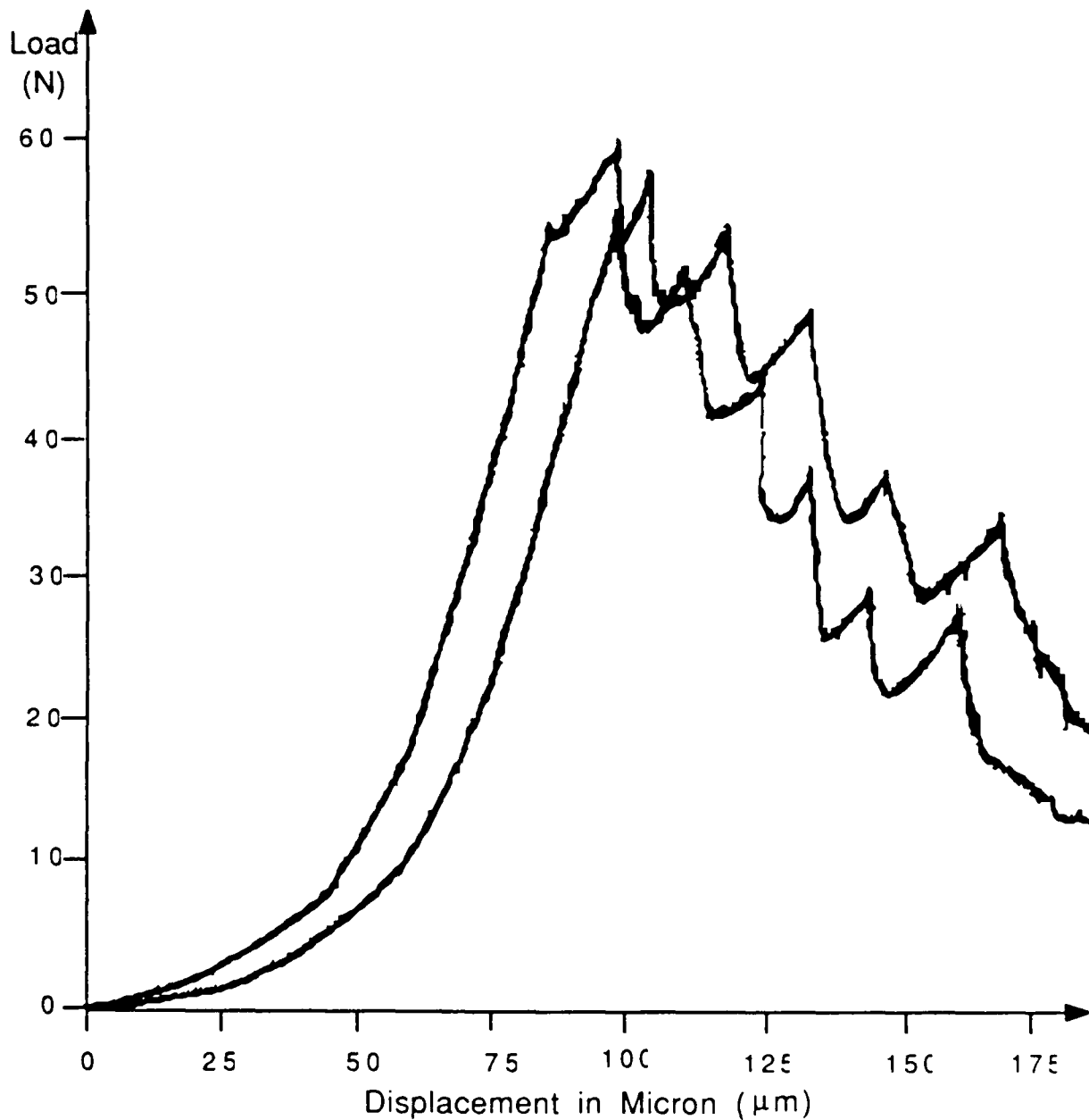
FIGURE A19: Load-Displacement Curves for 30 Vol.% Silar SiC Whisker/Aluminum Oxide Matrix Composite at High Temperature (1000 Degree Celsius) with an Angle of 45 Degree at the Base of the Chevron Notch.
