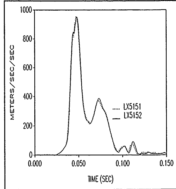
Figure 107. Resultant head linear acceleration (X-Z plane).
