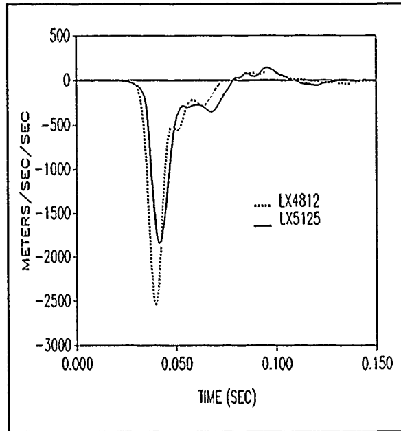
Figure 75. Head linear acceleration (X-component).
