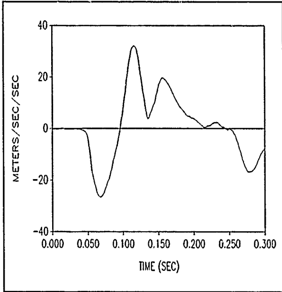
Figure 21. Head linear acceleration (Z-component) for 10 g, -X human, NFGD run.
