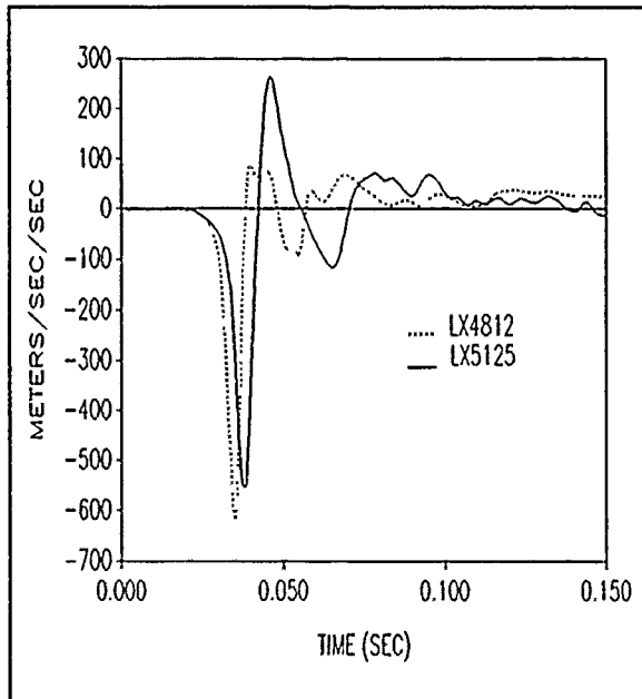
Figure 76. Head linear acceleration (Z-component).
