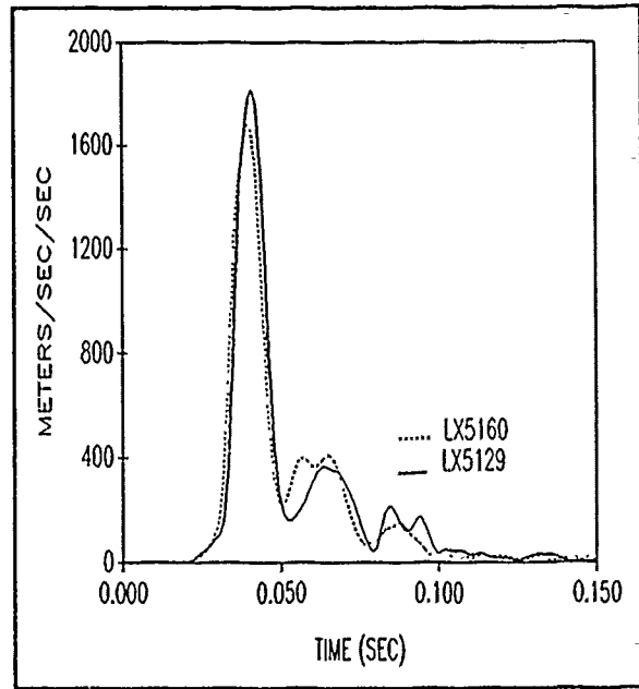
Figure 119. Resultant head linear acceleration (X-Z plane).
