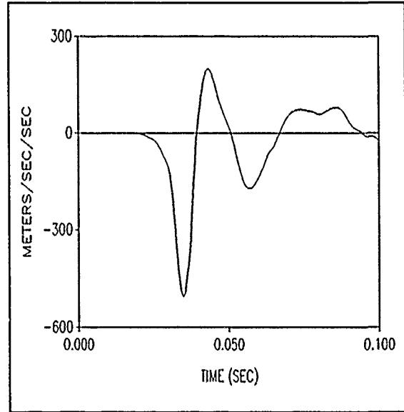
Figure 22. Head linear acceleration (Z-component) for 74 g, -X animal, NFGD run.
