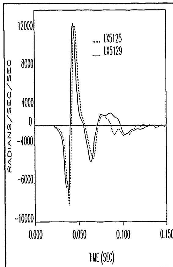
Figure 97. Head angular acceleration (Y-axis).
