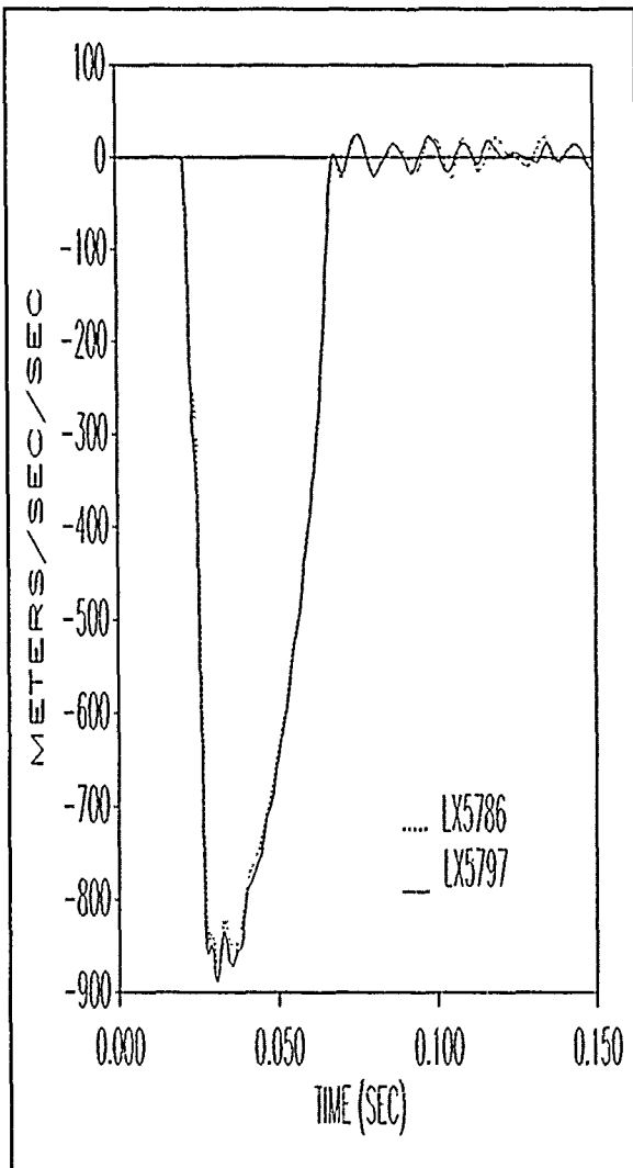
Figure 49. Sled acceleration profile.
