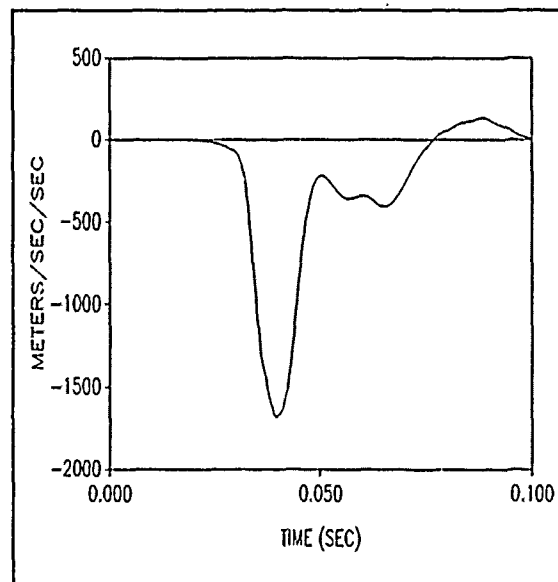
Figure 20. Head linear acceleration (X-component) for 74 g, -X animal, NFCD run.
