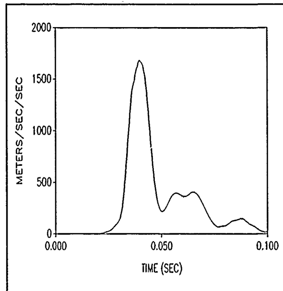
Figure 24. Resultant linear acceleration (X-Z plane) for 74 g, -X animal, NFGD run.
