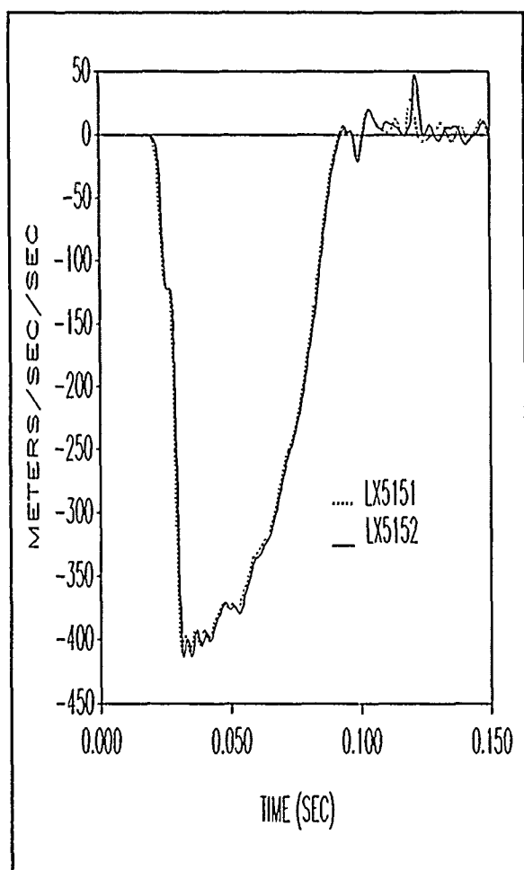
Figure 102. Sled acceleration profile.
