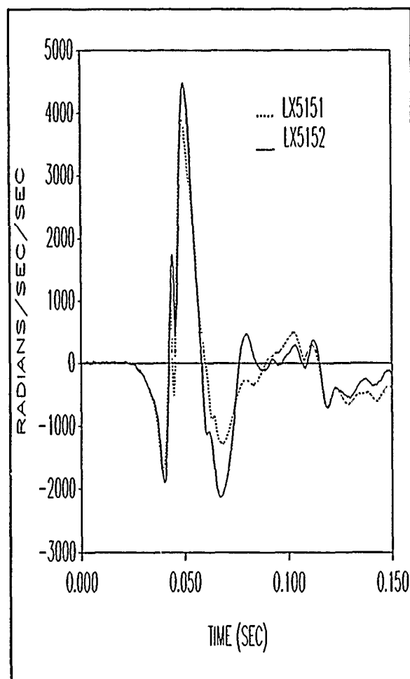
Figure 103. Head angular acceleration (Y-axis).
