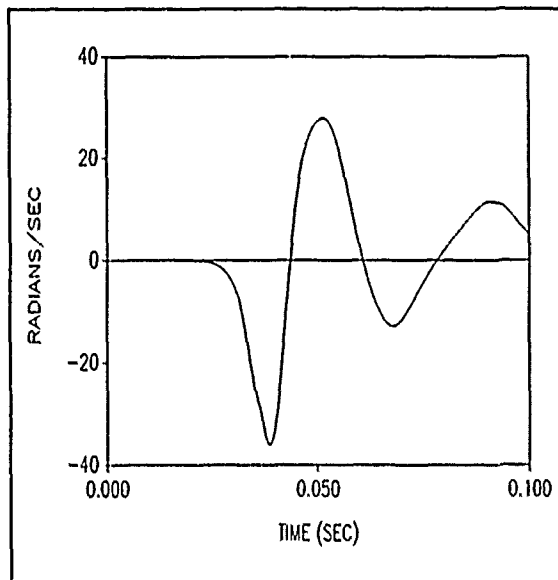
Figure 18. Head angular velocity (Y-axis) for 74 g, -X animal, NFCD run.
