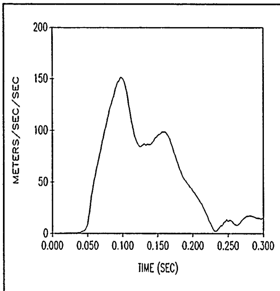
Figure 23. Resultant linear acceleration (X-Z plane) for 10 g, -X human, NFGD run.
