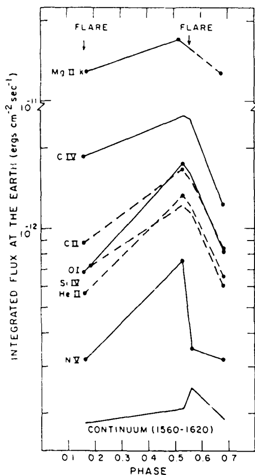
FIG. 5—The integrated emission-line fluxes of various lines received at Earth from HR 5110 as a function of phase. All lines (except Mg II) vary in unison by roughly the same factor with maximum emission occurring at phase 0.52.
