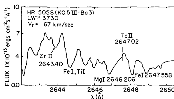
FIG. 1. The 2647 Å region of HR 5058 (LWP 3730). Several photospheric absorption lines are indicated, as well as the position of the Tc II line at 2647.02 Å. The radial velocity for the star is +67 km/s.
