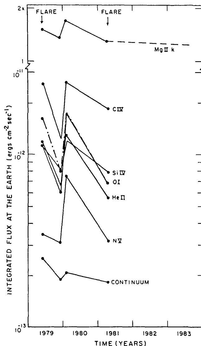
FIG. 3.—The integrated UV emission line flux received at Earth from HR 5110 as a function of time. The occurrences of the two radio flares are indicated with arrows. The continuum flux is the average flux measured in the region 1560-1620 Å.
