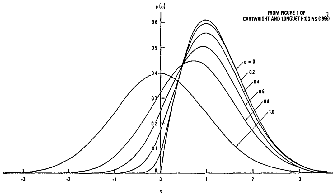
Fig. 7 Probability distribution of the heights of maxima for different values of the width \epsilon of the energy spectrum
