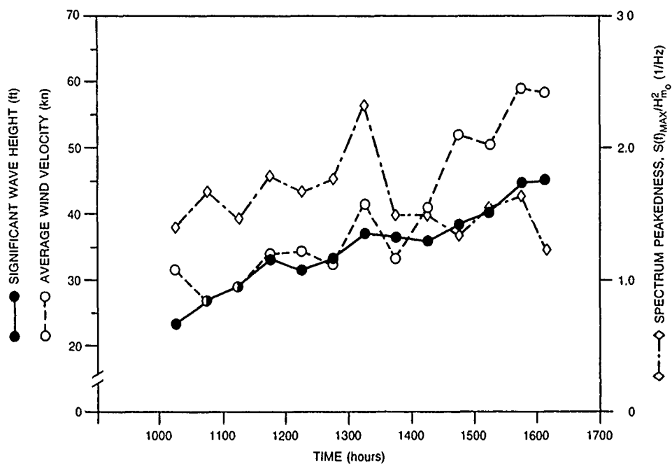
Fig. 15. Significant Wave Height, Average Wind Velocity and Spectrum Peakedness vs. Time During Hurricane Camille (1000-1618 hours).
