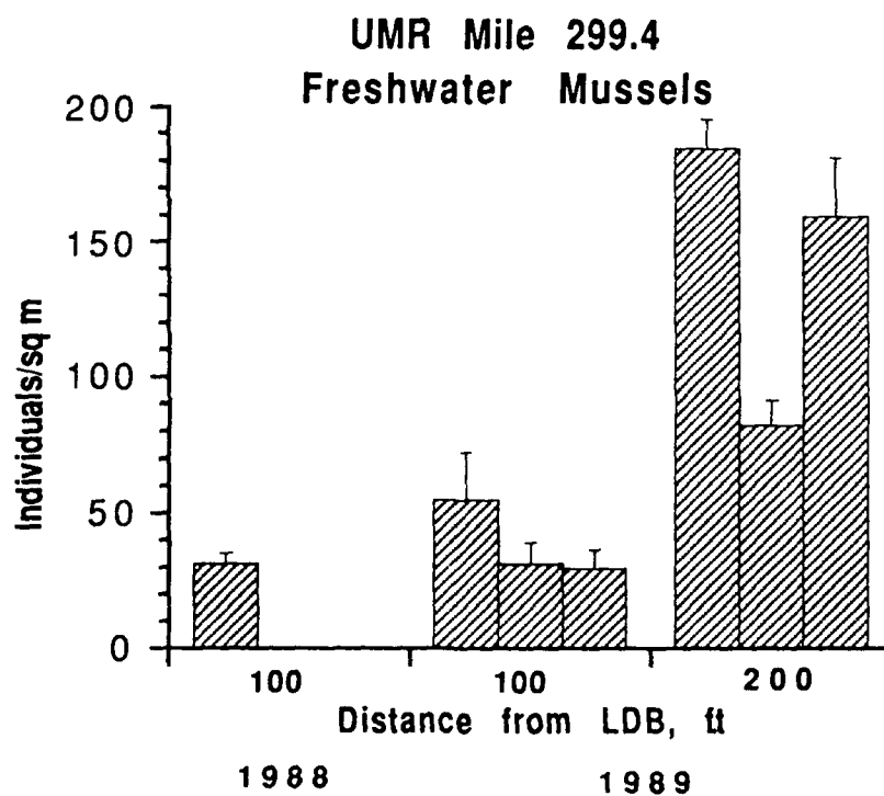
Figure 14. Total density of mussels in 1988 and 1989
