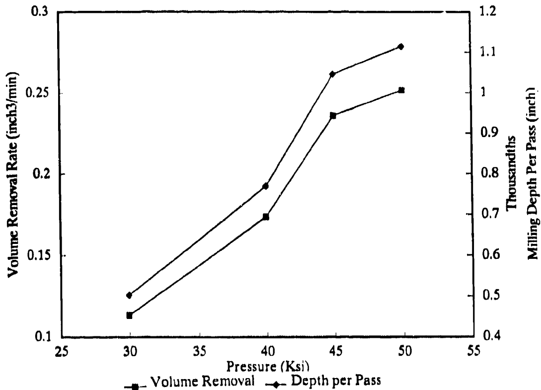
Figure 25. Effect of Pressure on Volume Removal Rate and Milling Depth Per Pass. d_m = 0.047 inch, l_m = 3 inches, d_n = 0.013 inch, gs mesh 100, m_a = 0.53 lb/min, n = 10.96 rps, inc = 0.6 , u = 6.18 in/min (see appendix test numbers 26, 31-33)
