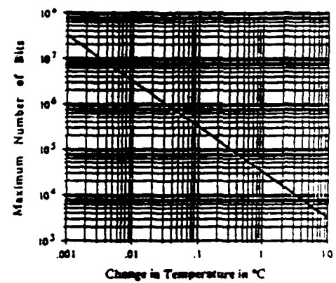
Fig. 3. Maximum number of bits b_{max} as a function of temperature stability \Delta T for a lightly doped fiber operating at 1310 nm.
