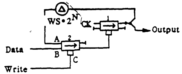
Figure 2a. Fiber Optic Delay Line Memory
