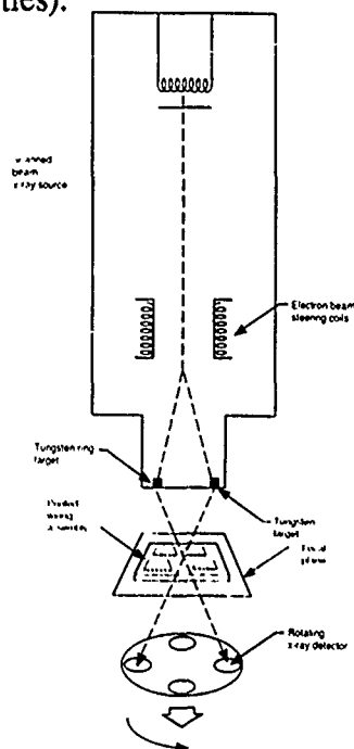
Figure A3-1 Scanned beam laminography
