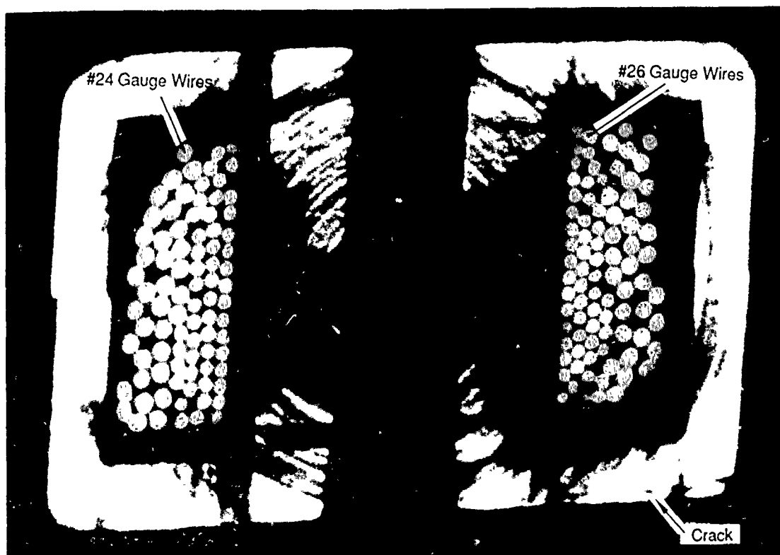
Figure 4.2-4 CT image of cracked core
