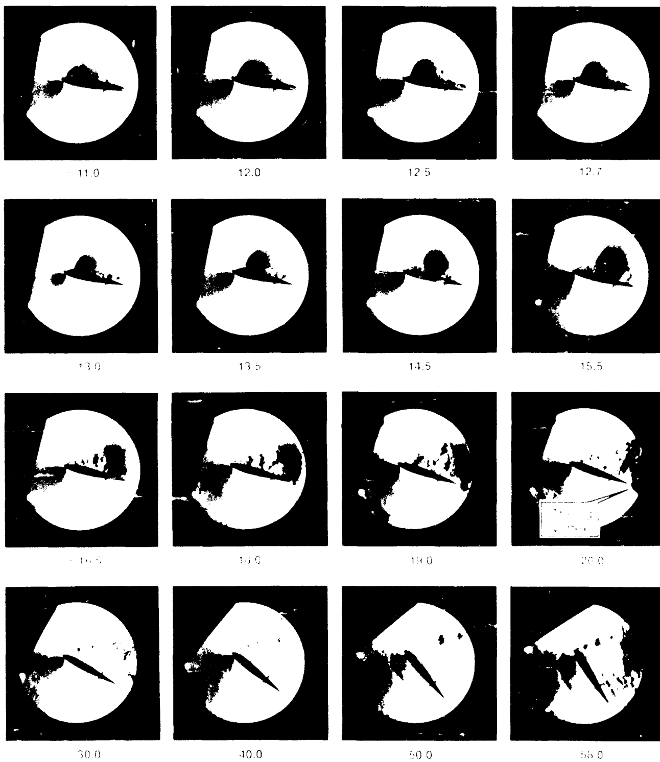
Fig. 5 Stereoscopic Schlieren Pictures of the Compressibility Effects on Dynamic Stall of a Rapidly Pitching Airfoil ( M_\infty = 0.45 , \alpha^* = 0.03 )
