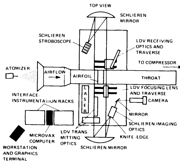
Fig. 3. Schematic of the CDSF Instrumentation.
