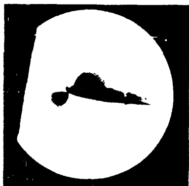
FIG. 12.3. A Solid-on Picture of a Shock on a Pitching Airfoil. M = 0.24 , \alpha = 0.4^\circ , \omega = 0.005 rad/sec, \omega t = 16.7^\circ .
