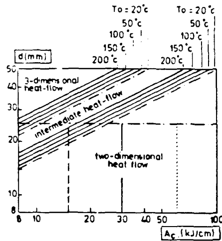
Fig.3.9(1). Charts for the determination of t_{8/5} . Type of heat-flow.
