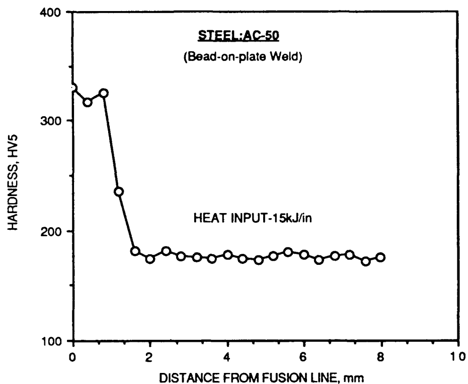
Fig. B-34. HAZ hardness profile. Steel : AC-50. Heat Input : 15 kJ/in
