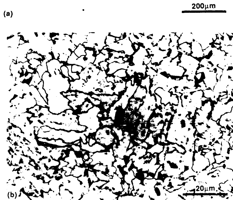
Fig. A-1.(a) Distribution of Inclusions, 100X, as-polished.
