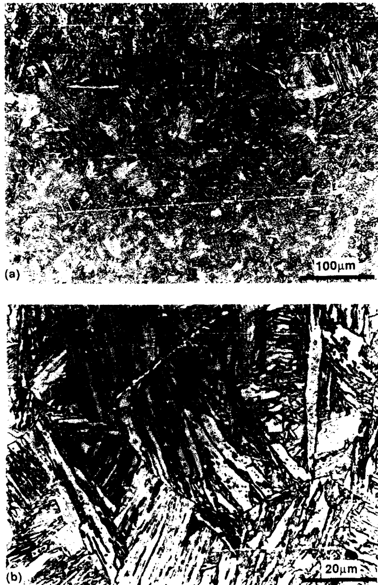
Fig. A-10. Microstructure of the coarse grained HAZ containing 100% martensite; (a) 200X, (b) 1000X.
