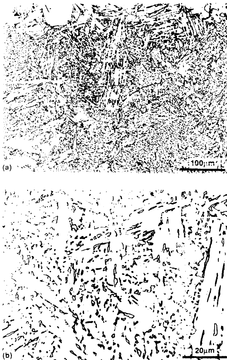
Fig. A-8 Microstructure of the fully bainitic coarse grained HAZ; (a) 200X, (b) 1000X.
