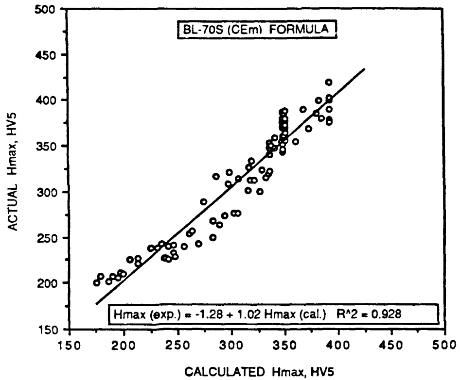
Fig.3.34. Comparison between experimental and calculated maximum HAZ hardness from BL-70S (CE m ) for all steels.
