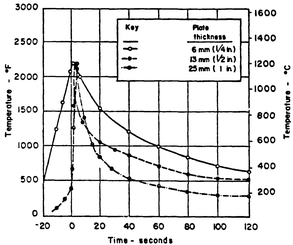
Fig.3.6. Effect of plate thickness on the thermal cycles in the weld HAZ of SMA welds in steel plate [25] Energy Input: 47 kJ/in. Initial plate temperature: 80°F.
