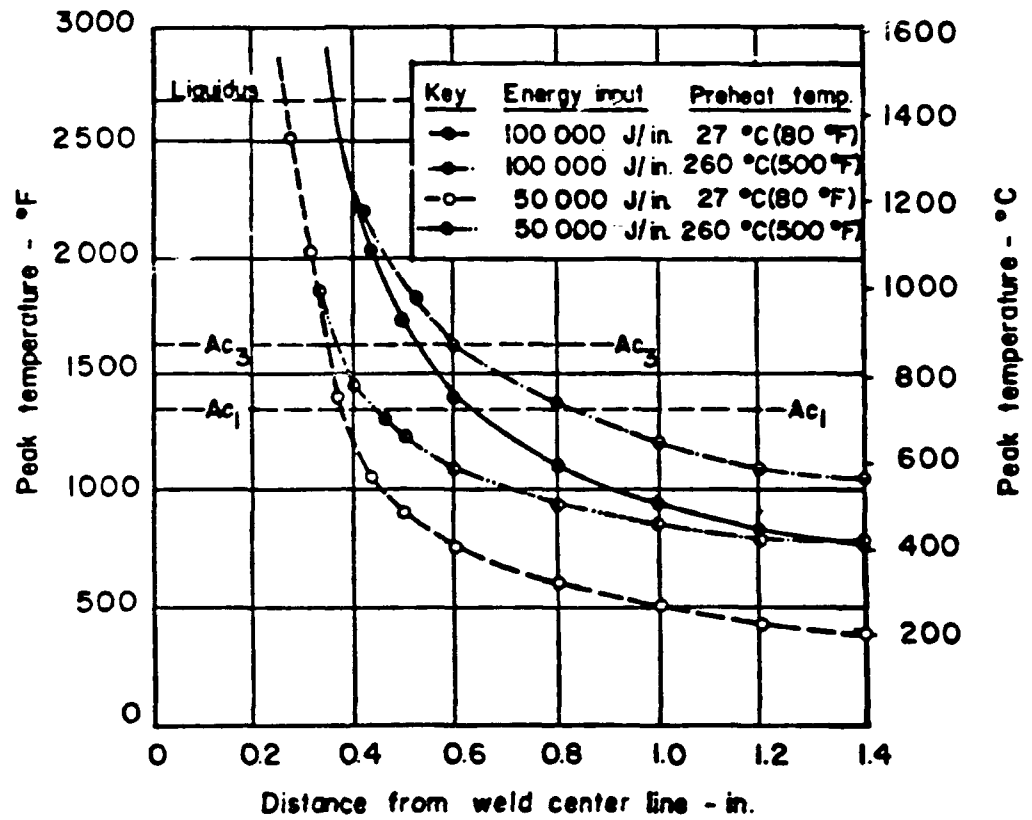
Fig.3.1. Effect of energy input and preheat temperature on peak temperature distribution. [25]
