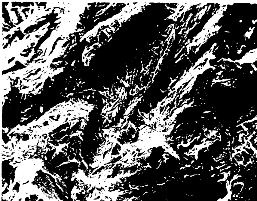
Fig.4.38. Quasi-cleavage mode of fracture in the hydrogen embrittled HAZ of HSLA-80-2; 500X
