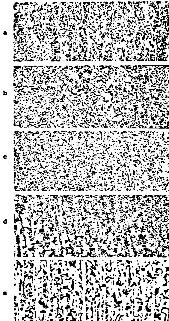
Fig.3.2. (a) Fusion zone (b) CGHAZ (c) FGHAZ (d) ICHAZ (e) Unaffected base metal [22]
