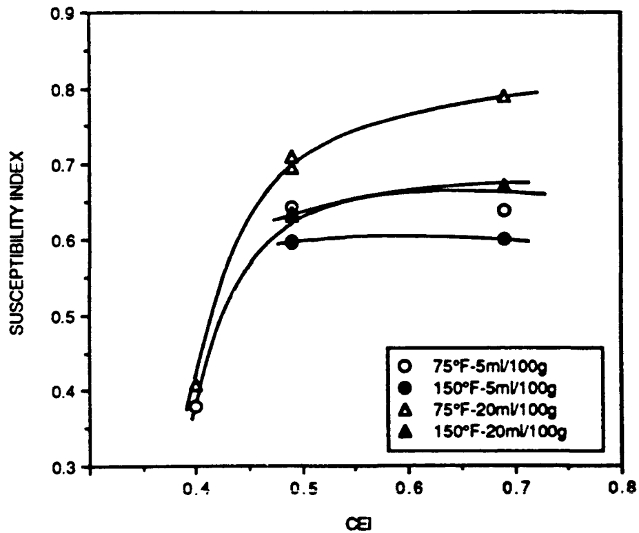
Fig.4.61. Variation of susceptibility index with P_{cm} for lower strength level steels
