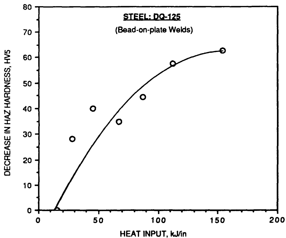
Fig. B-33. Variation of decrease in HAZ hardness with heat input for DQ-125
