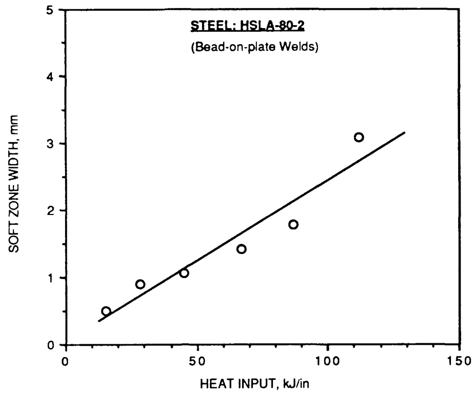
Fig. B-15. Variation of soft zone width with heat input for HSLA-80-2
