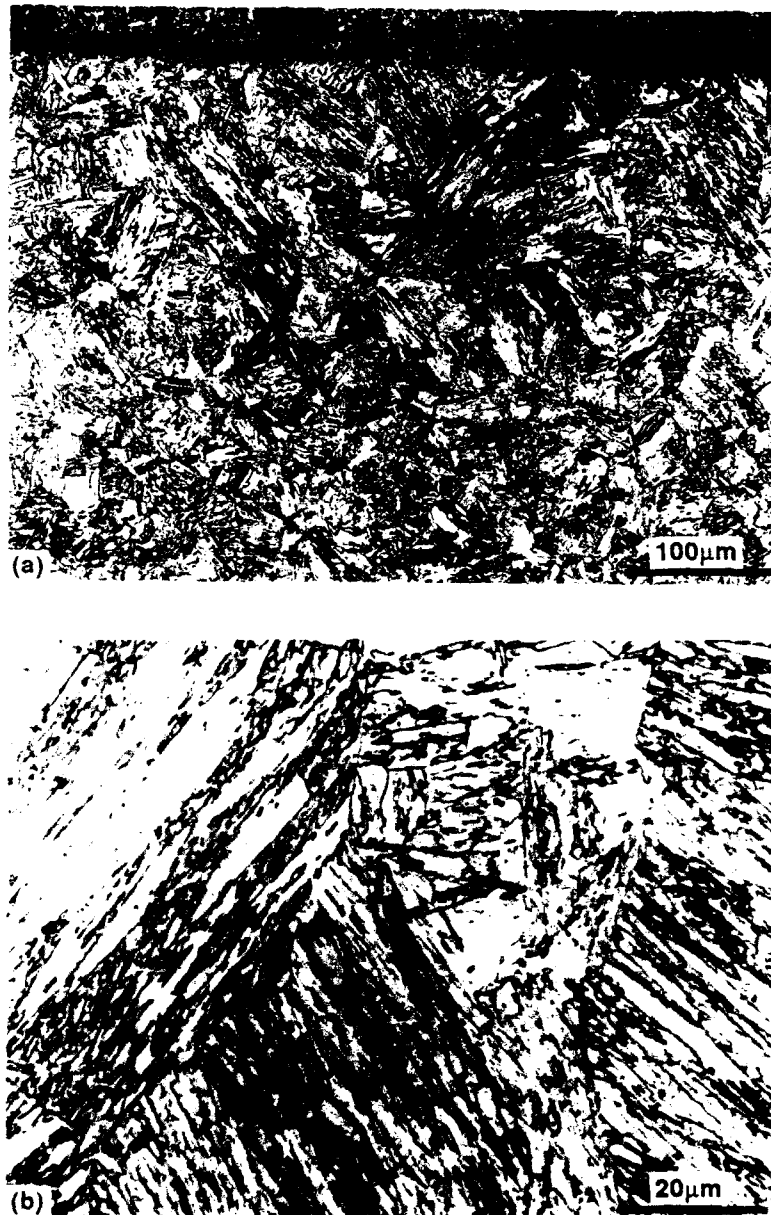
Fig. A-22. Microstructure of the fully martensitic coarse grained HAZ; (a) 200X, (b) 1000X.
