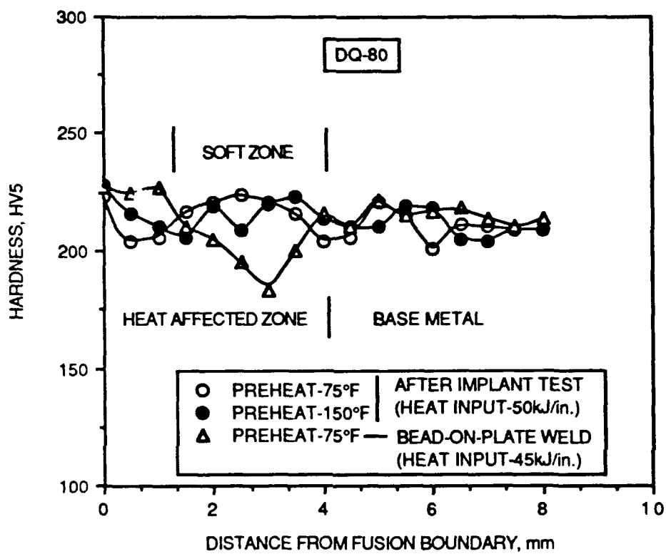
Fig.4.35. HAZ hardness profile in the as-welded bead-on-plate sample and implant samples after testing at 75 and 150°F preheat temperature
