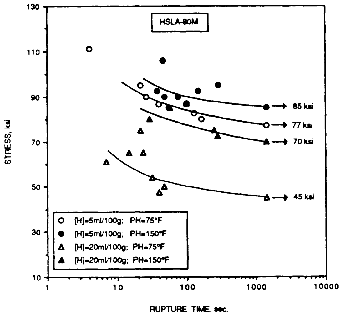
Fig.4.28. Implant cracking test results for HSLA-80M
