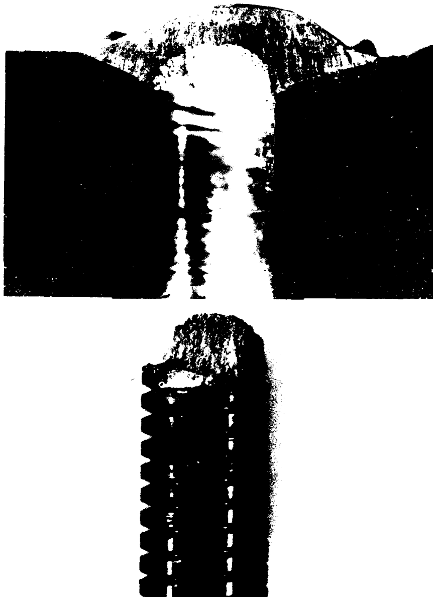
Fig.4.36. Cross-sectional view of an implant sample after rupture; HSLA-80-2; Stress-95ksi; Preheat temp. 75°F; 5X
