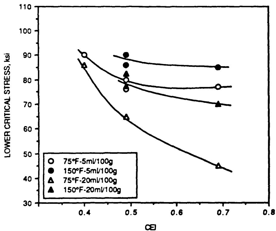
Fig.4.58. Variation of lower critical stress with CEI for lower strength level steels
