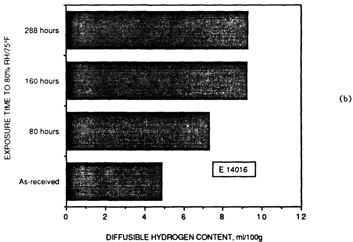
Fig.4.24. Increase in the diffusible hydrogen content with exposure time to controlled humidity environment for (a) E11018M and (b) E14016 electrodes
