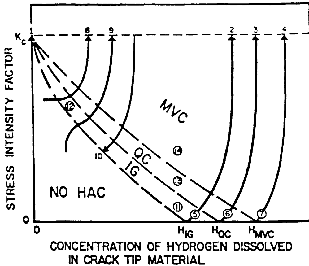
Fig.4.40. Interrelationship between stress intensity factor, diffusible hydrogen content and failure mode (Beachem diagram) [66]
