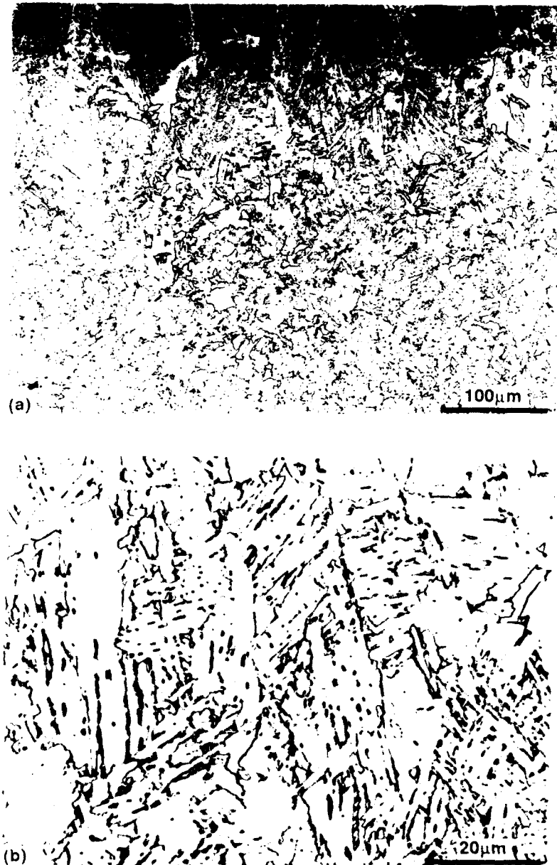
Fig. A-30. Microstructure of the coarse grained HAZ containing bainite and martensite; (a) 200X, (b) 1000X.
