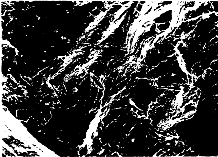
Fig.4.42. Quasi-cleavage mode of rupture observed in DQ-80 when tested at 5ml/100gm hydrogen level; 500X
