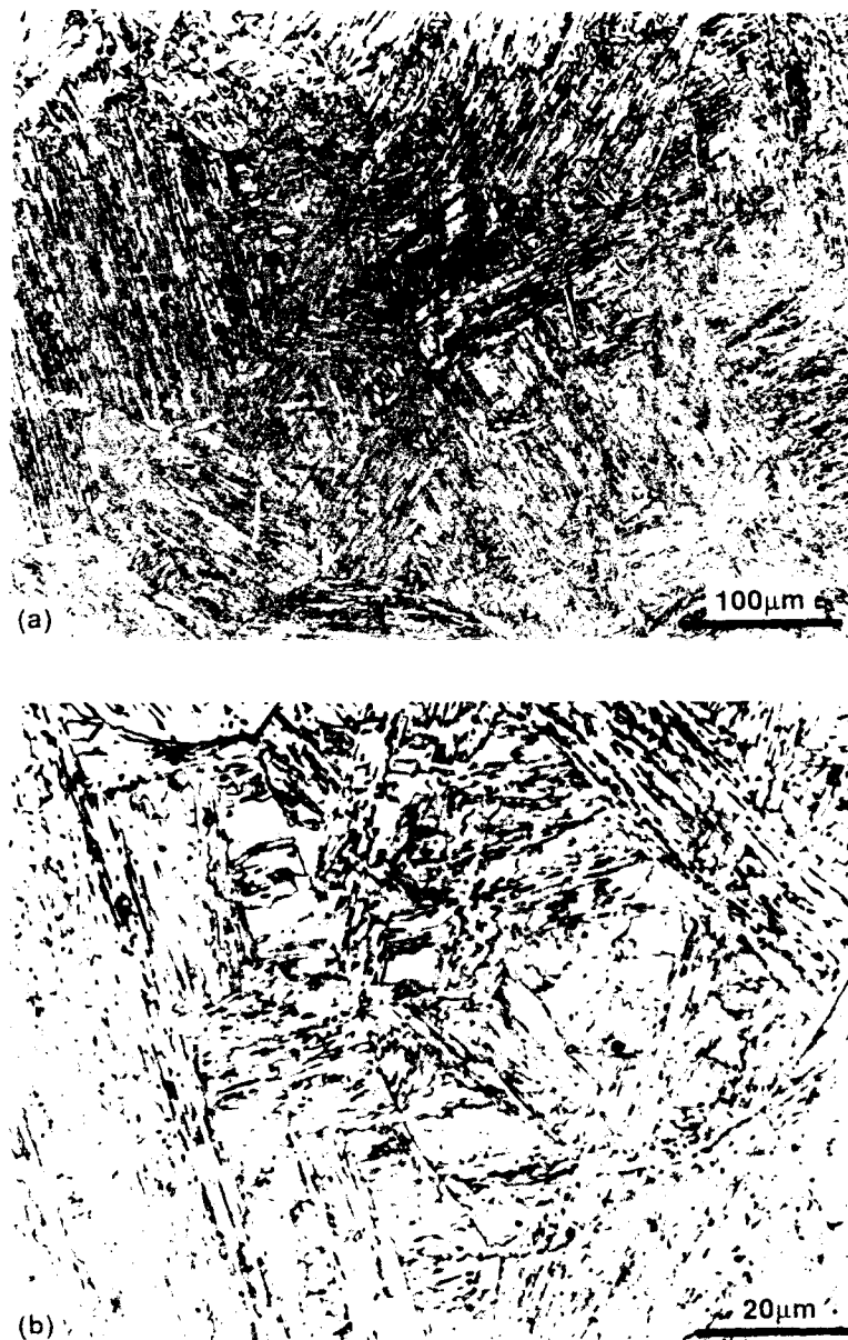
Fig. A-24. Microstructure of the coarse grained HAZ containing predominant amount of martensite; (a) 200X, (b) 1000X.
