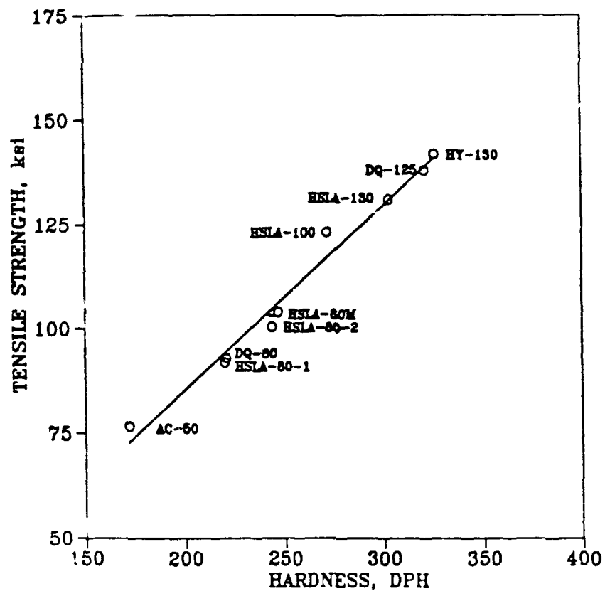
Fig.2.1. Variation of UTS with base metal hardness
