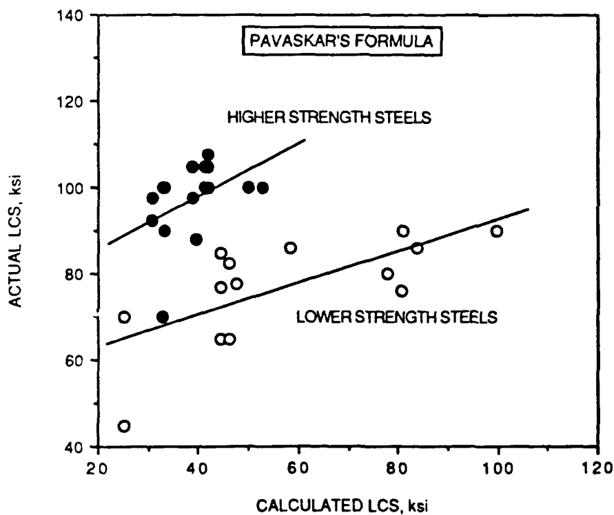
Fig.4.52. Comparison between actual and calculated lower critical stress by Pavaskar's formula for all steels
