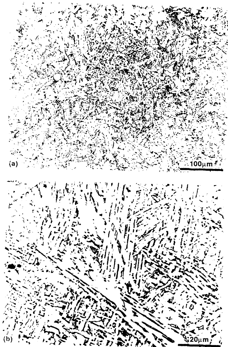
Fig. A-35. Microstructure of the coarse grained HAZ containing ferrite and small amount of martensite; (a) 200X, (b) 1000X.
