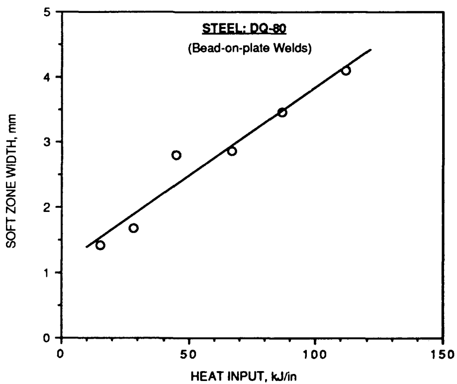
Fig. B-24. Variation of decrease in HAZ hardness with heat input for DQ-80
