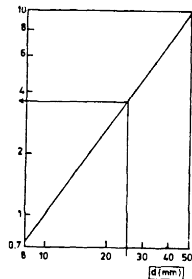
Fig.3.9(6). Charts for the determination of t_{8/5} . Two-dimensional heat-flow. Correction for thickness.
