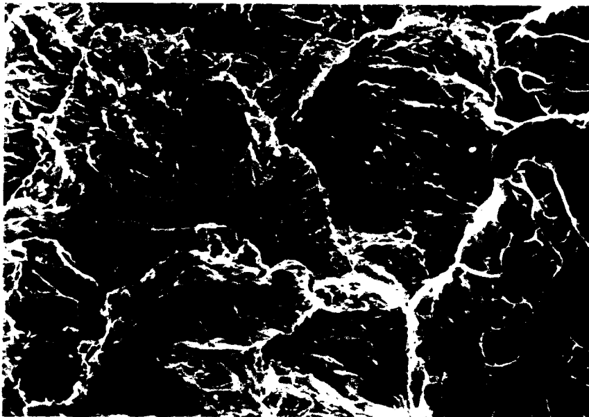
Fig.4.43. Quasi-cleavage with grain boundary decohesion in DQ-80 when tested at 20ml/100gm hydrogen level; 500X
