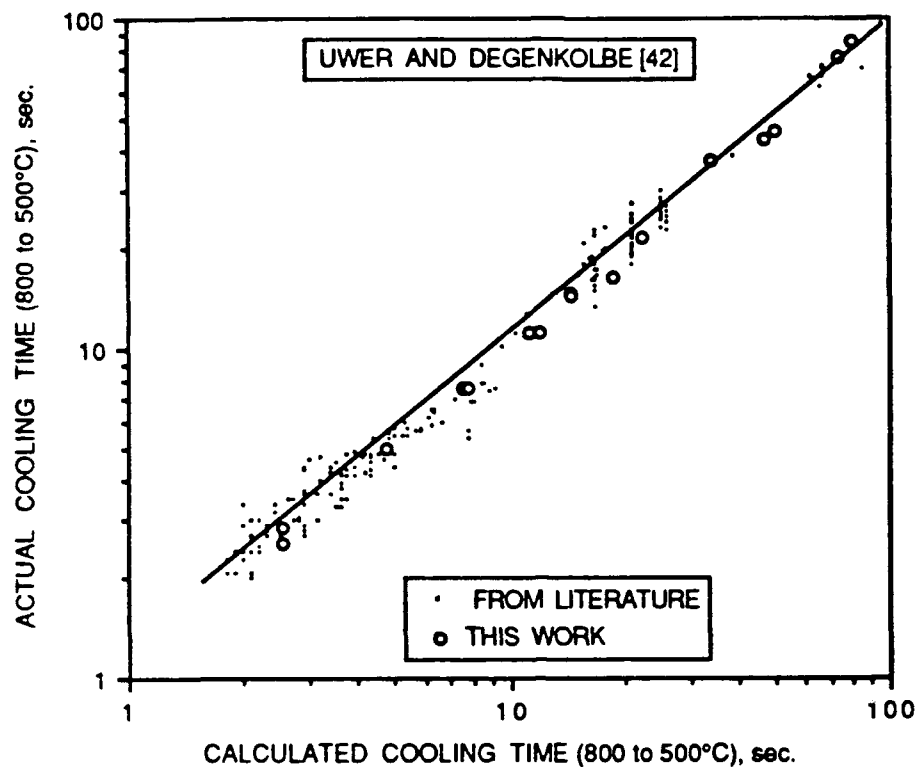
Fig.3.20. Comparison between the experimental (from this study and from literature) and calculated cooling time employing Uwer and Degankolbe equation.
