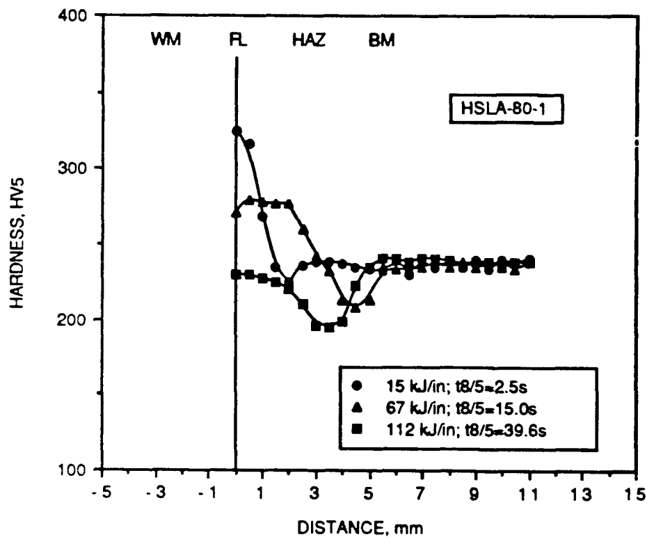
Fig.5.3. Typical microhardness distribution across HAZ from fusion line to the unaffected base metal for HSLA-80-1 at three different cooling times (800 to 500°C)
