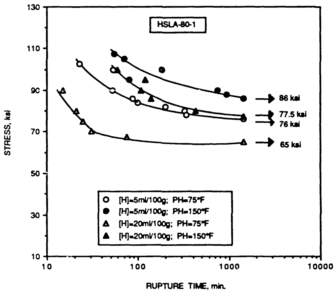
Fig.4.26. Implant cracking test results for HSLA-80-1
