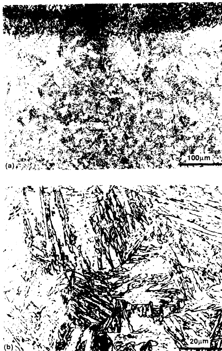
Fig. A-14. Microstructure of the fully martensitic coarse grained HAZ; (a) 200X, (b) 1000X.
