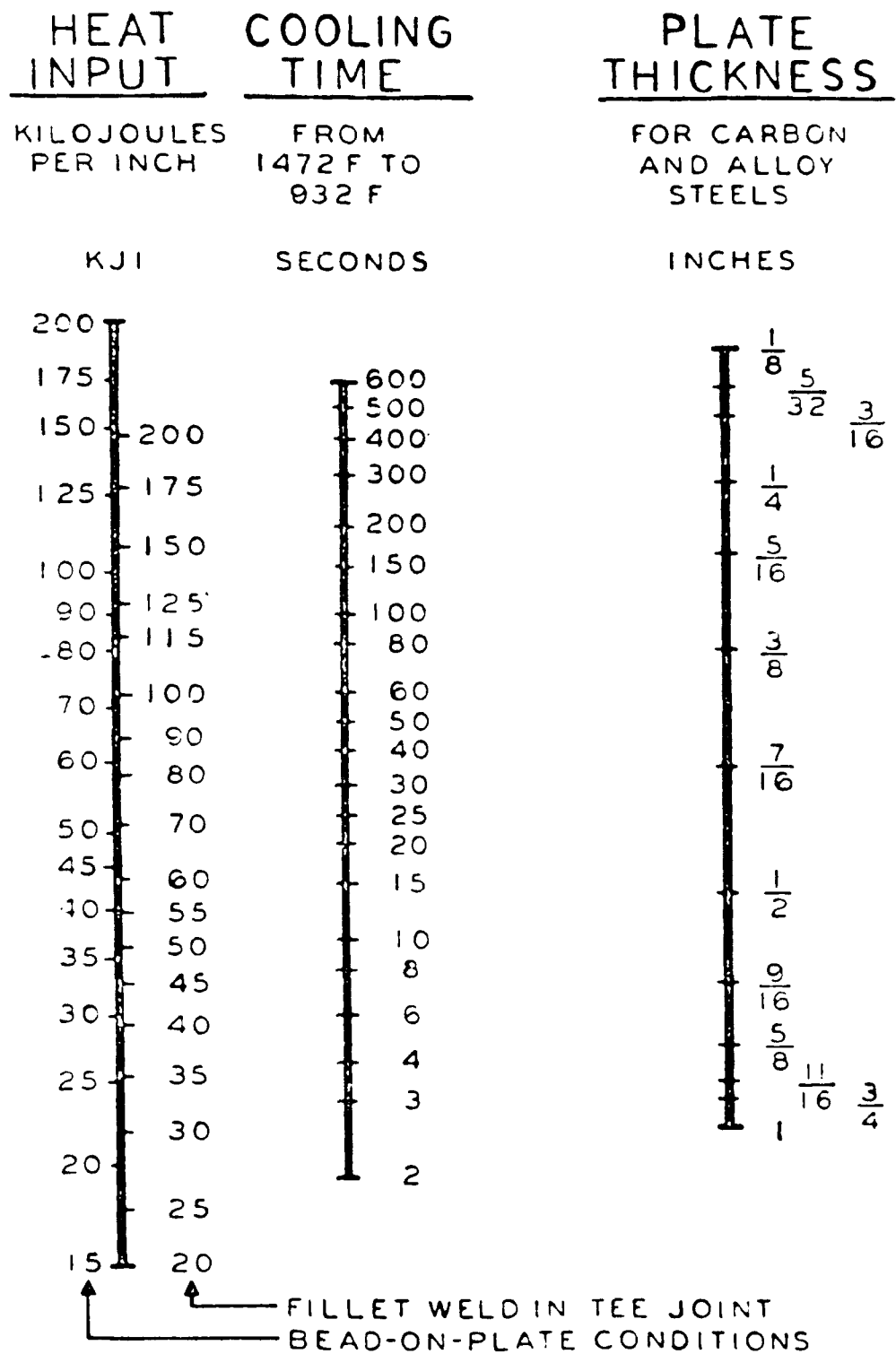
Fig.3.7. Nomograph for calculating cooling time which elapses between 1472 and 932 °F when the base metal heat-affected zone cools from an arc-welding operation. [39]
