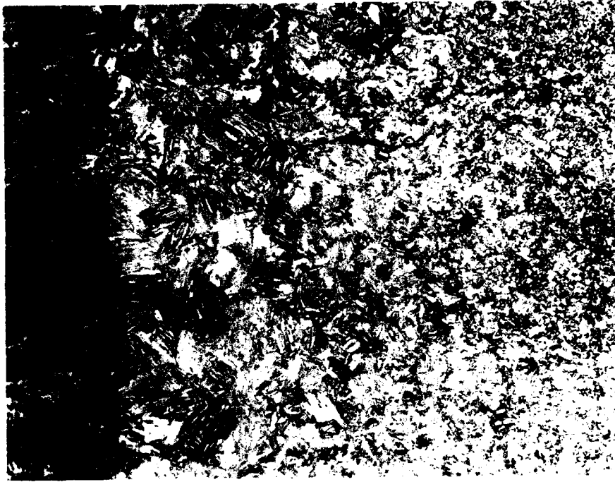
Fig.4.20. A typical weld metal/HAZ crack in the Battelle test. Steel HSLA-80-2; Preheat temp. 32°F; E6010 electrode; 200X
