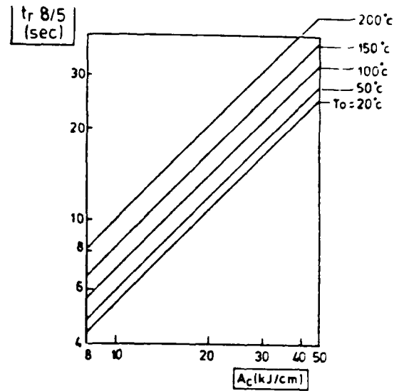
Fig.3.9(2). Charts for the determination of t_{8/5} . Three-dimensional heat-flow.
