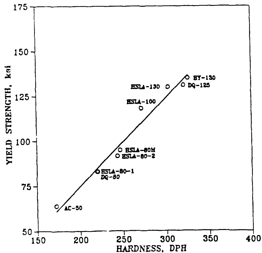
Fig. 2.2. Variation of yield strength with base metal hardness
