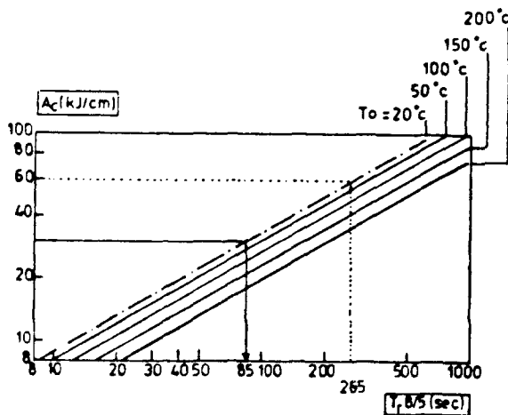
Fig.3.9(5). Charts for the determination of t_{8/5} . Two-dimensional heat-flow. Cooling time for d: 10 \text{ mm} .
