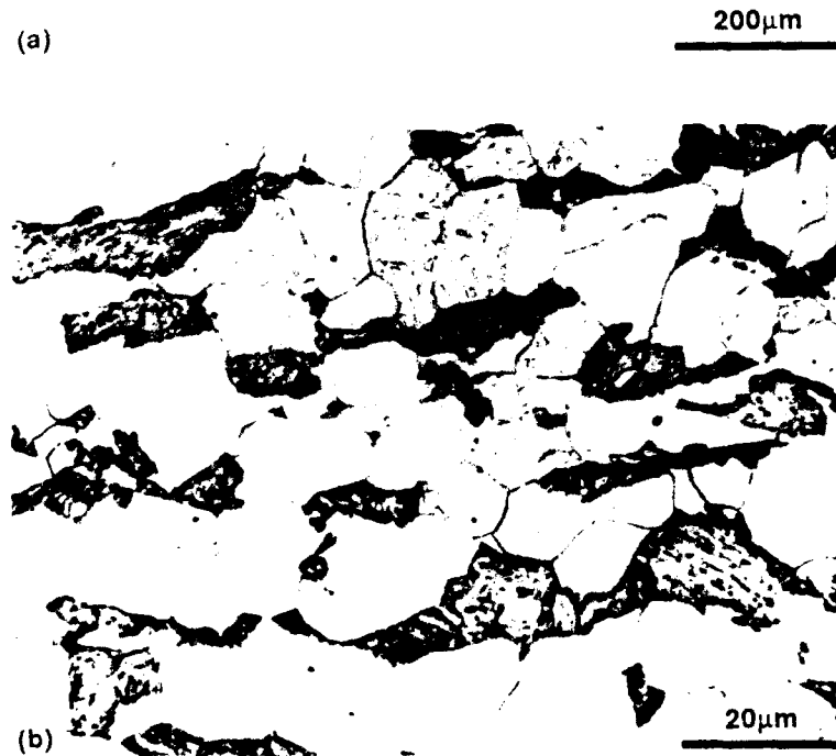
Fig. A-33.(a) Distribution of Inclusions, 100X, as-polished.
