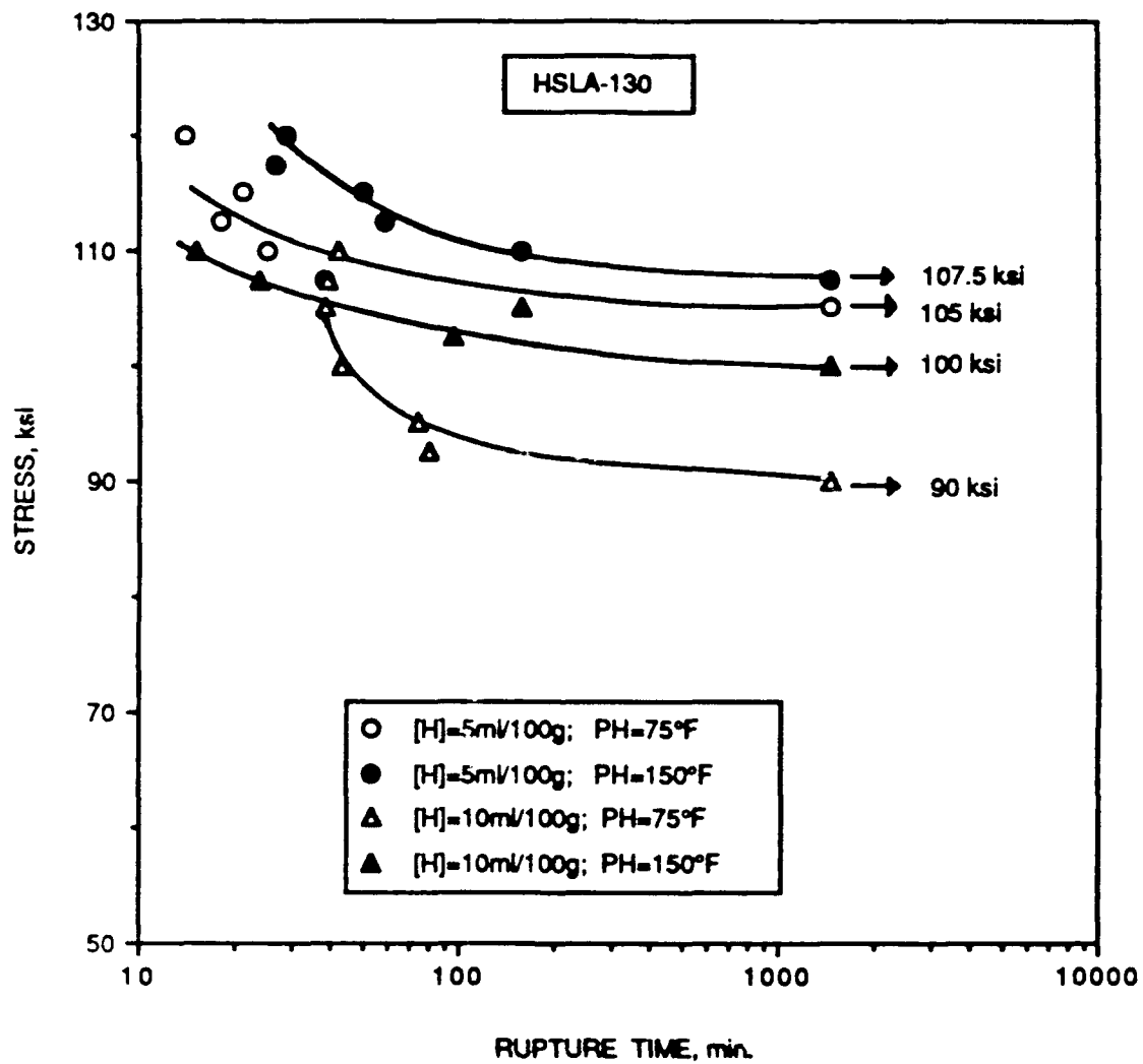
Fig.4.31. Implant cracking test results for HSLA-130
