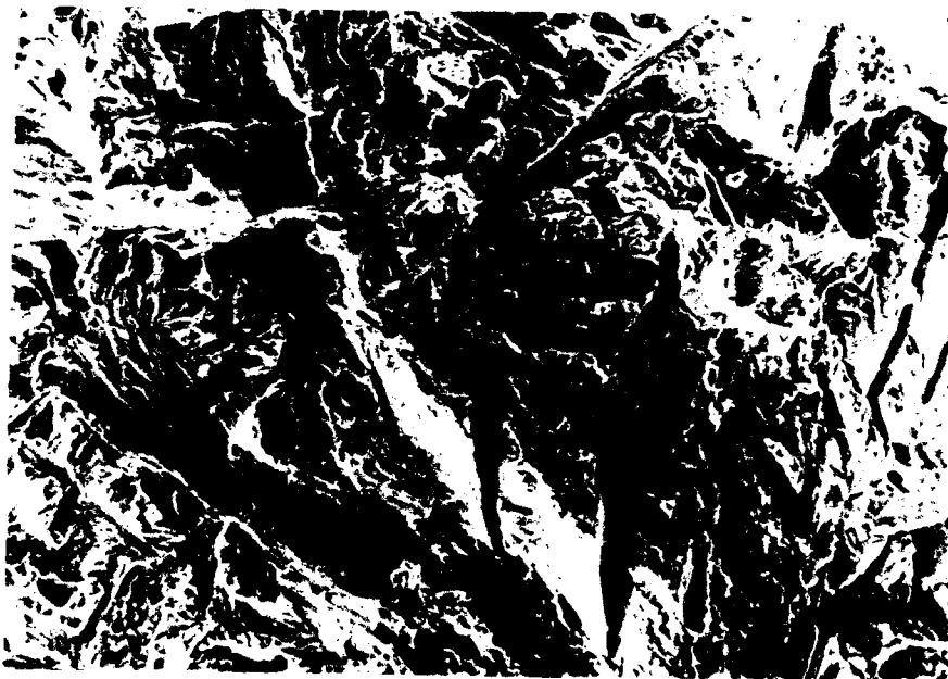
Fig. 4.45. Quasi-cleavage fracture mode with river patterns and tear ridges indicating the influence of martensite in HSLA-130; 500X
