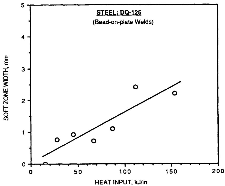
Fig. B-32. Variation of soft zone width with heat input for DQ-125
