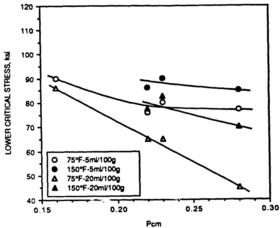
Fig.4.57. Variation of lower critical stress with P_{cm} for lower strength level steels
