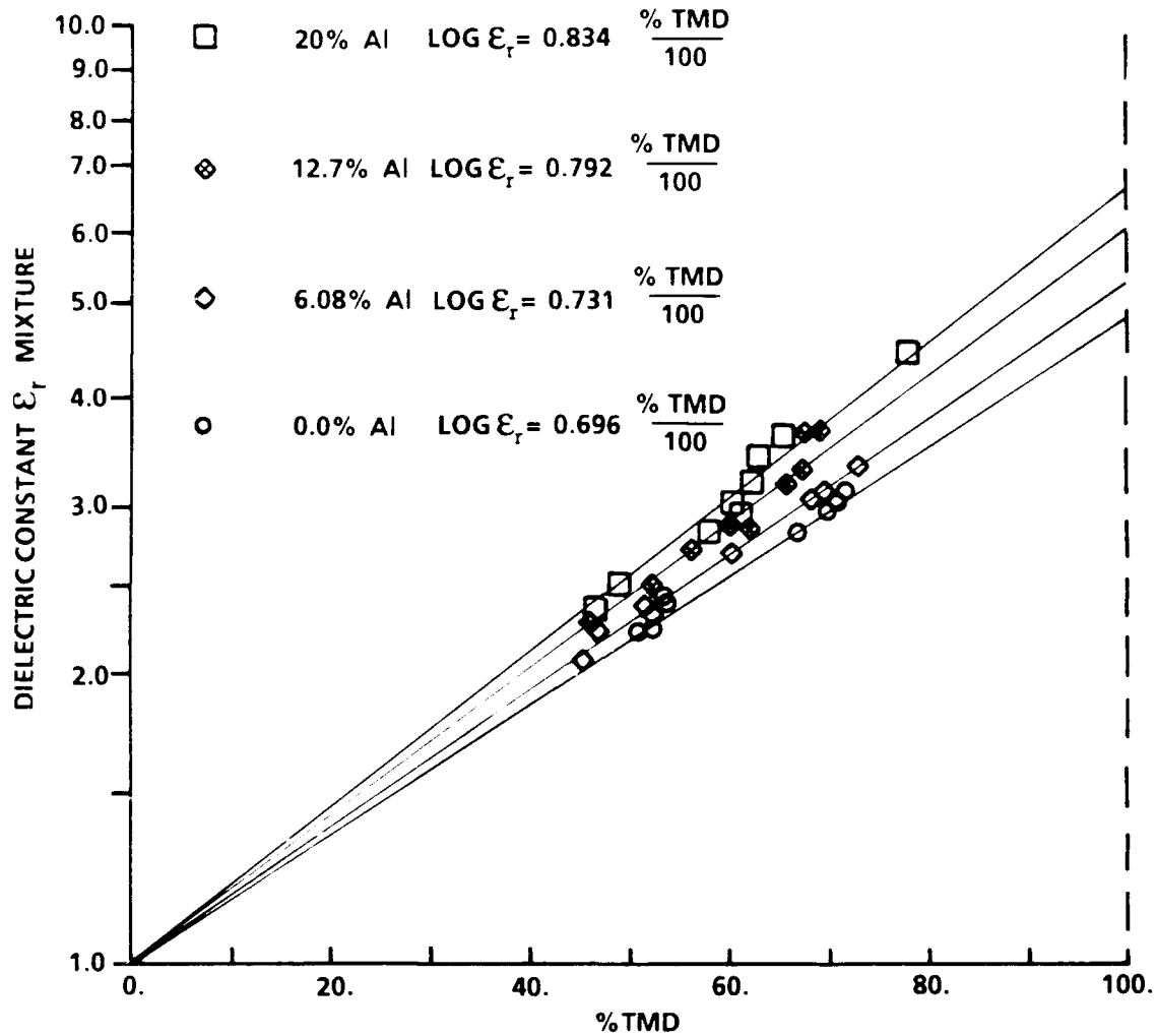
FIGURE 3-3. VARIATION OF DIELECTRIC CONSTANT WITH DENSITY FOR MIXTURES OF MELAMINE AND ALUMINUM AT 8.3 GHz
