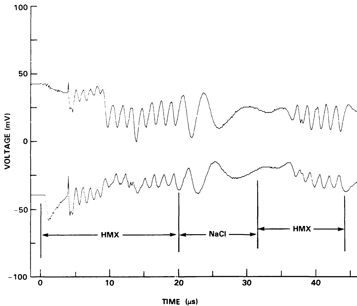
FIGURE 5-4. OUTPUT FRINGES FROM DETONATION TRANSFER TEST, M-7, USING COMPOSITE BED OF HMX/NaCl/HMX
