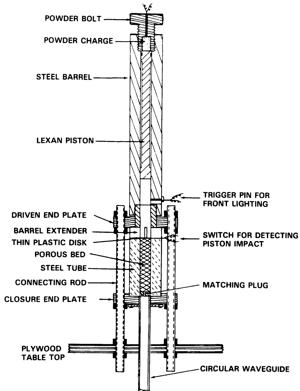
FIGURE 5-14. PDC APPARATUS INTERFACED WITH MICROWAVE INTERFEROMETER
