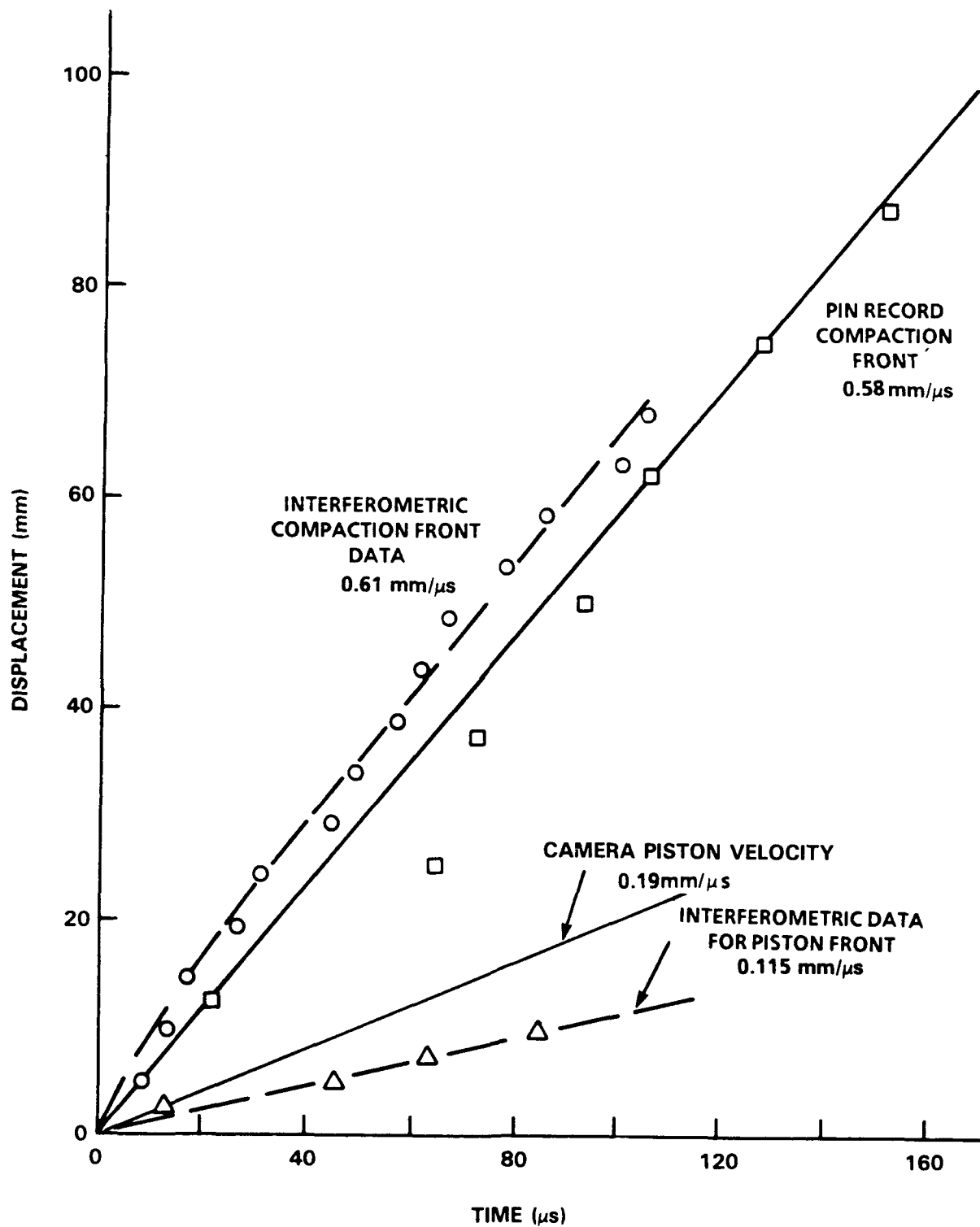
FIGURE 5-15. INITIAL REDUCTION OF SUPERIMPOSED DATA SHOWING DISAGREEMENT OF PISTON FRONT MOTION
