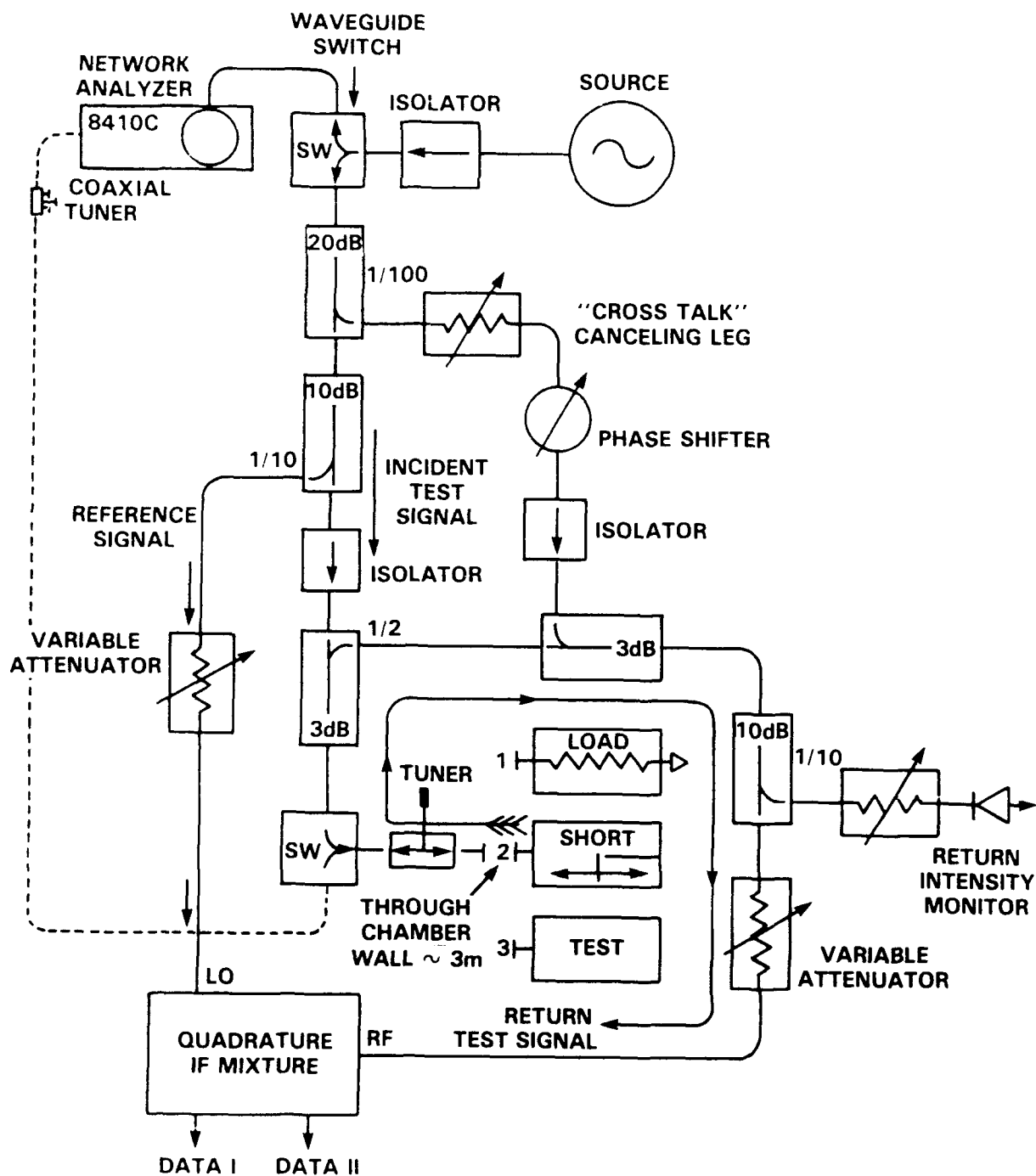
FIGURE 2-1 SCHEMATIC OF NSWC INTERFEROMETRIC CIRCUIT
