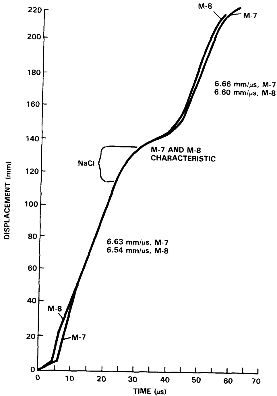
FIGURE 5-5. DISPLACEMENT-TIME HISTORY COMPARISON OF TWO HMX/NaCl/HMX DETONATION TRANSFER TESTS
