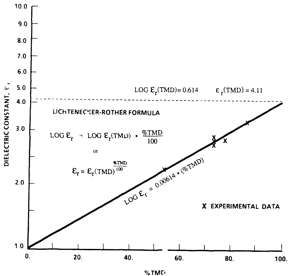
FIGURE 3.1. VARIATION OF DIELECTRIC CONSTANT WITH DENSITY FOR CLASS D HMX AT 8.3 GHz
