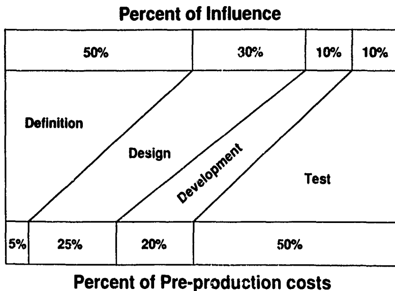
FIG. 4. SOFTWARE DEVELOPMENT
