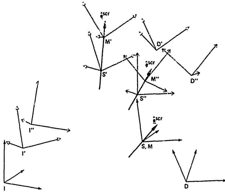
Figure 10. Screw constraint.
