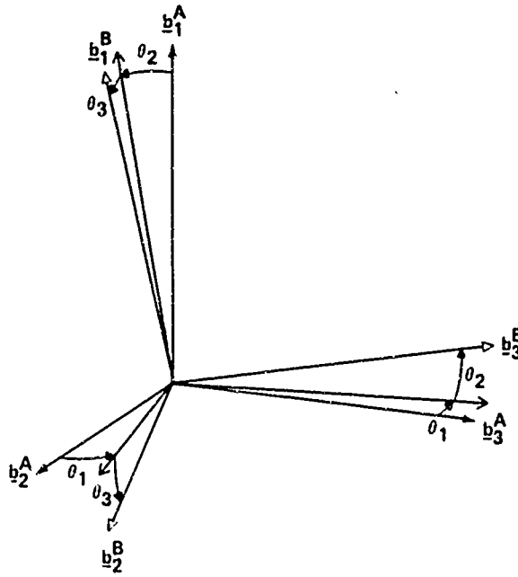
Figure 6. Tait-Bryan orientation angles (1-2-3).
