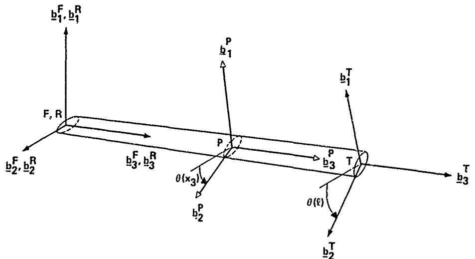
Figure 17. Aeroelastic beam element (undeformed with pretwist).
