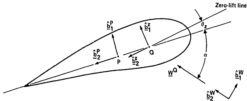
Figure 18. Aeroelastic beam cross section.
