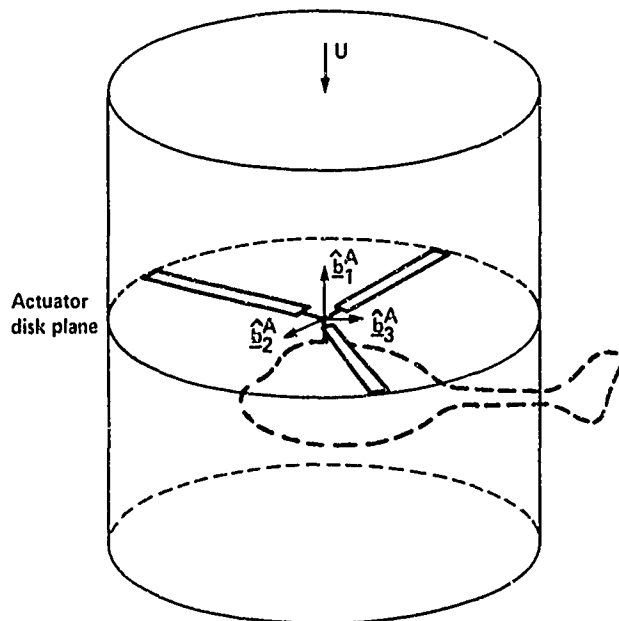
Figure 15. Air mass element flow field.
