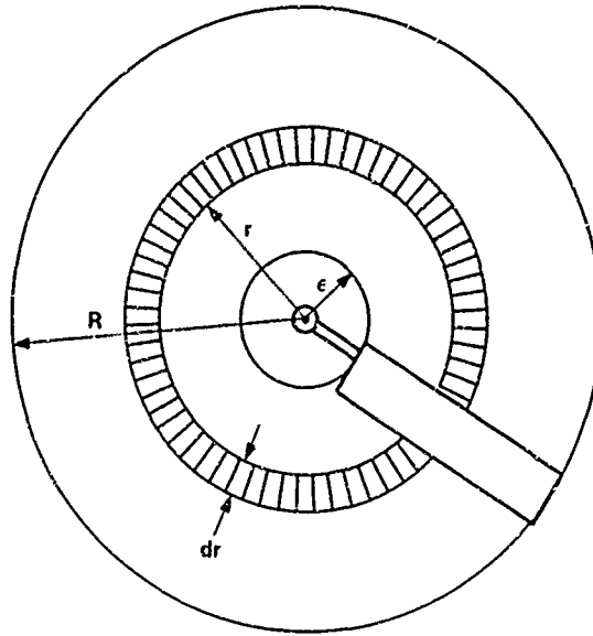
Figure 16. Air mass element differential annulus.
