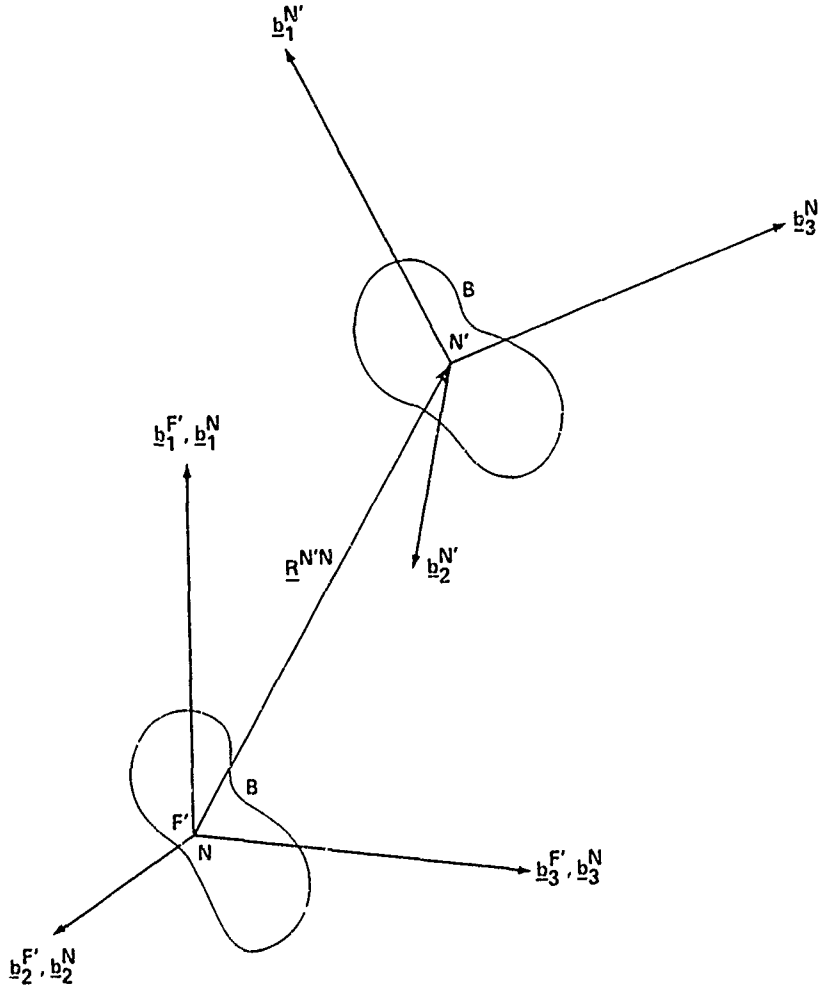
Figure 14. Rigid-body mass element.
